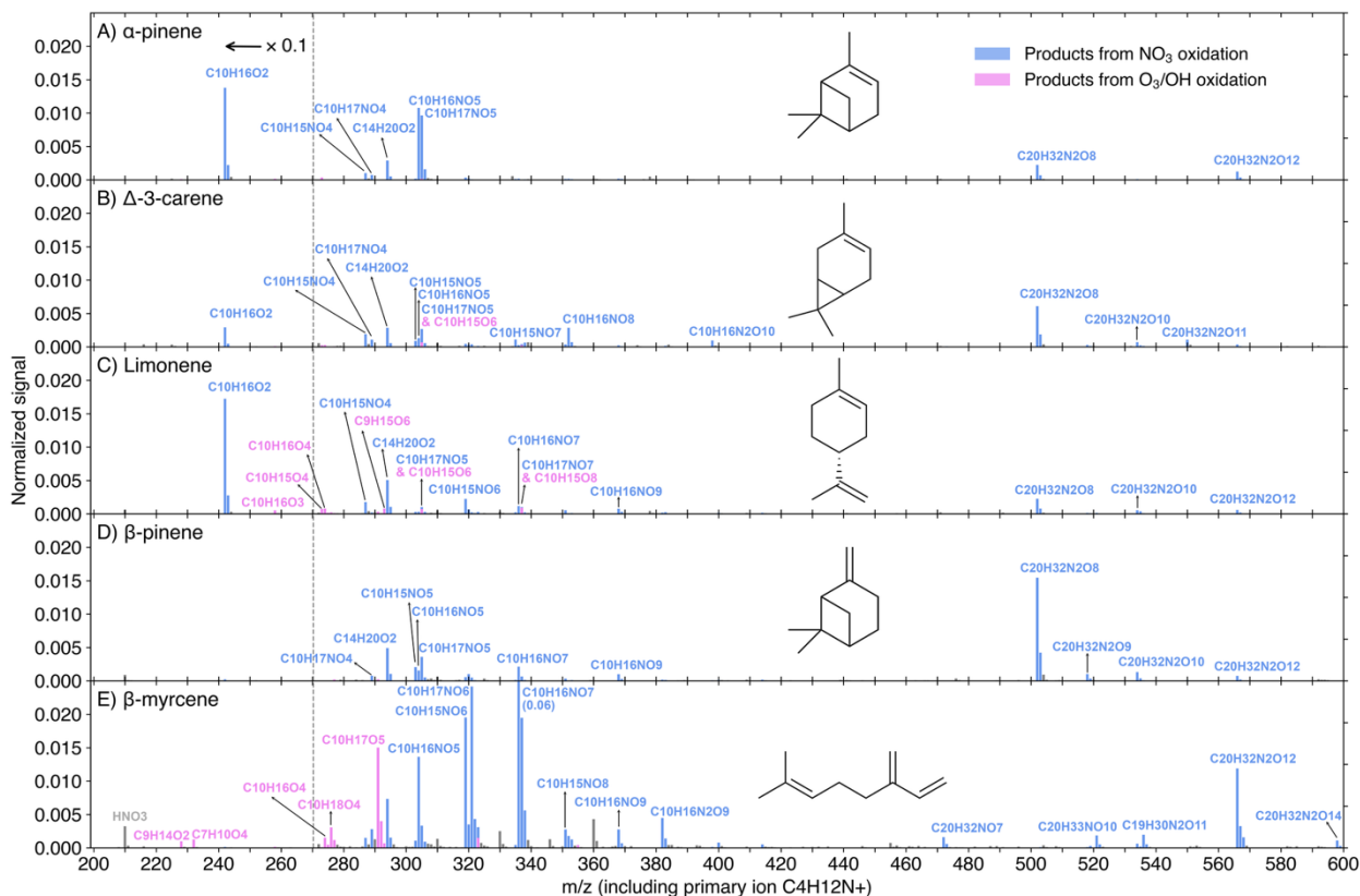
Figure 3. DEA-CIMS spectra (10 min average) of MT + NO_3 reactions at the experimental stage 6. Initial concentrations were [MT]_0 = 20 ppb, [O_3]_0 = 12 ppb, and [NO_2]_0 = 50 ppb, with an effective reaction time of 8.8 s. The spectra display the normalized peak signals (see Equation S4) and were corrected by subtracting background signals. Blue bars represent products (including both radicals and closed-shell species) from NO_3 oxidation, pink bars show products from O_3 or OH oxidation, and grey bars are for peaks not of interest. All compounds of interest were charged by clustering with the C_4H_{12}N^+ reagent ion, which is omitted from the displayed molecular formulas for clarity. Peaks smaller than 271 Th are divided by 10.
