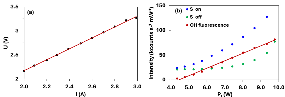
255 Figure 7: (a) Voltage–current relationship of the filament, (b) On-resonance signal intensity, S_{on} , background noise, S_{off} , and the OH fluorescence signal at elevated filament power. Where dots represent experimental data and solid lines represent linear fit results, the coefficients are 0.999 and 0.995 for (a) and (b).
