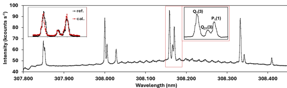
Figure 4: OH excitation spectrum obtained by scanning the laser from 307.800 nm to 308.450 nm in 0.001 nm steps. The inset with red frame shows the characteristic three peaks corresponding to the Q_1(3) , Q_{21}(3) , and P_1(1) rovibronic transitions. The upper-left inset shows the comparison results of the three characteristic peaks measured simultaneously by the reference (ref.) system and the ambient measurement system combined with a OH calibration (cal.) source.
