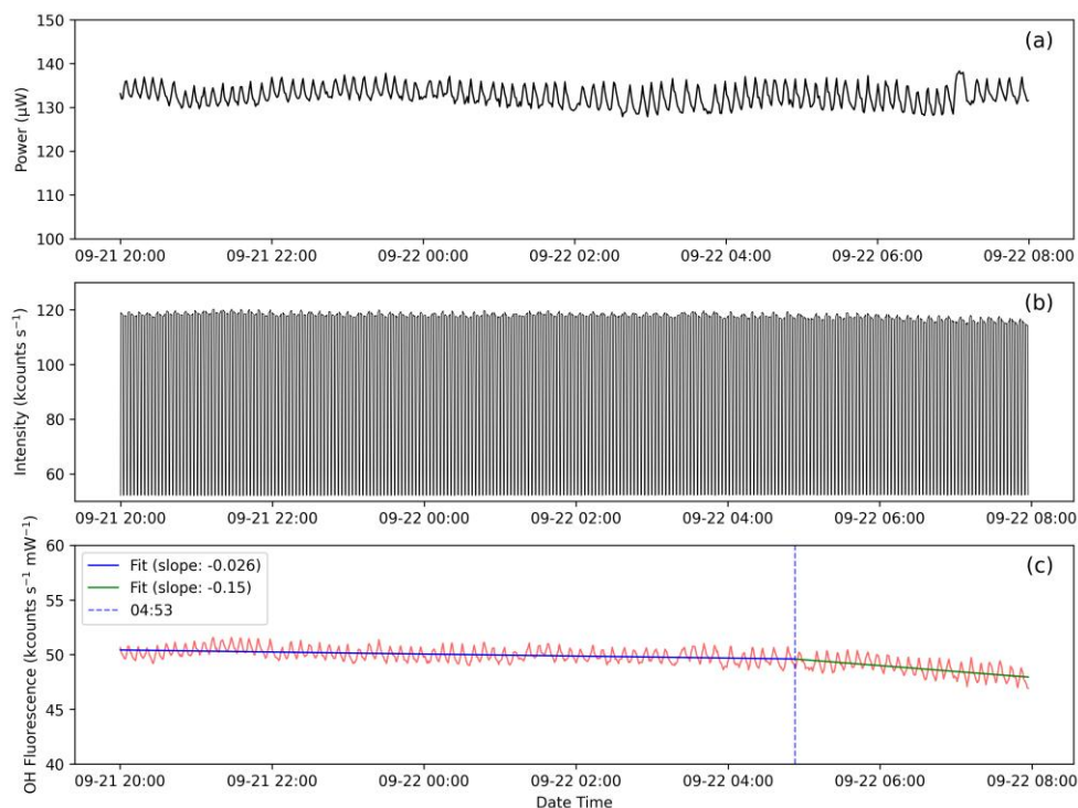
305 Figure 9: Long-term stability assessment of the reference system: (a) laser power in the reference cell, (b) signal intensities during alternating acquisition of background and on-resonance measurements, and (c) derived OH fluorescence signal, from 20:00 on September 21 to 08:00 on September 22. The short-term fluctuations observed in the signals are primarily attributed to the instability of the laser.
