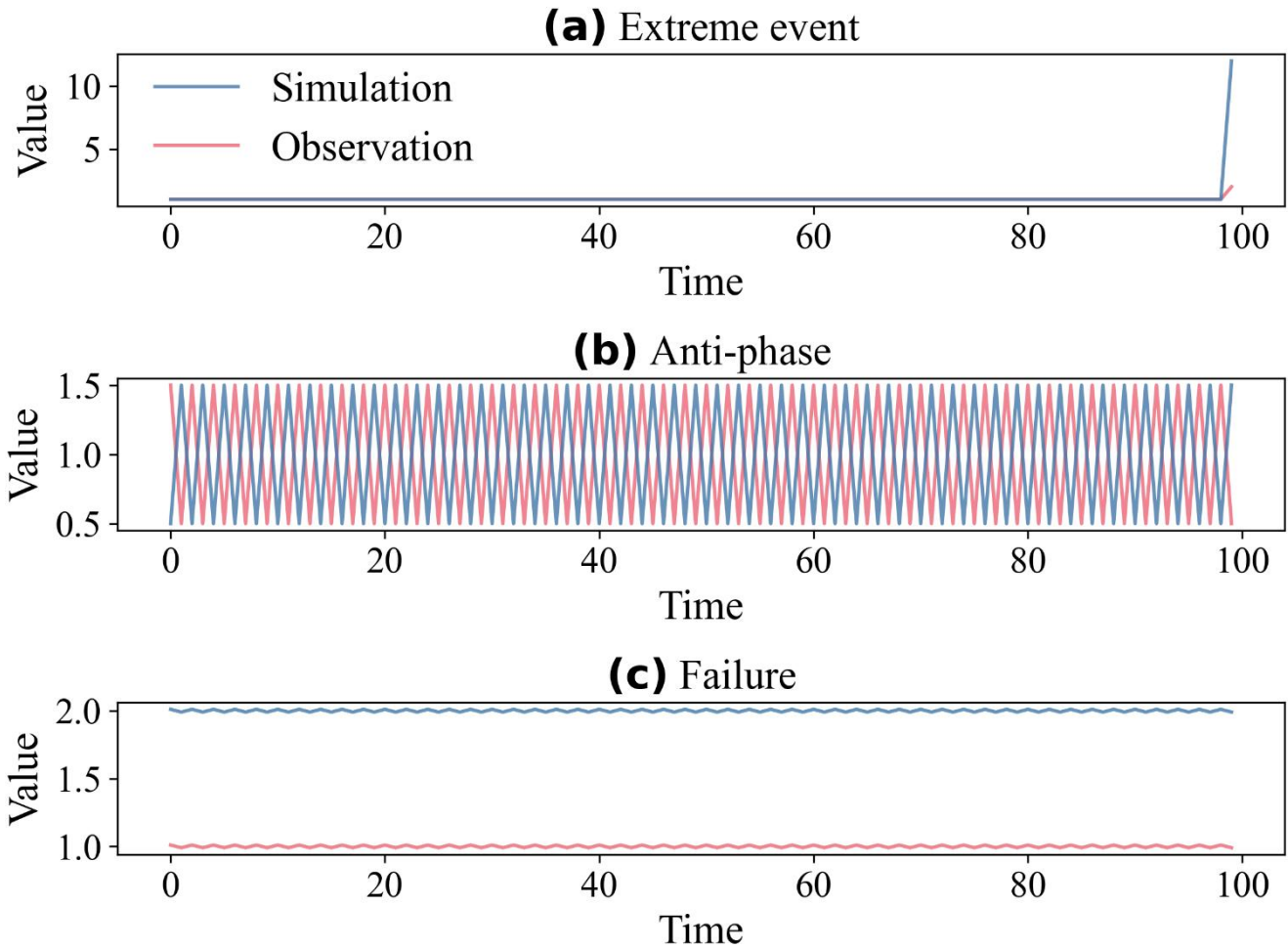
Figure 6. Phase and error decoupling test (all scenarios have RMSE = 1.0). (a) Extreme event. MFM (0.936) identifies high fidelity, while standard-baseline metrics fail (NSE = -100, KGE = -9.00, mKGE = -8.00, NRMSE = 0.990); (b) Reverse phase. All metrics identify failure, driven by r = -1.0 or PPF = 0.707 (MFM = 0.572, NSE = -3.0, KGE = -1.0, mKGE = -1.0, NRMSE = 1.0); (c) Simulation failure, driven by large bias/error (MFM = 0.316, NSE = -9999, KGE = 0.0, mKGE = -0.118, NRMSE = 1.0).
