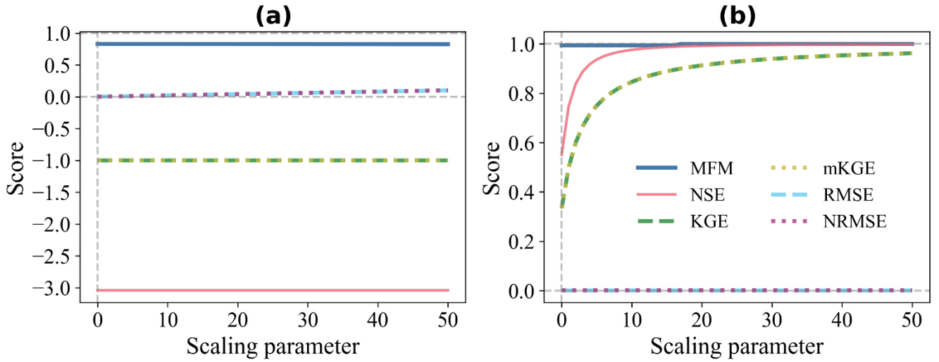
Figure 5. Sensitivity analysis under near-constant conditions. (a) Scenario A: Increasing error magnitude. MFM shows a slight decrease, while standard-baseline metrics remain insensitive at their failed values; (b) Scenario B: Constant error magnitude but increasing outlier size. Standard-Baseline metrics exhibit volatile increases attributable to changes in normalization factors, whereas MFM remains stable.
