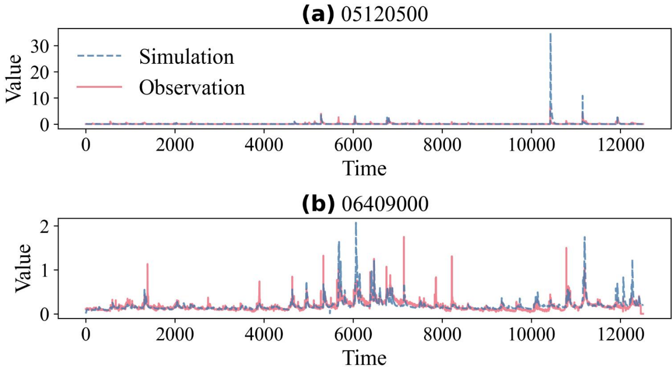
Figure 9. Time series examples from the CAMELS dataset. (a) Site 05120500. Near-constant data with an extreme event, highlighting the instability of standard-baseline metrics; (b) Site 06409000. Data with a small phase shift but low r , highlighting MFM's ability to decouple phase and magnitude errors.
