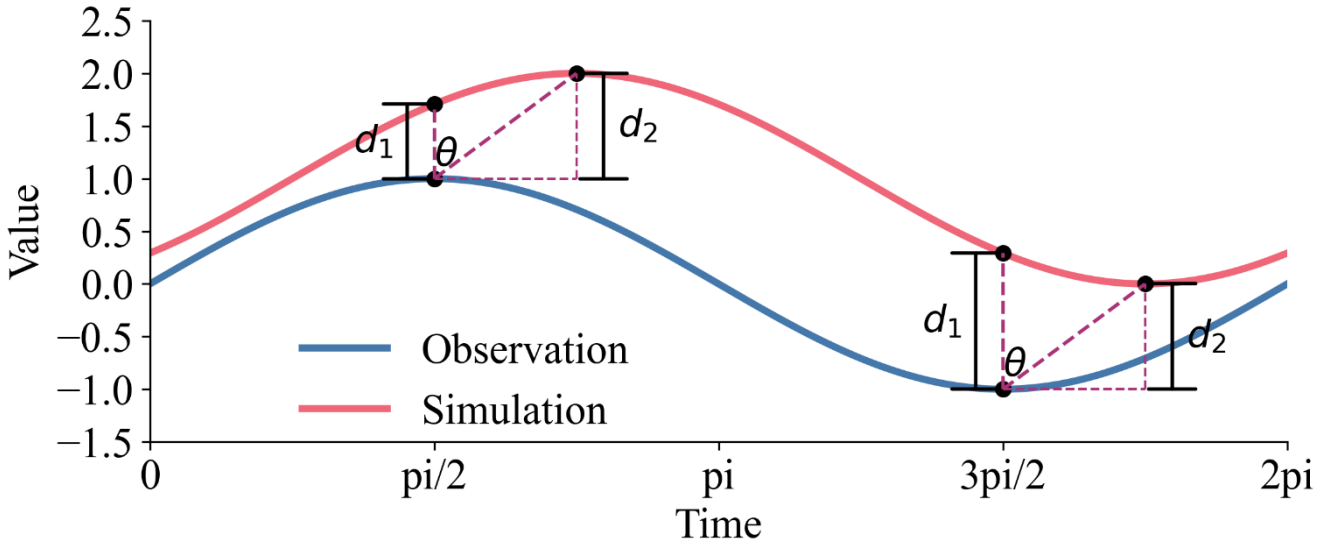
240 Figure 1. Geometric interpretation of the relationship between instantaneous error ( d_1 ), phase-corrected error ( d_2 ), and phase shift ( \theta ). This illustrates how phase differences inflate perceived magnitude errors, thereby justifying treating phase shift as a penalty factor (PPF) applied to the accuracy component.
