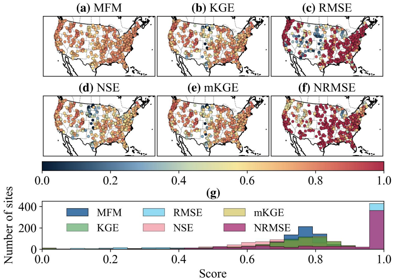
490 Figure 8. Spatial pattern and distribution of metrics across CAMELS dataset. (a) - (f) Spatial representation of MFM, KGE, RMSE, NSE, mKGE, and NRMSE; (g) Histogram of scores. MFM shows a more centralized distribution, reflecting its robustness. Standard-Baseline metrics exhibit long tails and extreme negative values.
