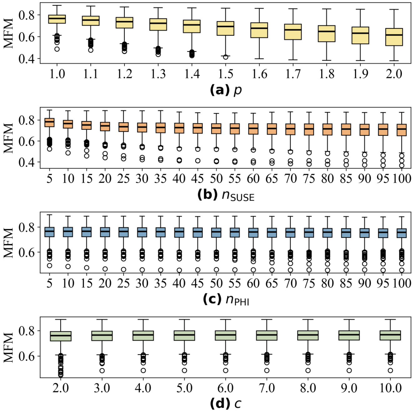
535 Figure 11. Sensitivity of MFM scores across the CAMELS dataset to its four hyperparameters. (a) Sensitivity to error exponent ( p ). MFM scores decrease as p increases, reflecting a higher penalty for large errors; (b) Sensitivity to bins for SUSE ( n_{\text{SUSE}} ). Scores are stable; (c) Sensitivity to bins for PHI ( n_{\text{PHI}} ). Scores are stable; (d) Sensitivity to phase penalty ( c ). MFM slightly increases as c increases.
