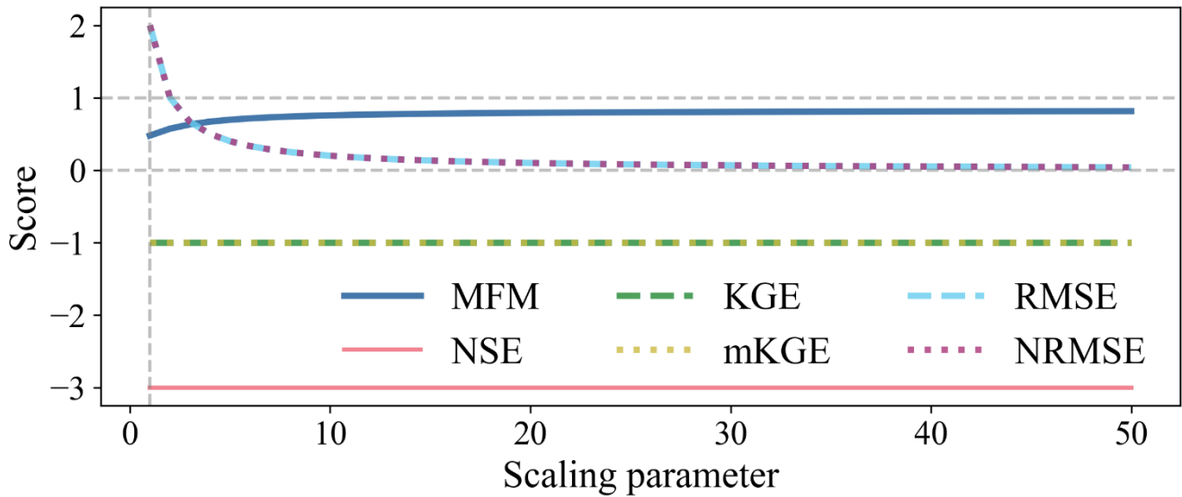
Figure 7. Sensitivity analysis of the reverse phase scenario with decreasing magnitude error. MFM correctly responds to the decreasing error, while standard-baseline metrics remain insensitive, overly penalized by the constant anti-correlation ( r = -1.0 ).
