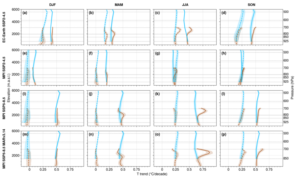
355 Figure 3: Alpine temperature trends near the surface (along the slopes) averaged over 200 m-elevation bins (T2m, brown) and in the free atmosphere averaged over the available pressure levels (Tp, blue). The historical period (1961-2014) is in dashed lines, projection (2015-2100) is in full lines. Shaded bands represent the spatial standard deviation (1 sigma). 360 The first three rows are based on the MAR v3.10 simulations and the last one on the MAR v3.14 experiment. Columns are for each season.
