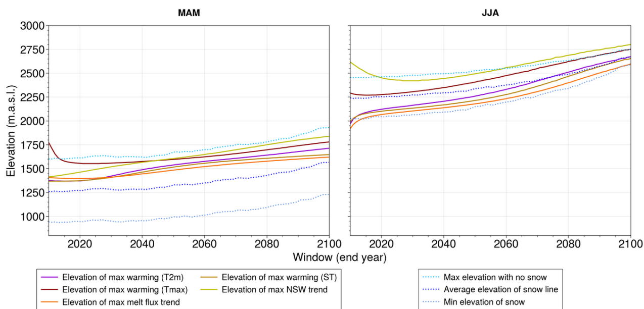
535 Figure 5: Elevation of snowline, maximum warming trends (T2m, Tmax, ST), melt flux trend and net shortwave trend in spring and summer over the course of rolling 50-year windows spanning 1961-2100 in the MAR v3.14 simulation over the Alps. The final year of each window is shown on the x axis.
