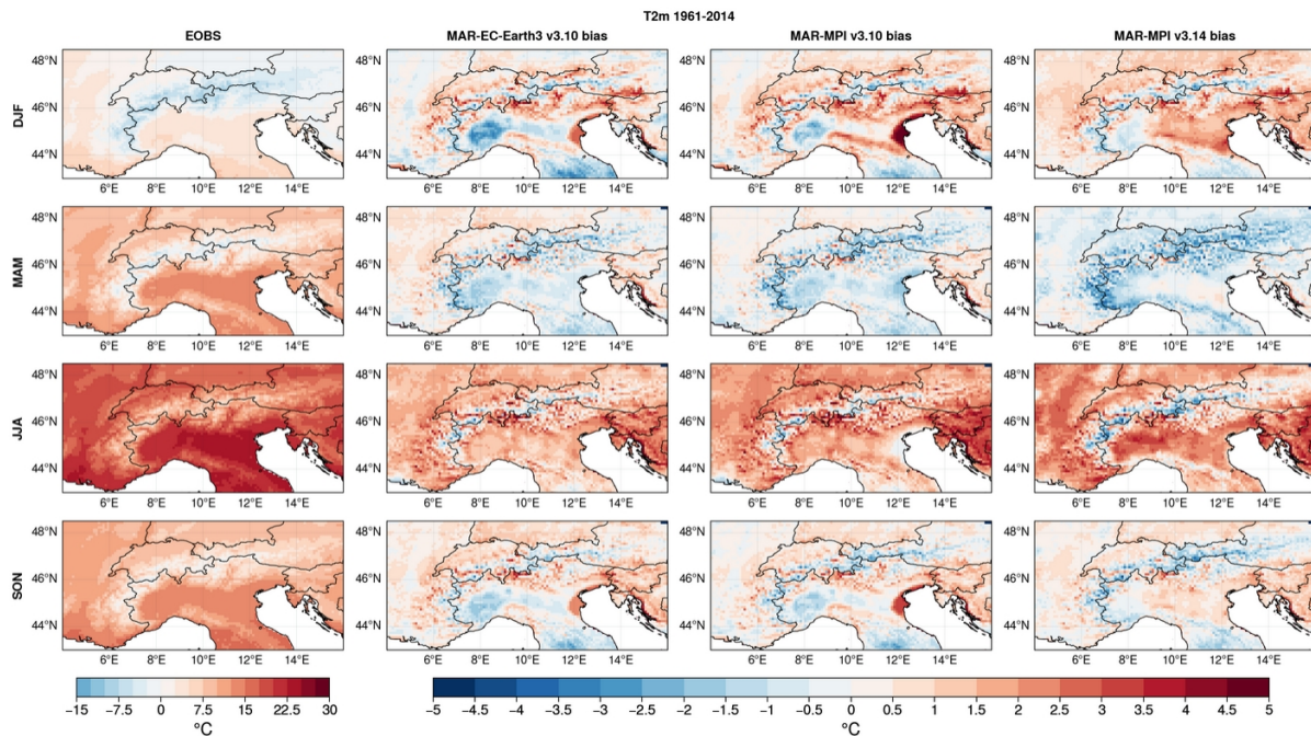
775 Figure C2: First column: Mean daily temperature at 2m (T2m) for each season averaged over 1961-2014 for E-OBS. Next three columns: Difference between MAR simulations (forced by EC-Earth3 and MPI-ESM1-2-HR using version 3.10 of MAR, and by MPI-ESM1-2-HR using version 3.14 of MAR for the 2nd, 3rd and 4th columns respectively) and E-OBS over the same period.
