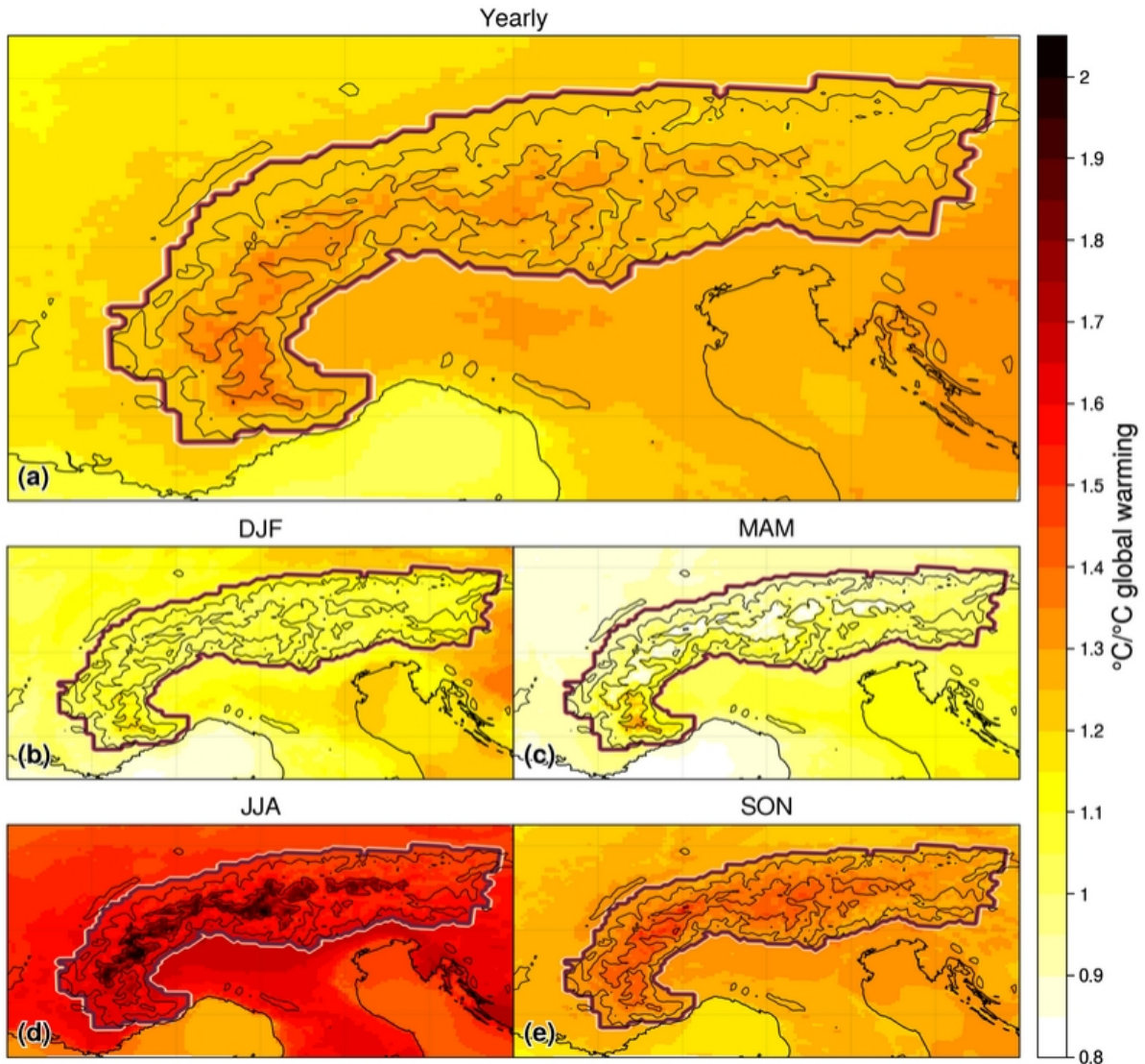
Figure 2: (a) Yearly warming over 1961-2100 in the three v3.10 simulations scaled with respect to global warming level in the forcing GCM. (b), (c), (d), (e): same as (a) at the seasonal timescale. 325 See Figure 1 for the definition of the contour line. Isolines every 1000 m are shown.
