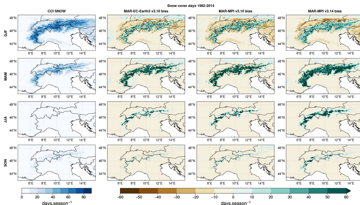
Figure C5: Same as Fig. C2 but for the number of days per season with snow on the ground, using SNOW-CCI. A grid point in MAR is considered to have snow if it has >50 mmWe of snow.
