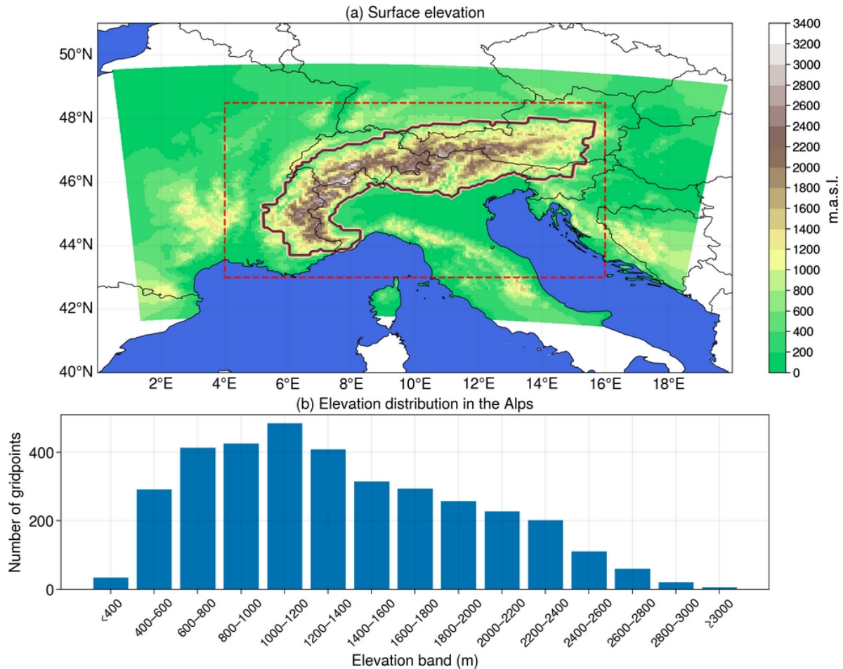
Figure 1: (a) Domain and orography of MAR simulations. The contour defines the Alps (see Sect. II.2.2) and is used as a mask further on in this paper (e.g. whenever there is a value averaged over the Alps). The red box is the area shown in Fig. 2, corresponding to the domain considered after excluding the lateral parts affected by boundary conditions in the MAR experiments. (b) Distribution of elevation inside the alpine contour discretized over 200m elevation bands. There are six gridpoints lying above 3000 m.a.s.l.
