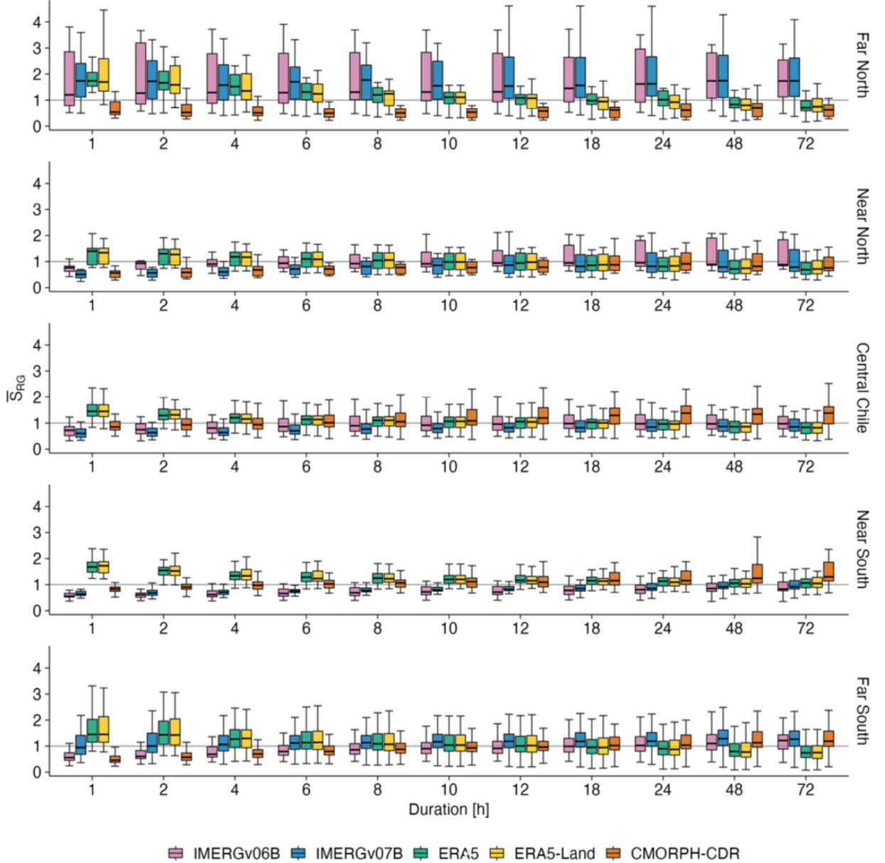
Figure 3. Boxplot of average annual bias-correction factors ( \bar{S}_{d, RG} ) for each gridded product per macroclimatic zone; for durations of 1, 2, 4, 6, 8, 10, 12, 18, 24, 48, and 72 hours.
