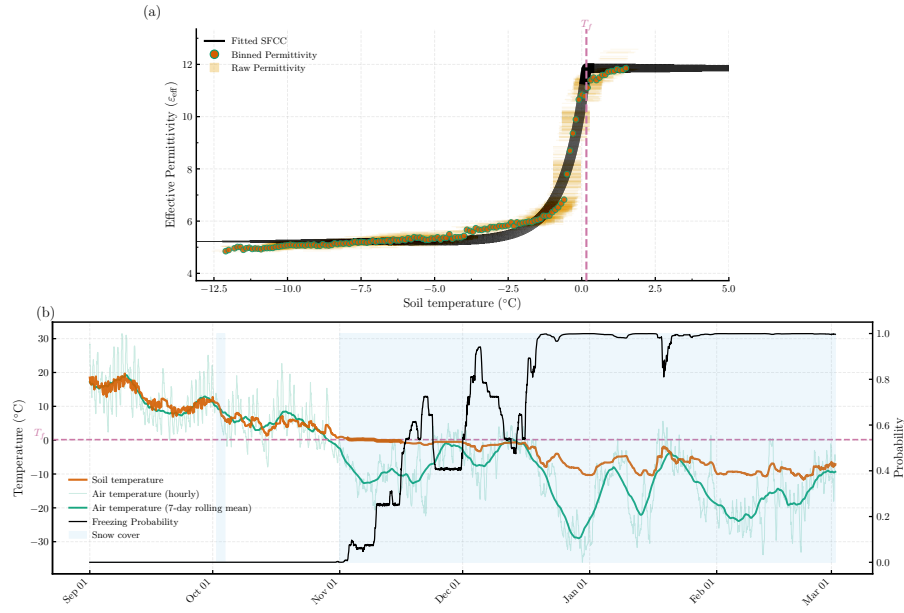
Figure 6. Fitted SFCC (a) and corresponding time series of soil temperature, air temperature, snow cover, and freezing probability (b) for the EC17 site in the Kenaston network (prairie). The site location is available via the interactive map on GitHub: Soil-Temperature-Permittivity-Monitoring-Sites.
