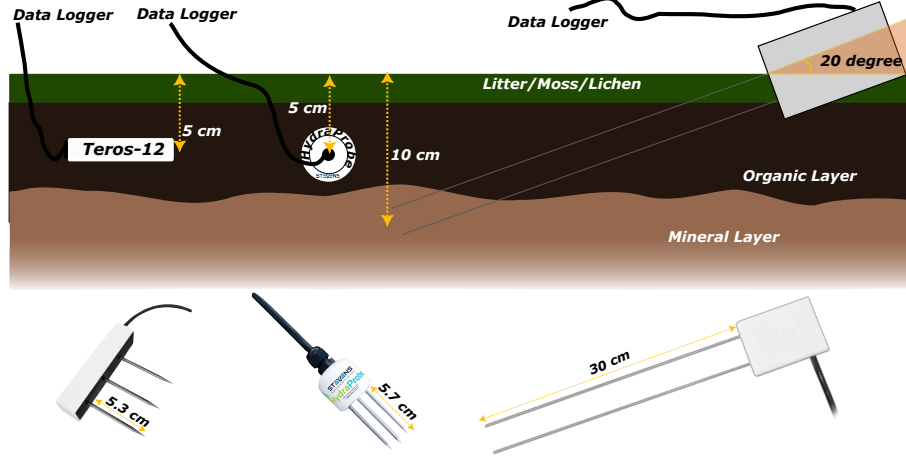
Figure A1. Instrumentation setup for soil moisture probes (CS616, HydraProbe, and TEROS12), with a schematic and corresponding probe images.
