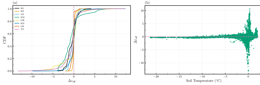
Figure 4. CDFs of residuals across networks (a), showing most residuals are small with steep slopes near zero, indicating minimal bias. Residuals as a function of soil temperature (b), with random subsampling of an equal number of samples per network for balanced representation.
