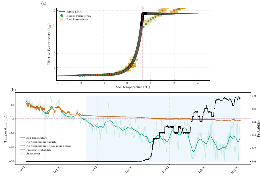
Figure 8. Similar to Fig. 6, but for the BJ01 site in the Baie-James network (eastern boreal forest).
