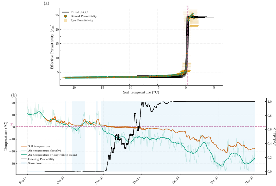
Figure 9. Similar to Fig. 6, but for the GR01 site in the George River network (tundra).
