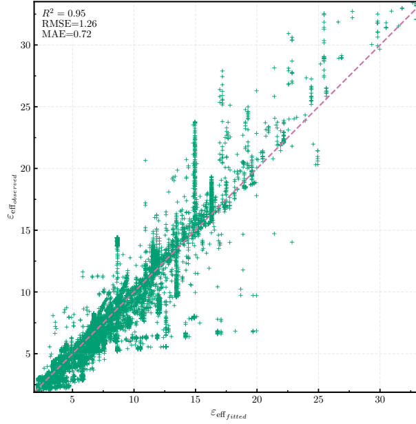
Figure 3. Comparison of \varepsilon_{\text{eff,observed}} and \varepsilon_{\text{eff,fitted}} for freezing cycles.
