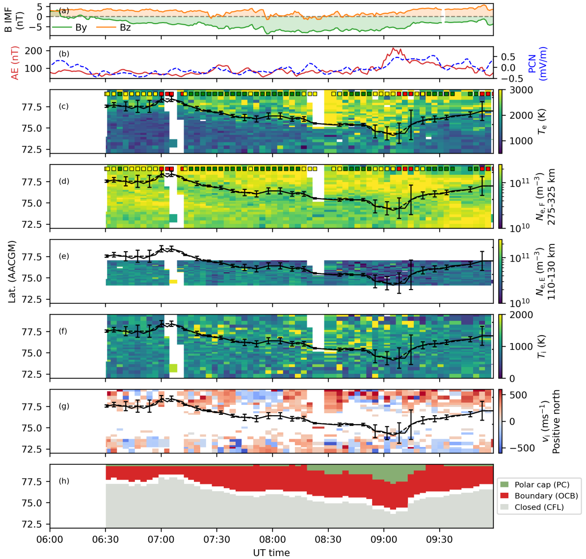
Figure 2. Overview of observed T_e , T_i and N_e , and identified regions on open and closed field lines by the ESR 32 meter from December 4 2014. Panel a shows the IMF B_z and B_y components, panel b the AE (red solid, left hand axis) and PCN (blue dashed, right hand axis) indices, panels c-g show T_e , N_{e,F} (high F-region (275-325 km), N_{e,E} (E-region, 110-130 km), T_i , and v_i observed at 300 km altitude by the 32 meter along the geographic meridian. The solid black line indicates the open-closed field line boundary. The colored squares show the quality flags. Panel h shows colored regions of the 32-meter data corresponding to closed field lines (grey), in the polar cap (green) and along the open-closed field line boundary (red).
