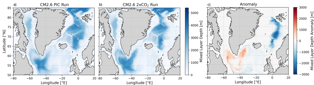
Figure C2. We show 20-year mean March mixed layer depth (MLD) from the (a) preindustrial control (PIC) simulation as well as (b) the 2 \times CO_2 experiment. (c) shows the anomaly in March MLD, computed as the difference between the 2 \times CO_2 and PIC simulations. MLD and the respective anomalies are shown in meters (m).
