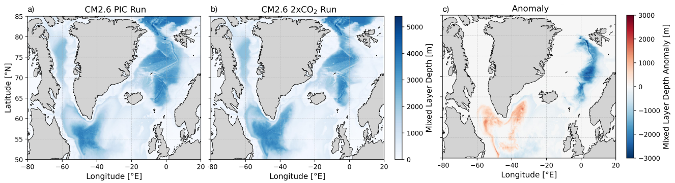
Figure C2. We show 20-year mean March mixed layer depth (MLD) from the (a) preindustrial control (PIC) simulation as well as (b) the 2\times CO_2 experiment. (c) shows the anomaly in March MLD, computed as the difference between the 2\times CO_2 and PIC simulations. MLD and the respective anomalies are shown in meters (m).
