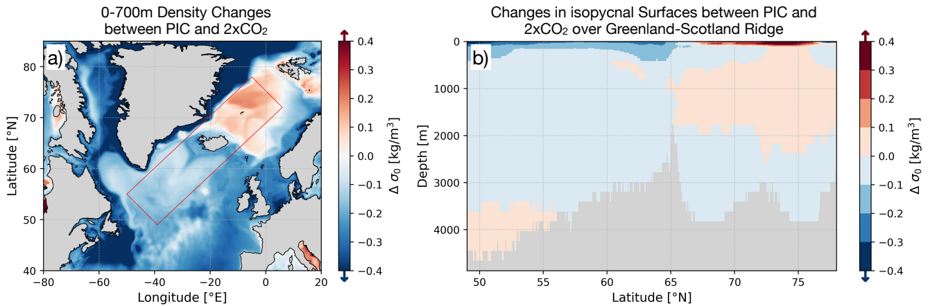
Figure 5. Density changes under elevated atmospheric CO_2 concentration averaged over 20 model years. a) is depicting density changes in the upper 700 m between the CM2.6 PIC run and the 2 \times CO_2 scenario. b) is showing the latitude-depth cross section of the red box in a) .
