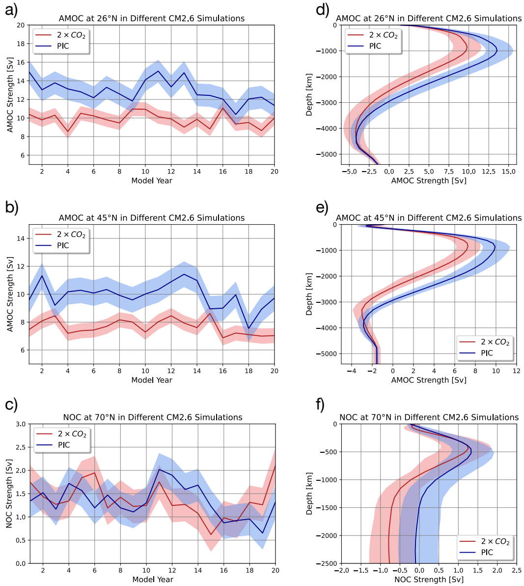
Figure C1. We show the AMOC at 26°N and 45°N, together with Nordic Seas overturning (NOC) estimates at 70°N. Panels (a–c) display annual mean time series for the last 20 years of the CM2.6 pre-industrial control (PIC) and 2 \times CO_2 simulations, while panels (d–f) show the corresponding overturning estimates at different depth levels (shading represents \pm 1 standard deviation).
