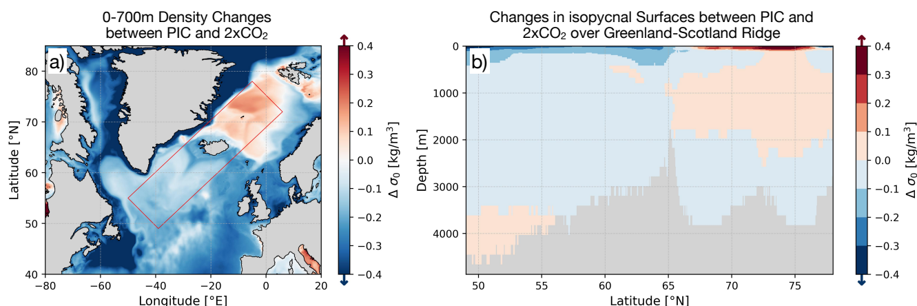
Figure 5. Density changes under elevated atmospheric e\Theta_2\text{-}CO_2 concentration averaged over 20 model years. a) is depicting density changes in the upper 700 m between the CM2.6 PIC run and the 2 \times e\Theta_2\text{-}2 \times CO_2 scenario. b) is showing the latitude-depth cross section of the red box in a) .
