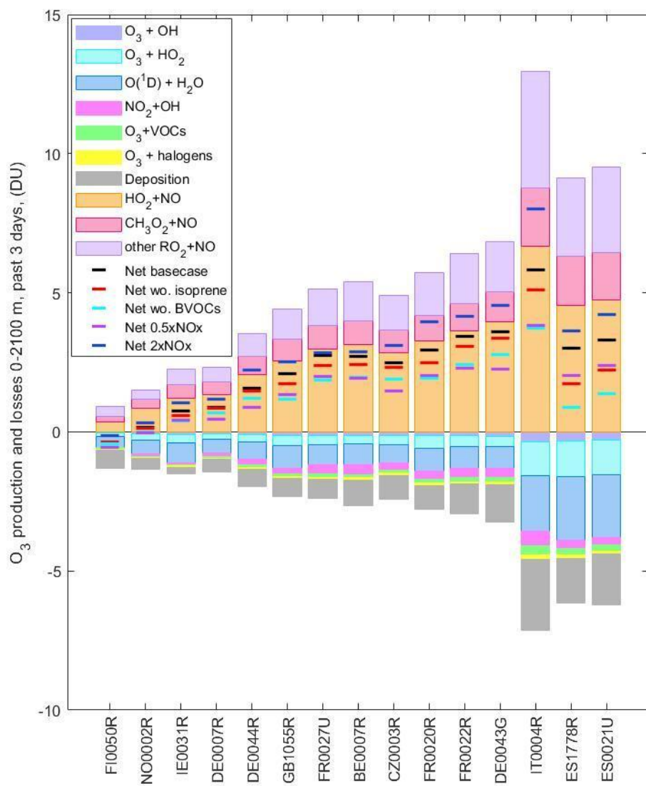
655 Fig. 27. Modelled (ADCHEM) 8-day averaged cumulative time-integrated O 3 production and losses in the lowest 2,100 m of the atmosphere for the past 3 days upwind of 15 targeted measurement stations. Ozone is lost by reactions with OH, HO 2 , unsaturated VOCs and various halogen (Br, I, Cl) radicals, when O( 1 D) reacts with H 2 O and when NO 2 reacts with OH. Ozone is produced when HO 2 , CH 3 O 2 and other RO 2 radicals react with NO. Also shown by horizontal lines are the net ozone formation (production minus losses) from the basecase simulations (Net basecase), for simulations without terrestrial biogenic emissions of isoprene (Net wo. isoprene), without any terrestrial BVOC
