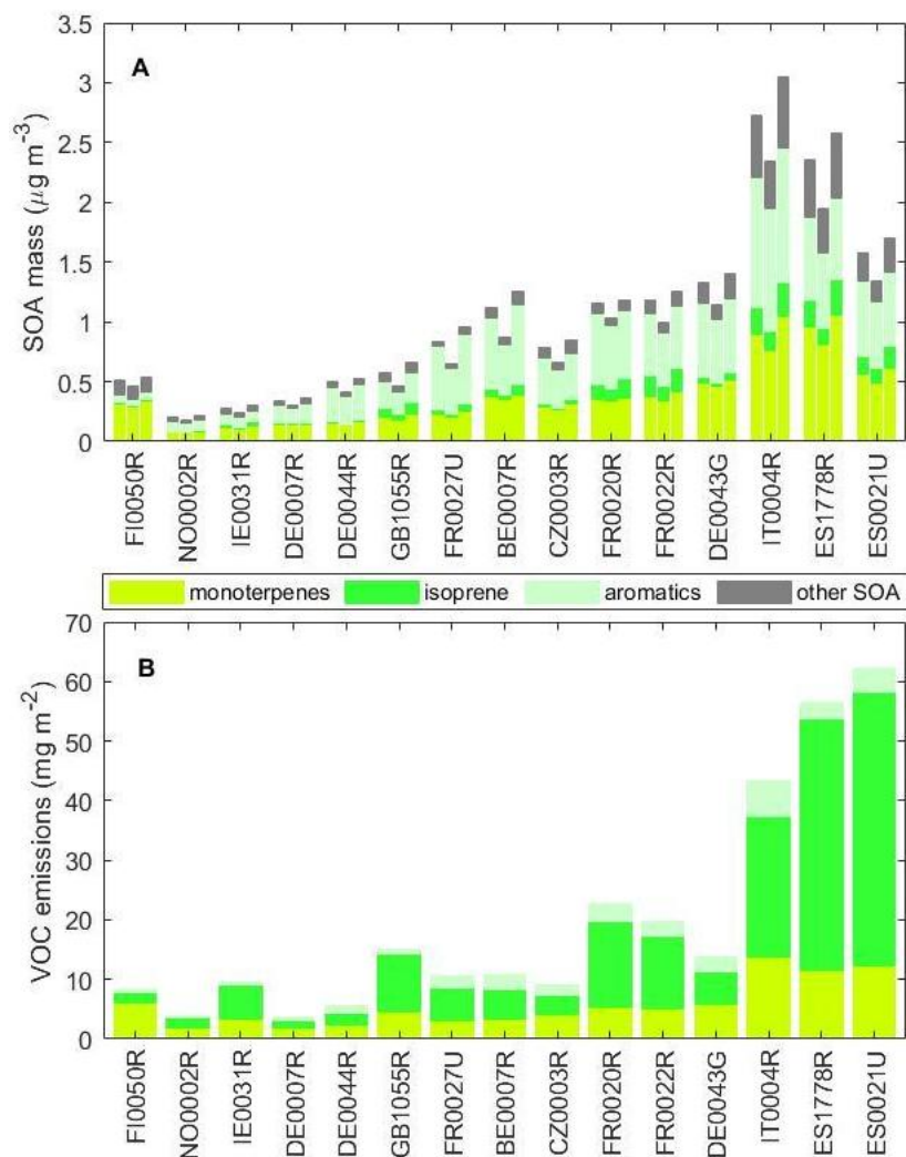
855 Fig. 153. Modelled averaged surface SOA mass concentrations (A) and 10-day cumulative SOA precursor emissions along the simulated air mass trajectories (B). In panel A, the three bars for each site represent the modelled average SOA mass for the basecase (left), 2xNO x (middle) and 0.5xNO x (right) simulations.
