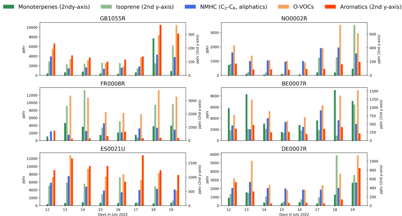
Fig. 76. Temporal variations of selected VOCs and VOC groups at 6 sites across Europe on 12-19 July.
