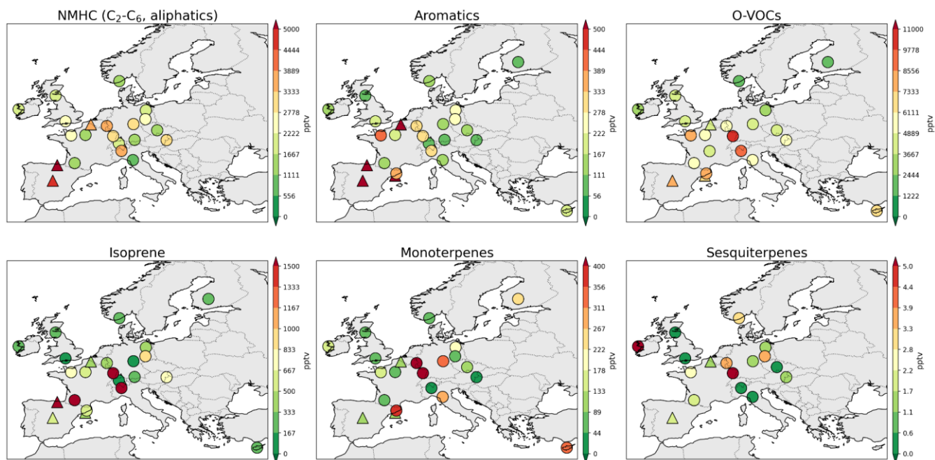
480 Fig. 5.4. Spatial variation of the average concentrations of the different VOCs from 12-19 July. The groups sum the average concentration for all the relevant components. The urban sites are marked as triangles.
