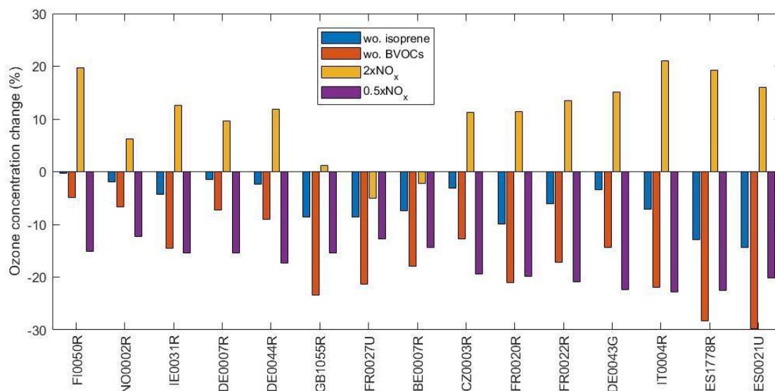
Fig. 108. Modelled 8-day averaged surface ozone concentration changes relative to the basecase simulations for 4 different model 665 sensitivity tests: without biogenic terrestrial isoprene emissions (wo. isoprene), without terrestrial BVOC emissions (wo. BVOCs), with 2 times higher anthropogenic NO x emissions (2xNO x ) and with 50 % lower anthropogenic NO x emissions (0.5xNO x ).
