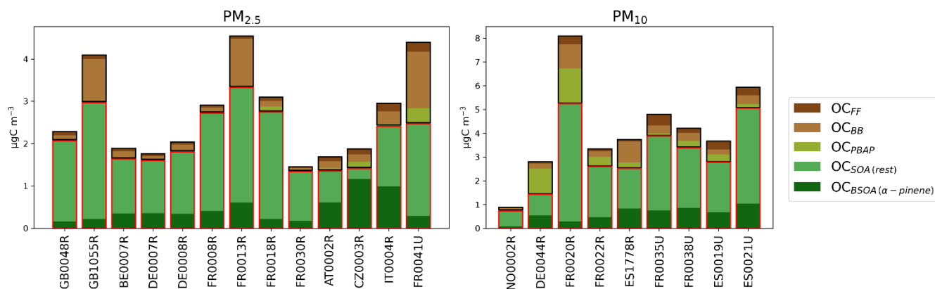
Fig. 120. OC apportioned into categories with PM_{2.5} (left) and PM_{10} (right) size fractions. Secondary OCs are indicated with a red border and primary OCs with a black border.
