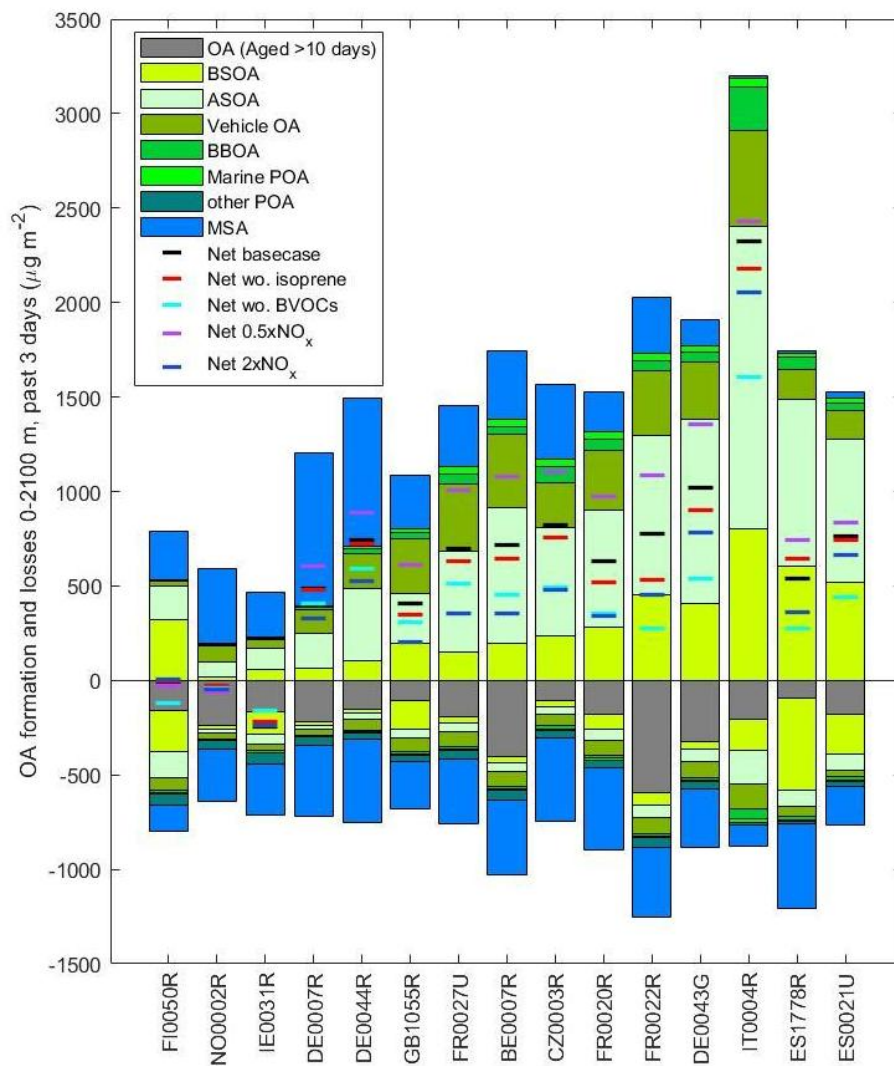
840 Fig. 134. Modelled (ADCHEM) 8-day averaged cumulative OA formation and losses during the past 3 days upwind of the measurement stations. OA formation includes primary emissions (POA) and secondary formation (SOA), while losses comprise dry/wet deposition and evaporation. OA is divided into source categories: aged background OA (>10 days), BSOA, ASOA, vehicle OA, biomass burning OA (BBOA), marine POA, other POA, and methyl sulfonic acid (MSA). Net OA formation (production minus losses) is shown for the base case and sensitivity simulations without isoprene, without all BVOCs, and with anthropogenic \text{NO}_x scaled by 0.5 \times and 2 \times .
