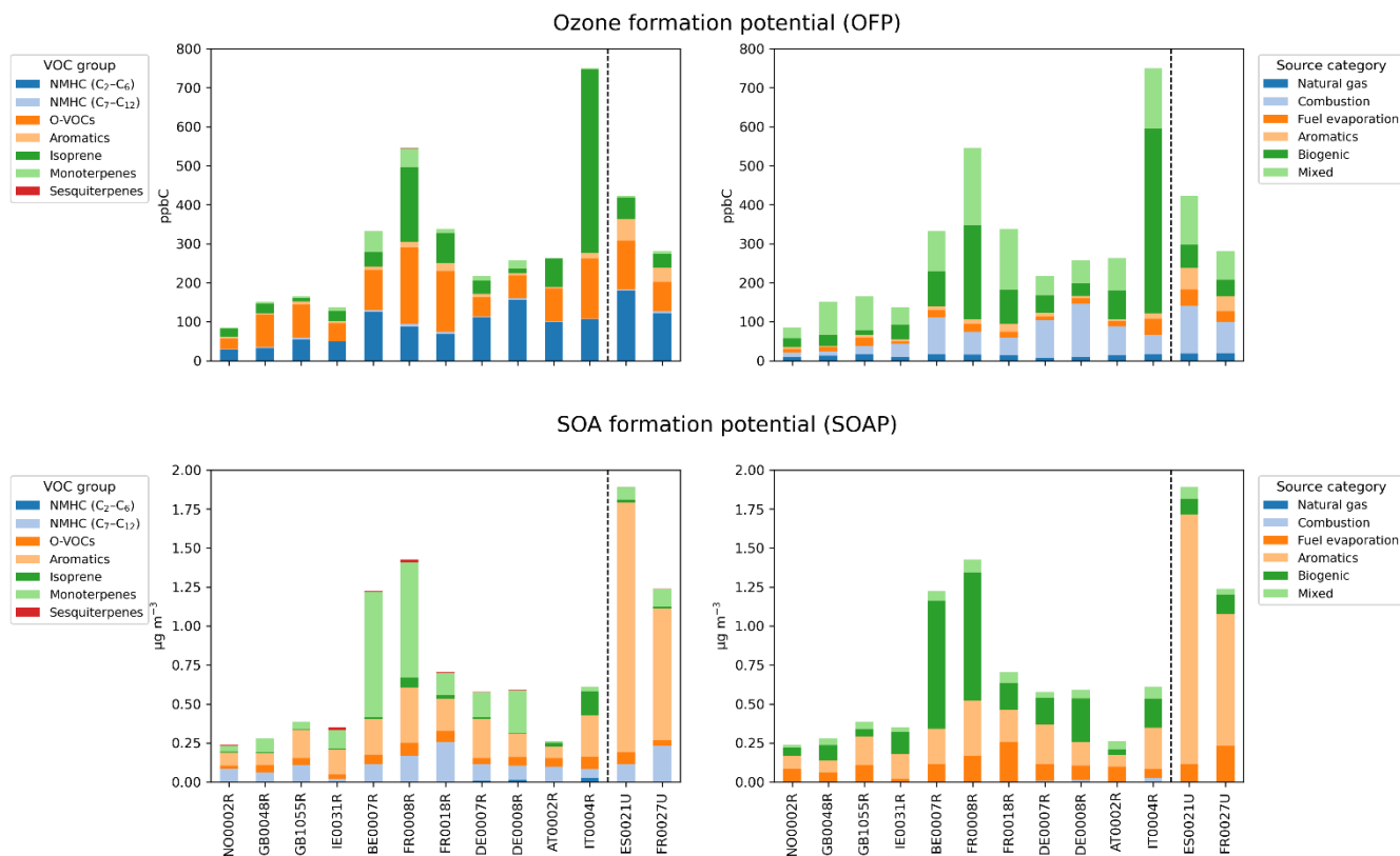
600 Fig 8. The ozone and SOA formation potentials related to 1) the sum of VOCs in the different component groups (left figures), averaged over 12-16 UTC, 12-19 July 2022 and 2) to the main emission source categories, the VOCs. Natural gas includes propane and ethane. Fuel evaporation covers branched/normal alkanes in the gasoline/distillate range (C 4 -C 12 ). Combustion includes unsaturated light hydrocarbons (butenes, pentenes, hexenes, 1,3-butadiene), acetylene, and propene. Aromatics are grouped together (toluene, xylenes, ethylbenzene, trimethylbenzenes, styrene, benzene) since they come from combustion, solvent use, and fuel evaporation. Biogenic includes isoprene mono- and sesquiterpenes Mixed is used for O-VOCs because they're largely secondary with multiple precursors/sources. 605
