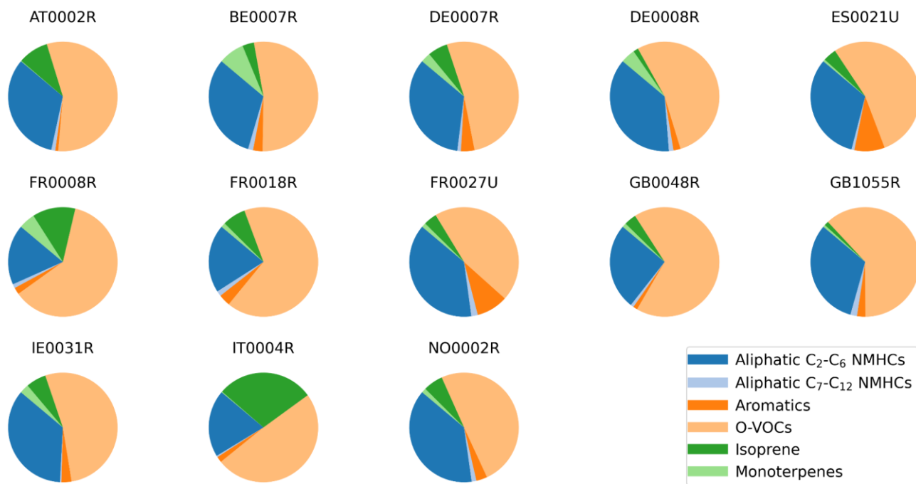
Fig. 32. Distribution of different VOC groups at sites where the most relevant component groups were measured. The figure is based on the relative contribution of the sum of the average concentrations (pptv), 12-19 July.
