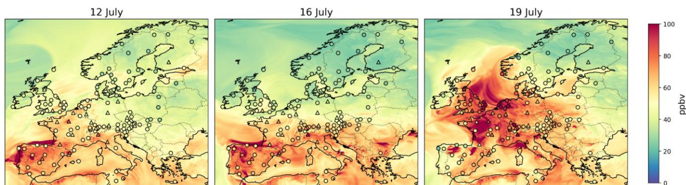
395 Fig. 24. 1-hour maximum ozone concentrations (ppb v ) based on the EMEP model and observations superimposed for the 12, 16 and 19 July 2022. The sites participating in the campaign are marked as triangles and regular EMEP sites as circles.
