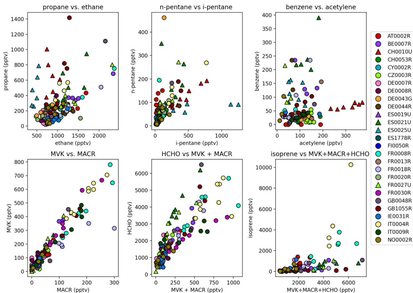
Fig. 65. Ratio of selected VOCs for daily-averaged concentrations. Urban sites are marked as triangles. Note that VOC concentrations at ES0025U are divided by five.
