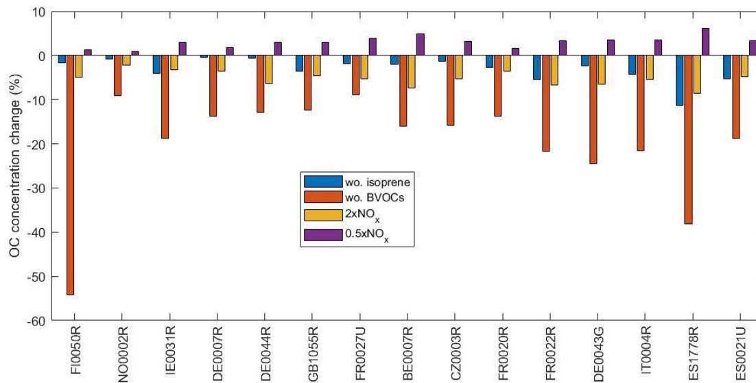
Fig. 142. Modelled 8-day averaged surface OC concentration changes relative to the basecase simulations for 4 different model sensitivity tests: without biogenic terrestrial isoprene emissions (wo. isoprene), without terrestrial BVOC emissions (wo. BVOCs), with twice the anthropogenic NO x emissions (2xNO x ) and half the anthropogenic NO x emissions (0.5xNO x ).
