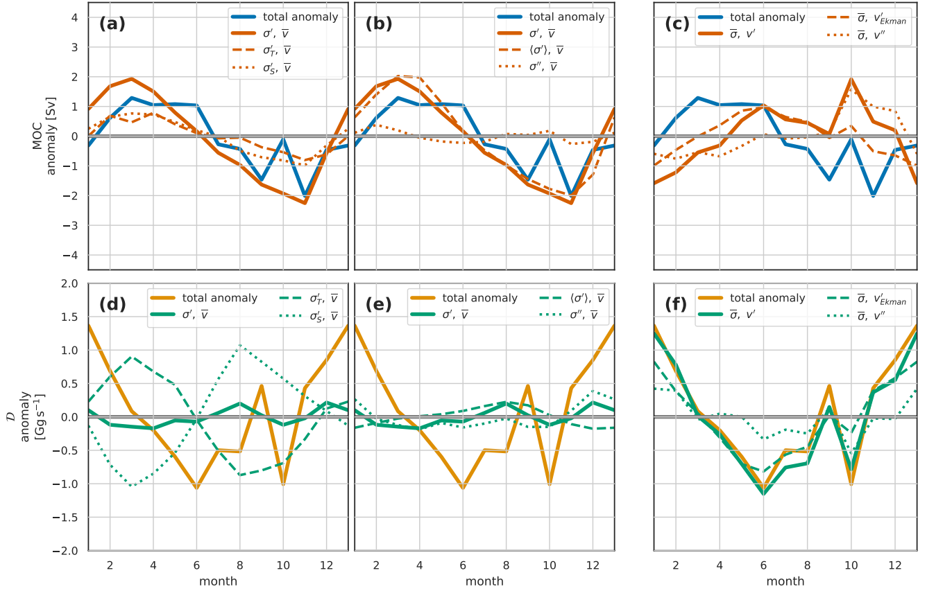
Figure 9. Summary plot of the decomposition of the seasonal cycle for the full OSNAP section of (a-c) \text{MOC}_\sigma and (d-f) density flux \mathcal{D} for the Viking20x model. The left-hand column (a,d) shows the density-driven decomposition into temperature and salinity components; the middle column the density-driven decomposition into zonal mean and remainder; and the right-hand column the velocity-driven decomposition into Ekman and remainder components. The blue line repeated in (a-c) is the total \text{MOC}_\sigma anomaly; the solid orange line is either the total density-driven anomaly component of \text{MOC}_\sigma (a,b), or the total velocity-driven component (c). The dashed and dotted lines in (a-c) are respectively: in (a) the temperature and salinity driven components; in (b) the zonal mean density and density-driven remainder components; and in (c) the Ekman driven and velocity-driven remainder components. Similarly, for (d-f) the repeated yellow line is the total \mathcal{D} anomaly; the solid green line is either the total density-driven anomaly component of \mathcal{D} (d,e), or the total velocity-driven component (f). The dashed and dotted lines in (d-f) are respectively: in (d) the temperature and salinity driven components; in (e) the zonal mean density and density-driven remainder components; and in (f) the Ekman driven and velocity-driven remainder components. Several of the figures following share this format so it is worth spending a moment to understand it.
