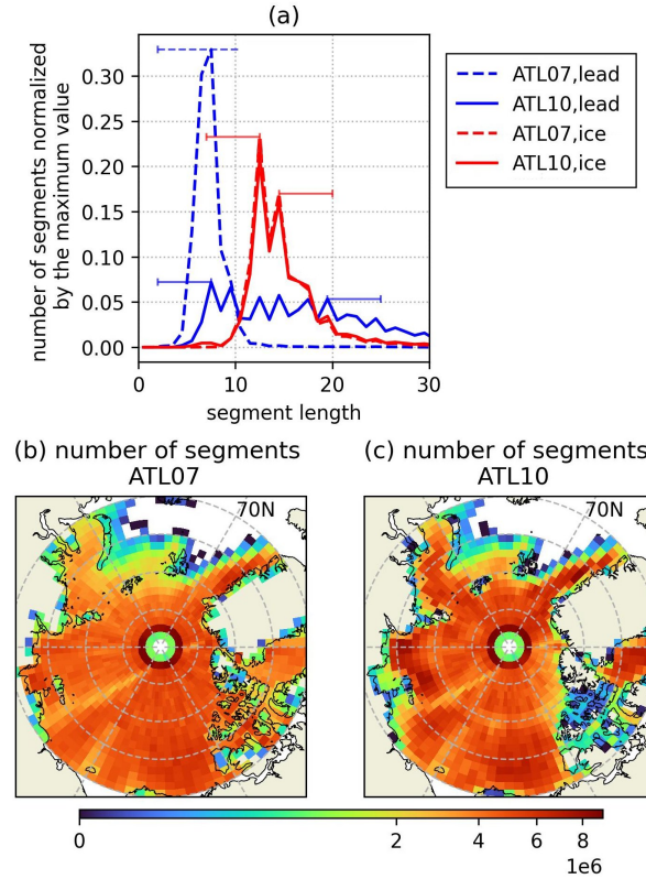
Figure 2. (a) Histogram of length of a single lead (blue) and ice (red) segment in ATL07 (dashed) and ATL10 (solid). Error bars represent half of the ICESat-2 footprint size (5.5 m). (b)-(c) Total number of segments in grid cells of 1^\circ longitude \times 4^\circ latitude in the winter of 2018–2024 in (b) ATL07 and (c) ATL10.
