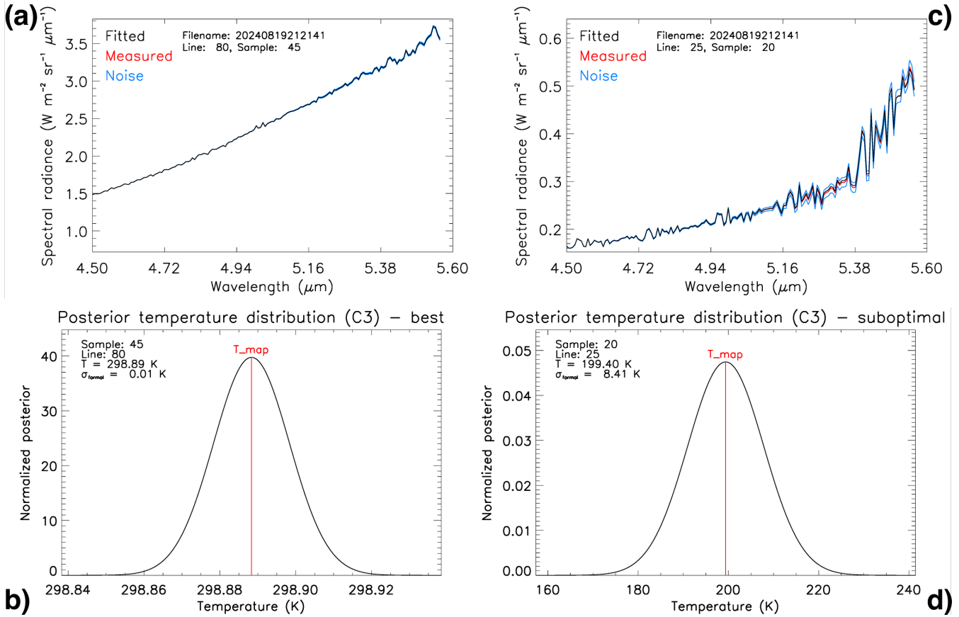
890 Figure A1. Example MAJIS thermal retrievals and associated posterior temperature distributions (C3). (a) Radiance fit for a best-case pixel (sample = 45, line = 80) from the MAJIS C3 observation (file 20240819212141), retrieved over 4.5–5.5 \mu m assuming an initial emissivity prior \epsilon_0 = 0.7 . The measured spectrum (red) is largely overlain by the model fit (black). The Noise Equivalent Spectral Radiance (NESR, light blue) is shown but is difficult to discern at this scale. (b) Corresponding posterior probability density of surface temperature, approximated as a Gaussian centred at the maximum a posteriori estimate T_{map} (red vertical line) with width given by the formal 1-sigma uncertainty from the posterior covariance matrix. (c) Same as (a) for a suboptimal pixel (sample = 20, line = 25), characterized by lower radiance levels and larger relative noise. (d) Corresponding temperature posterior for the suboptimal pixel, showing a broader distribution consistent with the larger formal uncertainty.
