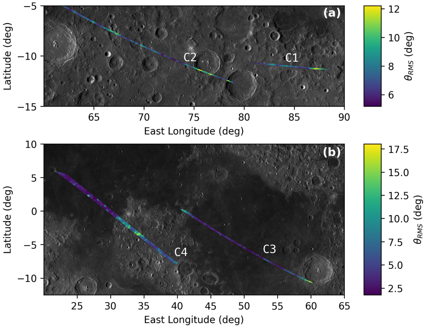
Figure 8. LOLA-derived roughness maps. Estimated large-scale roughness (RMS slope) derived from LDRM_32 LRO/LOLA data, interpolated with a Gaussian filter to match the spatial resolution of the four MAJIS observations: (a) C1 and C2; (b) C3 and C4.
