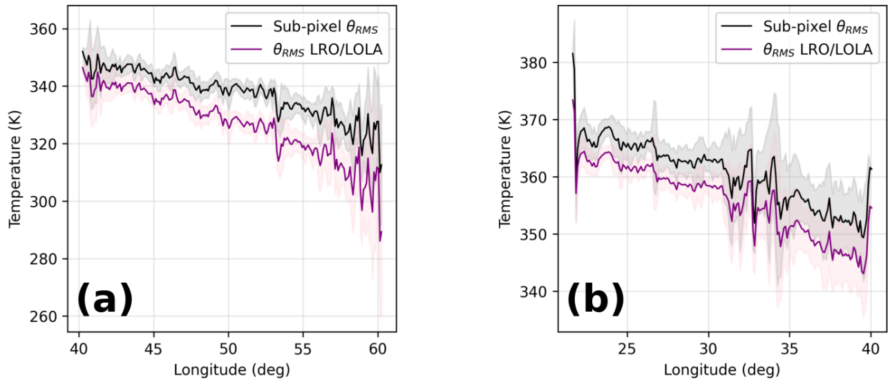
Figure 11. Effect of macroscopic roughness on retrieved surface temperatures (C3–C4). Surface temperature variations computed using the average sub-pixel roughness value (black line) and the macroscopic roughness values derived from LRO/LOLA data (purple line) for the sub-pixel fractal surface generation, shown for C3 (a) and C4 (b). The shaded areas correspond to the 1-\sigma dispersion after binning with a longitudinal step of 0.1^\circ .
