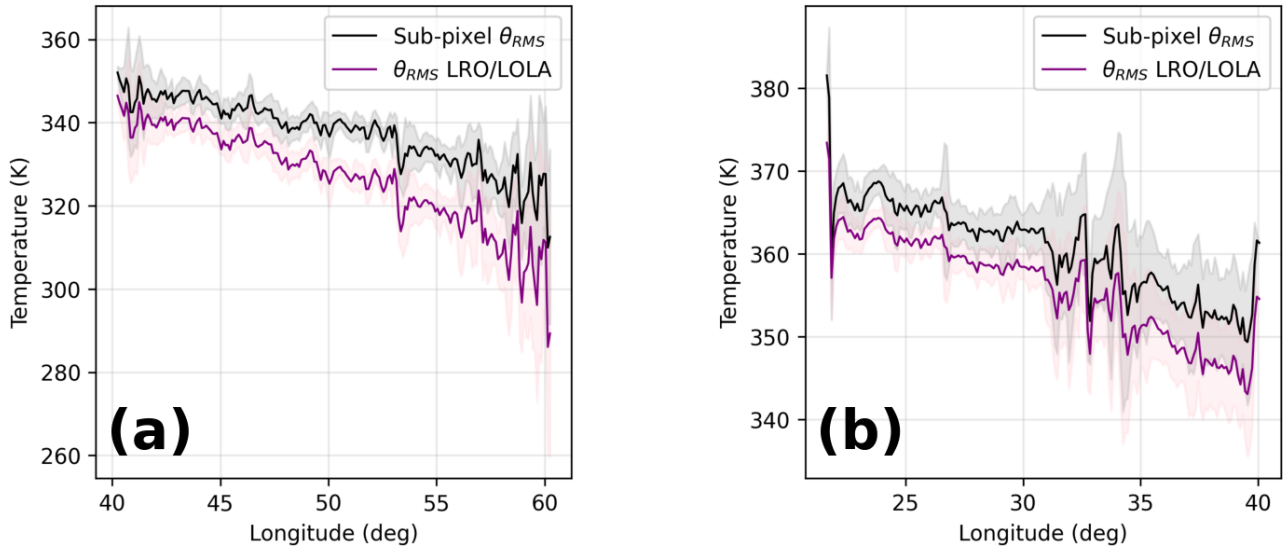
Figure 11. Effect of macroscopic roughness on retrieved surface temperatures (C3–C4). Surface temperature variations computed using the average sub-pixel mm-cm scale roughness value (black line) and the macroscopic meter-scale roughness values derived from LRO/LOLA data (purple line) for the sub-pixel fractal surface generation, shown for C3 (a) and C4 (b). The shaded areas correspond to the 1-\sigma dispersion after binning with a longitudinal step of 0.1^\circ .
