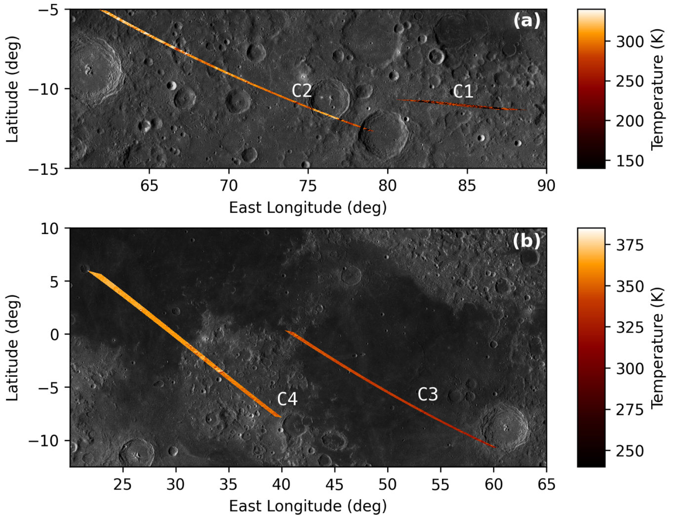
575 Figure 10. Temperatures from roughness-informed model. Temperatures retrieved using the roughness-informed thermal model: (a) C1 and C2; (b) C3 and C4. Spatial variations in the temperatures are primarily controlled by effective illumination conditions (Figure 9) and sub-pixel mm–cm em-mm scale roughness (Table 2). The maximum temperature value (383 K) is observed in the northwestern portion of C4, whereas the lowest values (<150 K) occur in C1 and C2, within areas strongly affected by local topographic shading, corresponding to non-illuminated surfaces ( i > 90^\circ ), as highlighted in Figure 9. Background image: Moon LRO LROC WAC Global Morphology Mosaic 580 100m, June 2013 (Speyerer et al., 2011; Wagner et al., 2015).
