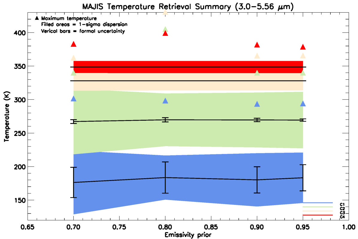
290 Figure 4. Summary of MAJIS temperature retrievals as a function of emissivity prior (3.0–5.56 μm spectral range). The coloured bands show the mean surface temperatures (solid lines) and corresponding \pm 1\sigma dispersion for the four MAJIS observations (C1–C4), obtained from Bayesian inversion without photometric correction. Vertical black bars represent the mean formal uncertainties, and triangles indicate the maximum retrieved temperature values. Compared with the 4.5–5.56 μm case, the wider spectral interval yields similar temperature trends but generally lower formal uncertainties, especially under well illuminated conditions.
