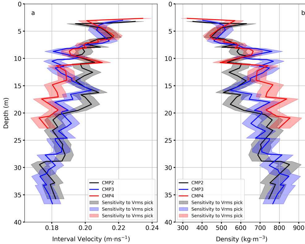
Figure 11. Interval velocity-depth (a) estimated from Vrms velocities picked from Semblance analysis using the Dix Eq. (1) and density-depth (b) profiles estimated from CRIM Eq. (2) using the Ground Penetrating Radar-based Common Mid-point Method (CMP) measurements (Fig. 1) at three locations of the Grosser Aletschgletscher. Sensitivity of interval velocity and density-depth profile for the Vrms picking in semblance analysis (Fig. 4) is shown in the shaded colours of the corresponding solid lines. More details on sensitivity analysis are discussed in section 5.3. All three CMP data sets were acquired on 16 and 17 May 2024.
