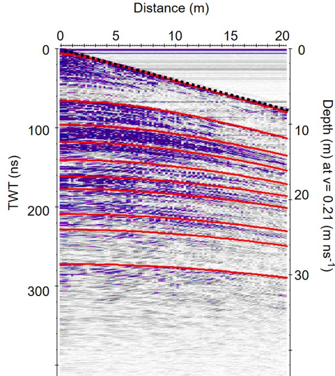
Figure 3. The processed GPR CMP data gathered at Ewigschneefeld on 17 May 2024 (CMP2 in Fig.1). The 20 m long CMP profile depicts various hyperbolic reflections, visible down to a depth of 30-32 m with an assumed constant velocity for two-way traveltime to depth conversion. The left y-axis shows the two-way travel time (tw) in ns, while the right y-axis indicates an approximate depth, assuming a constant radar velocity in firm of 0.21 \text{ m ns}^{-1} . The direct wave (black dotted line) and identified hyperbolic reflectors (solid red lines) are indicated at different depths.
