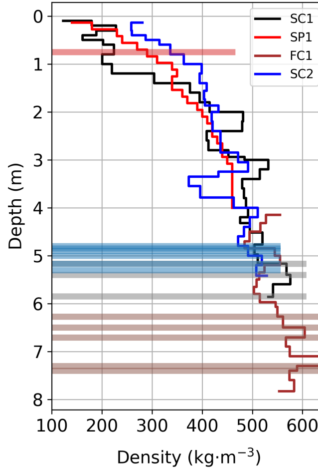
Figure 8. Density-depth profiles obtained from direct measurements using glaciological methods such as snow-pit and firn cores at two locations (Fig. 1). The firn core (FC1) density profile is shown in brown solid line, and was drilled from the bottom of the snow-pit (SP1) depicted as a red line. The black line illustrates the density profile obtained from the snowcore (SC1) drilled a few meters parallel to the snow pit (SP1). All these measurements were taken at the Ewigschneefeld (Fig. 1). The blue line is the density profile estimated from the snowcore (SC2) drilled at the Mönchsjoch plateau (Fig. 1). The ice lenses observed at particular depths were denoted in corresponding coloured horizontal bars. The thickness of observed ice lenses is not to scale.
