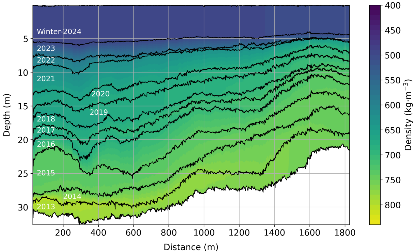
Figure 15. Spatial distribution of firm density along the GPR transect gathered at the Ewigschneefeld. Annual firm layers (black lines) are marked with the attributed years. X-axis is directed from the upper starting point (3550 m) to downvalley (end profile at 3380 m), along the GPR profile (Fig. 1).
