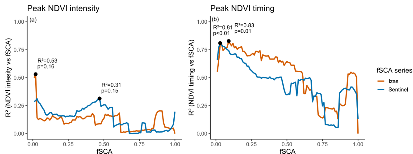
Figure 3. Evolution at each fSCA level of linear model fits between timing of snowmelt and (a) peak NDVI intensity and (b) timing of peak NDVI. Colour-coded for the source of fSCA series.
