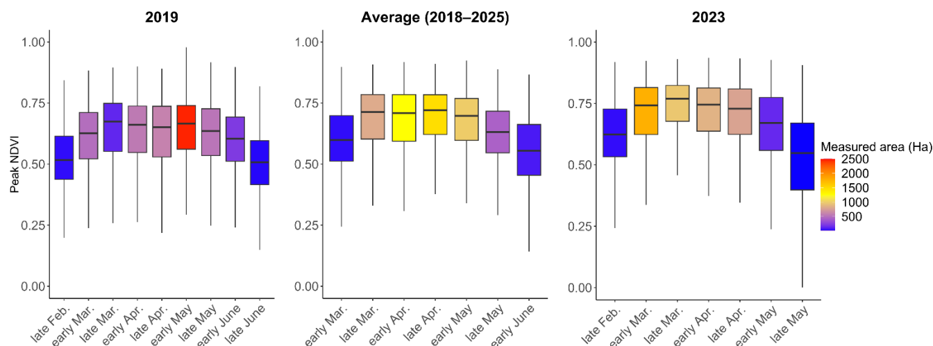
Figure 5. Distribution of values from the annual peak NDVI map in their corresponding SMOD period, colour-coded for covered area.
