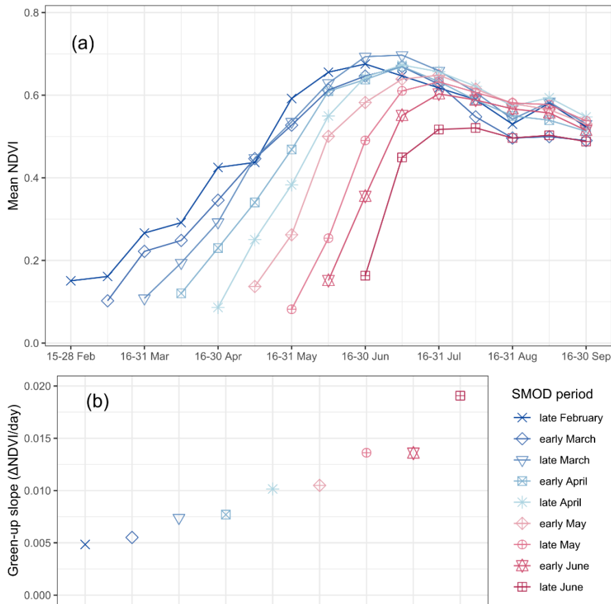
Figure 2. (a) Annual evolution of mean NDVI in each SMOD period zone (Average of the 2018-2025 period). (b) Slope of NDVI curves during growing phase.
