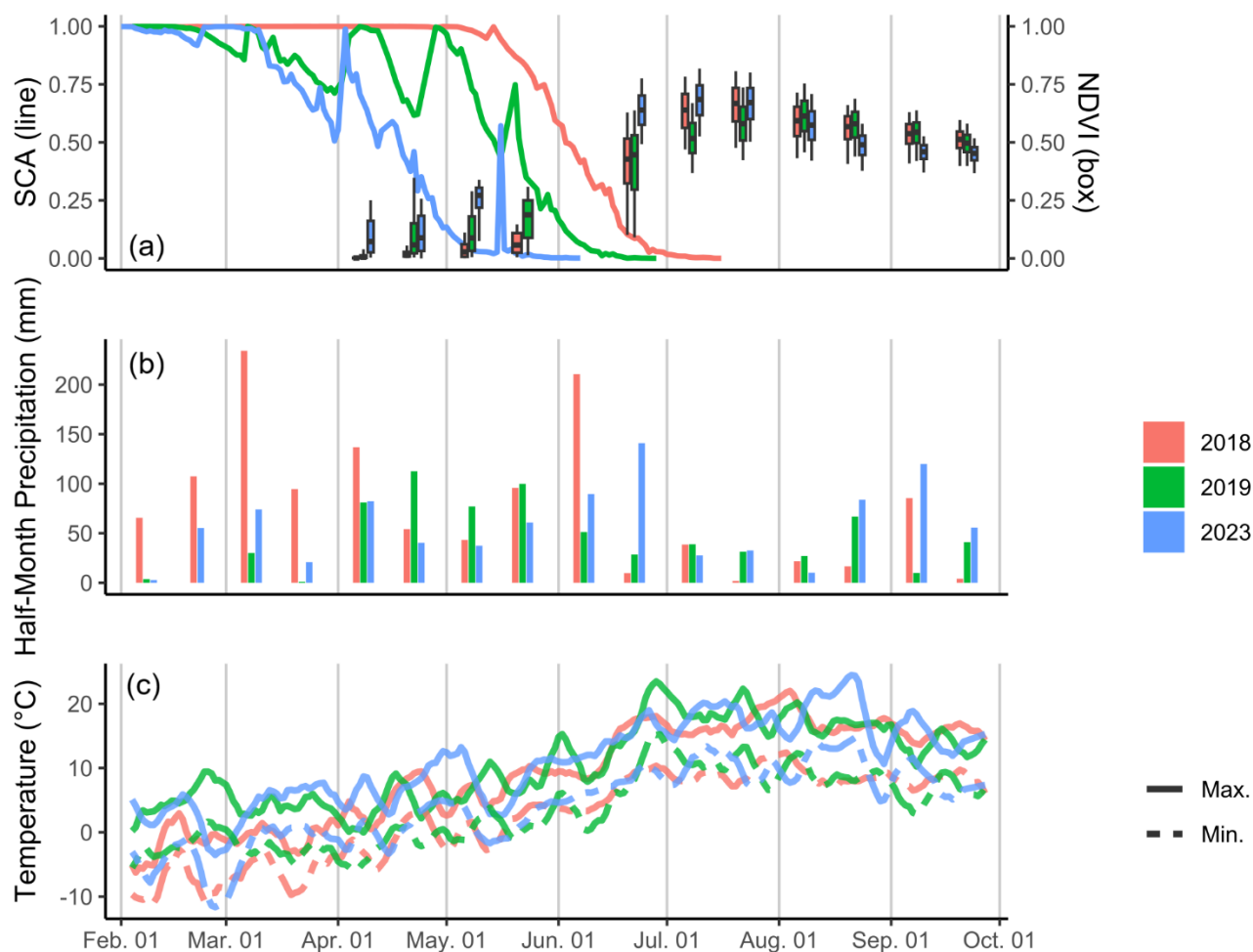
Figure 4. (a) Temporal evolution of fSCA and NDVI. (b) Precipitation from the Canfranc AEMET station, aggregated in 15-day intervals. (c) Maximum and minimum temperatures from the Izas experimental catchment AWS, smoothed by 7-day moving mean.
