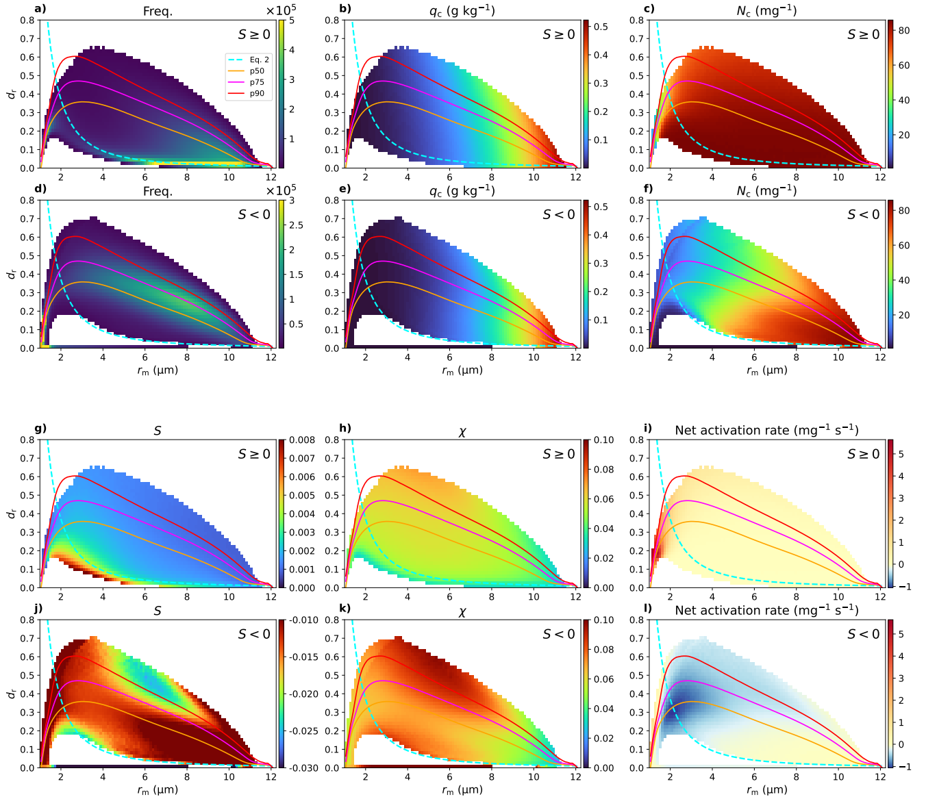
Figure 6. Contour-plots Two-dimensional binned mean values of cloud properties in the r_m and d_r phase space for S \geq 0 (first and third row) and S < 0 (second and fourth row). a) and d) show the frequency distributions, b) and e) show cloud water mixing ratio ( q_c ), c) and f) show cloud droplet number concentration ( N_c ), g) and j) show the mean supersaturation ( S ), h) and k) show mixing fraction ( \chi ) and i) and l) show net activation rate (activation rate - deactivation rate). In each panel, the 50th, 75th, and 90th percentile values (p50, p75, p90), and Eq. 5 from Fig. 4 are indicated by solid lines in orange, magenta, red, and cyan, respectively. Values represent bin-averaged means from 3D simulation results during the final 2 hours of simulation, mapped onto the r_m - d_r phase space.
