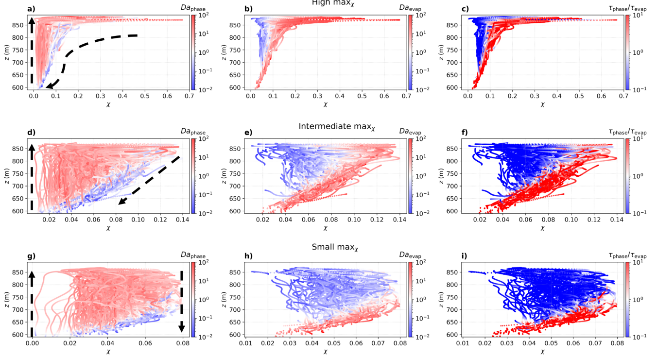
Figure 11. Particle trajectories in the \chi - z phase space, where different colors of dots indicate: the Da_{\text{phase}} ( Da_{\text{phase}} (first column), Da_{\text{evap}} ( Da_{\text{evap}} (second column), \tau_{\text{phase}}/\tau_{\text{evap}} ( \tau_{\text{phase}}/\tau_{\text{evap}} (third column). The first row shows trajectories with the maximum \chi > 0.14 , the third row shows trajectories where the maximum \chi \leq 0.08 , and the second row shows trajectories with intermediate values, where the maximum \chi lies between these two conditions. In panels a), d), and g), the dashed black arrows indicate inferred droplet motion directions based on the vertical velocity W .
