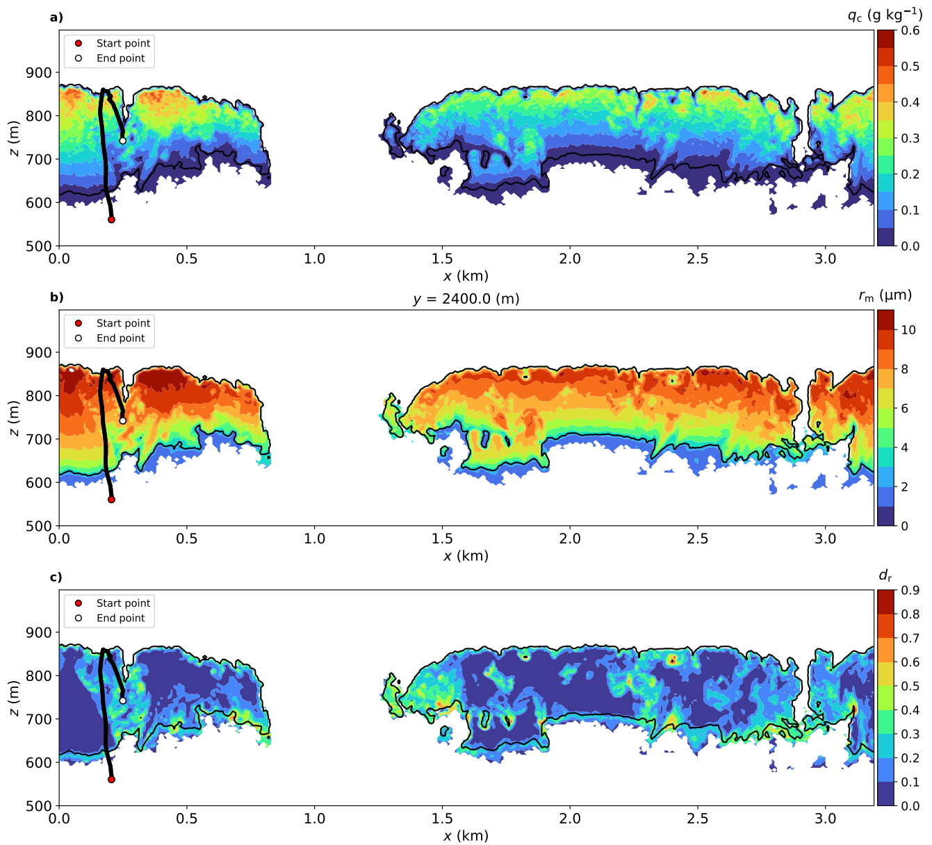
Figure 3. Vertical cross-sections of a) q_c , b) r_m , and c) d_r at y = 2400 m and z , presented as a snapshot at 13320 s of a simulation time of t = 13320 s. The trajectory of thick black line traces the particle-located Lagrangian history of a selected droplet, ending at the end-point its current position (white dot) at this instant and extending backward in time is shown as a thick black line, starting from the to its cloud entry point (red dot). The thin black lines in each panel indicate where the cloud water boundary defined by a mixing ratio q_c = 0.01 g kg -1 of q_c = 0.01 g kg -1 .
