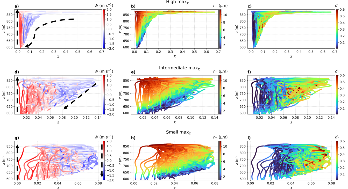
Figure 9. Particle trajectories in the \chi - z phase space, where different colors of dots indicate: the W (first column), r_m (second column), d_t (third column). The first row shows trajectories with the maximum \chi > 0.14 , the third row shows trajectories where the maximum \chi \leq 0.08 , and the second row shows trajectories with intermediate values, where the maximum \chi lies between these two conditions. In panels a), d), and g), the dashed black arrows indicate inferred droplet motion directions based on the vertical velocity W .
