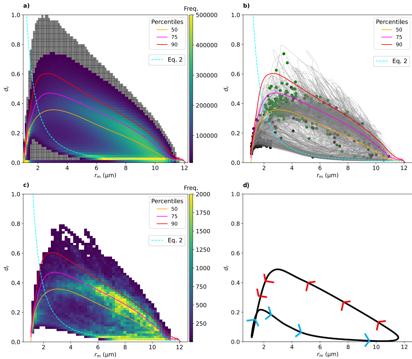
Figure 4. a) Contour plot of the Two-dimensional frequency distributions histogram in r_m and d_r phase space. b) Corresponding droplet evolution pathways (gray dotted lines) with start/end points in black/green. c) The corresponding frequency distribution of droplet evolution pathways. d) Conceptual schematic summarizing the composite evolution loop, constructed from the most frequently observed trajectory patterns in the r_m-d_r phase space. Blue and red arrows represent the dominant directions of growing and decaying pathways, respectively, based on the Lagrangian trajectory. In each panel, 50th, 75th, and 90th percentiles at each r_m value and Eq. 5 are indicated as solid lines in orange, magenta, red, and cyan, respectively. In panel a, the gray-shaded regions indicate areas where the sample count is below 10,000, which are masked for statistical robustness.
