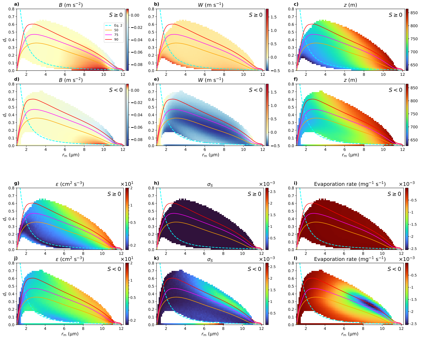
Figure 7. Contour plots—Two-dimensional binned mean values of cloud properties in the r_m and d_r phase space for S \geq 0 (first and third row) and S < 0 (second and fourth row). a) and d) show buoyancy ( B ), b) and e) show vertical velocity ( W ), c) and f) show height ( z ), g) and j) show kinetic dissipation rate ( \varepsilon ), h) and k) show supersaturation fluctuation ( \sigma_s ) and i) and l) show the evaporation rate. In each panel, the 50th, 75th, and 90th percentile values (p50, p75, p90), and Eq. 5 from Fig. 4 are indicated by solid lines in orange, magenta, red, and cyan, respectively. Values represent bin-averaged means from 3D simulation results during the final 2 hours of simulation, mapped onto the r_m – d_r phase space.
