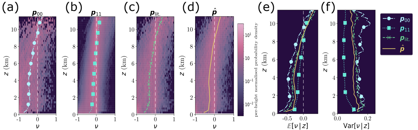
Figure 8. Bias distributions between ATL09 and Cloudnet VCF profiles as a function of height for the parametrisations p_{00} (a), p_{11} (b), p_{lit} . (c) and \hat{p} (d). Expected bias profiles are given as coloured dashed lines. (e) The expected bias profiles for the different parametrisations plotted together, using the same line styles and markers as in their individual panels. (f) The variance in the bias distributions as a function of height.
