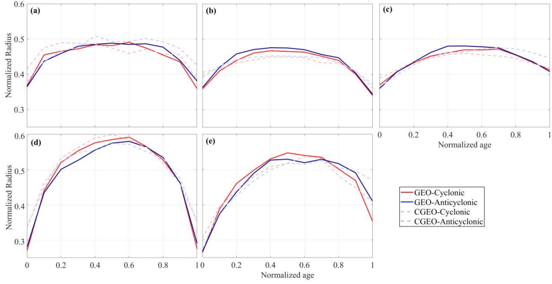
Figure 8 Temporal evolution of the mean normalized radius for the (a) SCS, (b) CC, (c) KE, (d) AI, and (e) HI. Each life stage is defined by normalized age: generation ( \sim 0-0.1 ), intensification ( \sim 0.1-0.3 ), maturation ( \sim 0.3-0.8 ), and decay ( >0.8 ).
