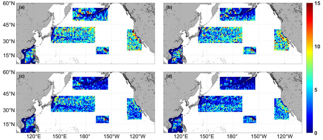
Figure 10 Spatial distribution of the number of eddies generated. The AEs and CEs detected by geostrophic currents are shown in (a) and (b), respectively. The AEs and CEs detected by cyclogeostrophic currents are shown in (c) and (d).
