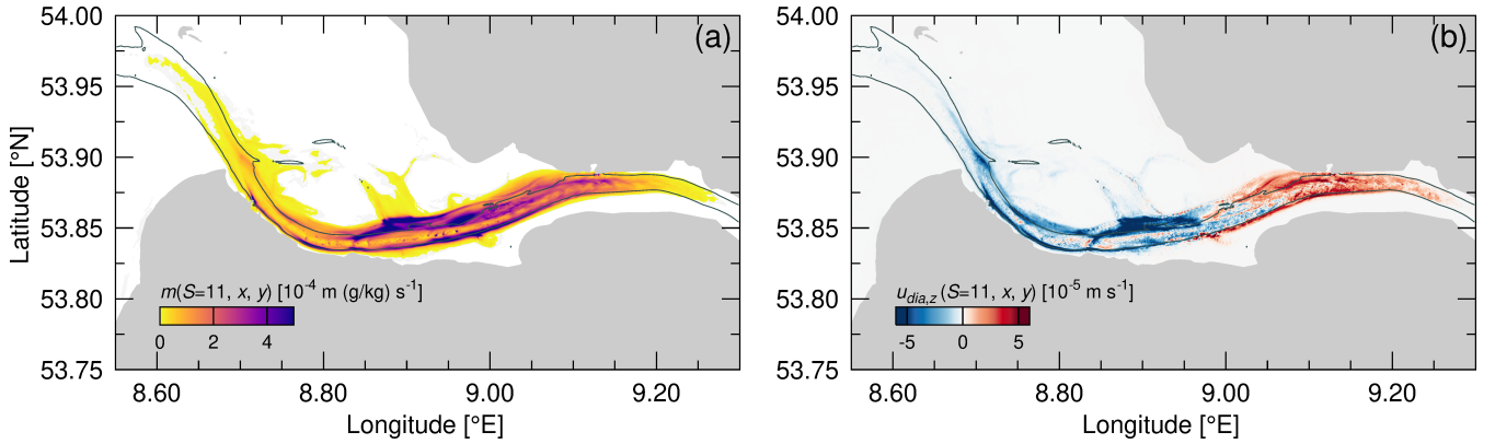
Figure 7. Dihaline mixing m (panel a) and diahaline entrainment velocity u_{\text{dia},z} (panel b) across the isohaline surface of 11 g/kg, averaged over two spring-neap cycles during April 2024 in the lower Elbe River estuary in Germany. The line in both panels shows the 10 m isobath.
