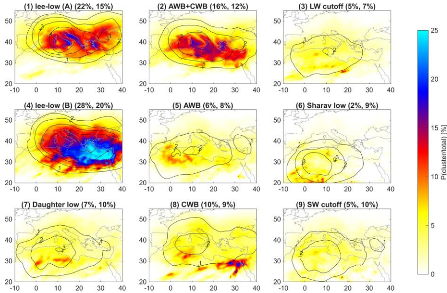
286 Figure 5: As Figure 4 but for P.
