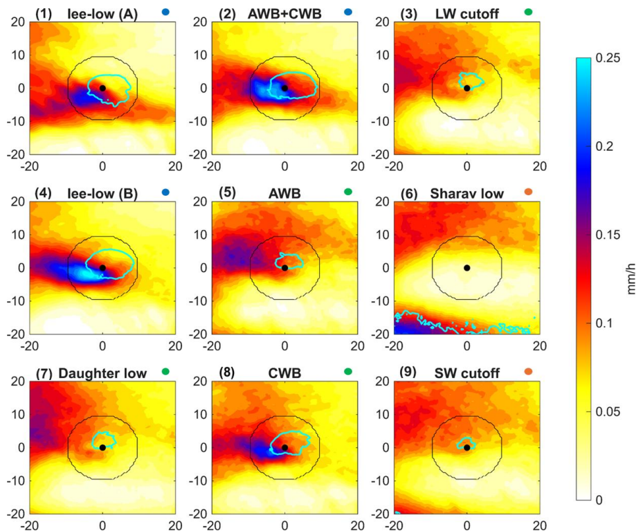
246 247 Figure 3: cyclone-centered cluster composites of E (shading) and P (cyan contours, 0.25 mm/h) at classification 248 time (minimum SLP time of each MC track). The black circles denote the 10° radius impact area considered for 249 cyclone-induced fluxes. Colored circles indicate the dominant season for each cluster: blue for winter, red for 250 summer, and green for spring/autumn.
