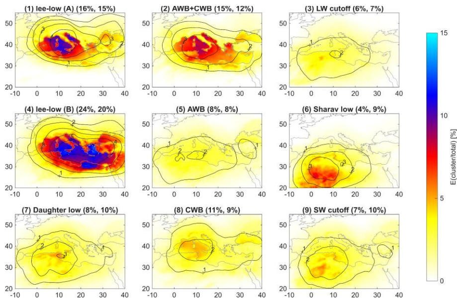
268 269 Figure 4: Relative contribution of each cluster to total E (shading, %) and cluster mask frequency (black contours, 270 % in 1% intervals). Titles denote cluster numbers and the dominant driving mechanism as reported in Givon et 271 al., (2024a). Numbers in brackets indicate the mean contribution of each cluster to total MC-induced surface 272 evaporation (left) and the mean cluster frequency out of all MCs (right).
