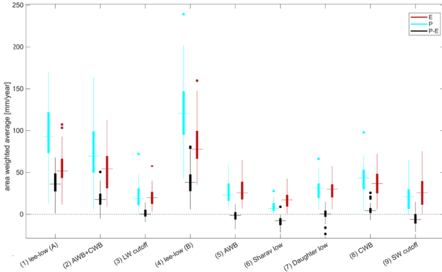
296 Figure 6: Distributions of area weighted annual mean MC-induced E, P, and P-E, separated by cluster. The 297 medians of each distribution are denoted by the horizontal lines, the boxes mark the 25 to 75 percentiles of the 298 distribution, and whiskers mark the 2.5 and 97.5 percentiles, setting the threshold for outliers, marked by the 299 colored dots.
