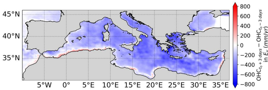
363 364 Figure 9: Composites of the difference in ocean heat content \pm 3 days before and after the influence of a MC, 365 normalized by annual MC frequencies. Negative values indicate net heat extracted from the ocean towards the 366 atmosphere.
