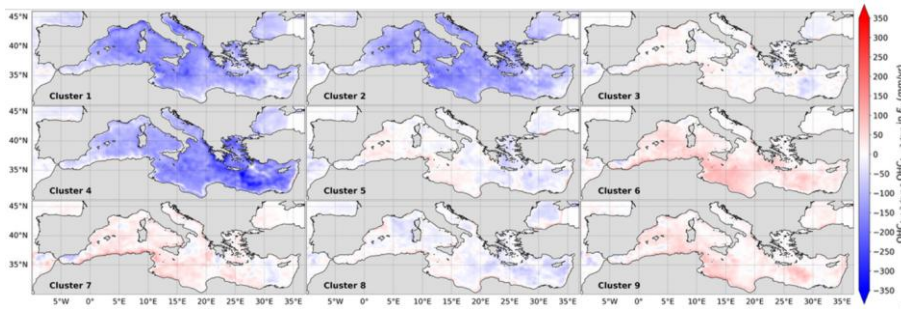
367 368 Figure 10: As Figure 9 but separated into clusters. Note that the values are normalized by annual MC cluster 369 frequencies, thus representing the net heat taken from (negative values) and added to (positive values) the 370 Mediterranean per cluster, per year.
