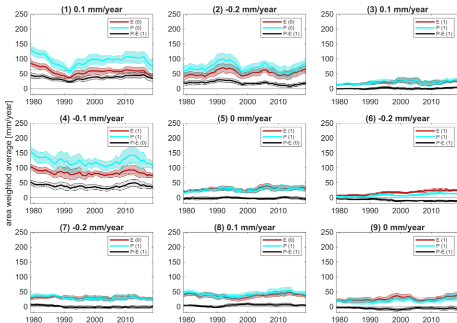
312 313 Figure 7: As Figure 2 (b) but separated by cluster. Titles denote the cluster number followed by the slope of the 314 linear best-fit (mm/year) for the P-E trend. The result of a 95% confidence level Mann-Kendall test for each 315 component is shown in the legend (1 for a significant trend)
