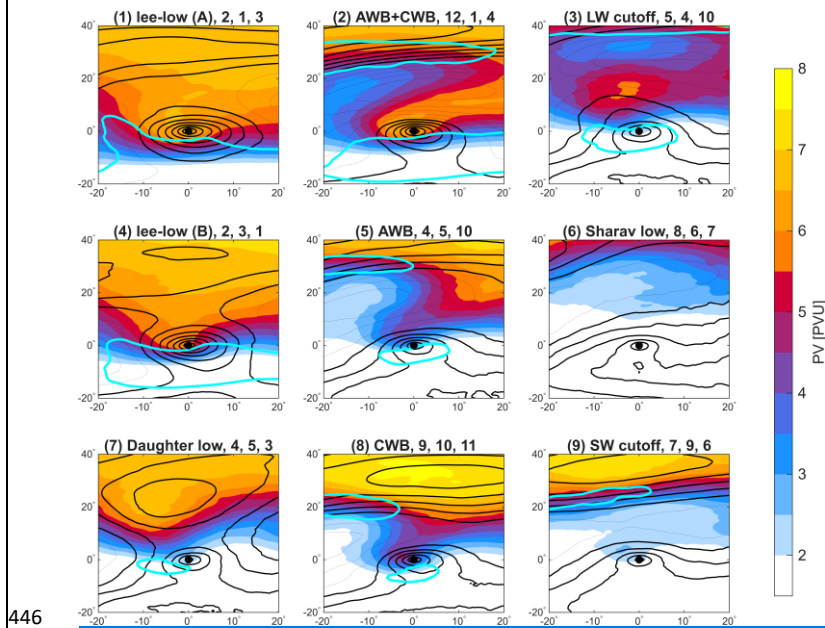
446 447 Figure A1: Cyclone-centered cluster composites of upper-level (320–340 K averaged) PV (PVU, shading) and 448 SLP (black contours at 2 hPa intervals, dashed above 1015 hPa) at minimum SLP time. Overlaid is the 449 corresponding composite of the 30 m s -1 isotach on the 300 hPa geopotential surface (cyan contour, roughly 450 denoting the subpolar and/or subtropical jets). Titles denote cluster number, name, and the leading cluster months 451 in a descending order.
