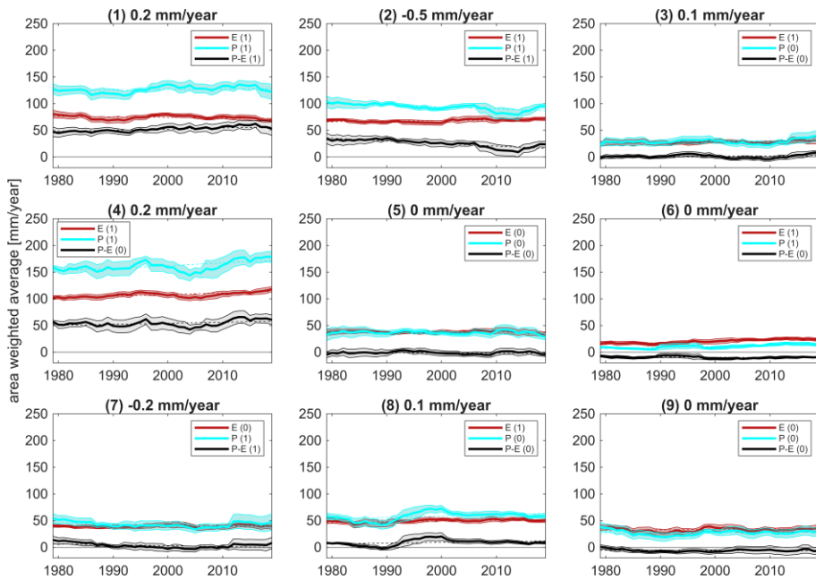
328 Figure 8: As Figure 7 but normalized by cluster frequencies, highlighting flux-intensity variations.
