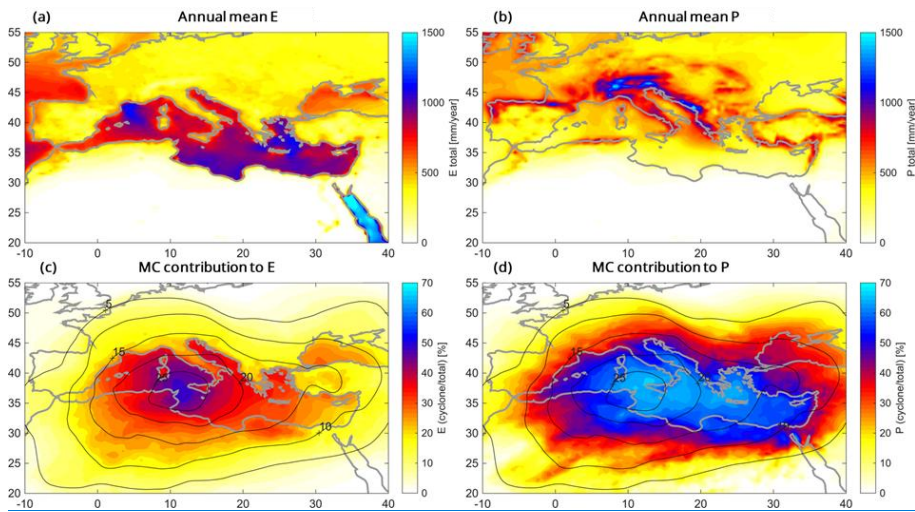
218 Figure 1: Annual-mean E (a) and P (b), and the relative contribution of MCs to both E (c) and P (d), in shading, 219 E and P respectively) along with mean cyclone frequency \bar{F}_{MC} (black contours, %).
