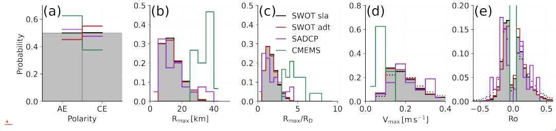
Figure 3. Probability distribution of eddy statistics detected by SWOT using SLA (gray bars, solid black lines) or ADT (red lines) , in comparison with ADCP (purple) and CMEMS (green) a) Polarity of detected eddies, expressed as the proportion of anticyclonic (AE) and cyclonic (CE) structures. b) Distribution of radius of maximum azimuthal velocity R_{\max} . c) Distribution of R_{\max} normalized by the first baroclinic deformation radius R_D . d) Distribution of maximum azimuthal velocity V_{\max} . e) Distribution of the Rossby number Ro of detected eddies; for CMEMS, the probability reaches 0.6 for -0.05 < Ro < 0 and 0.4 for 0 < Ro < 0.05 . In panels c and d, dotted lines are distributions including all detections prior to depth filtering ( i.e. , < 2000 including eddies on shelves).
