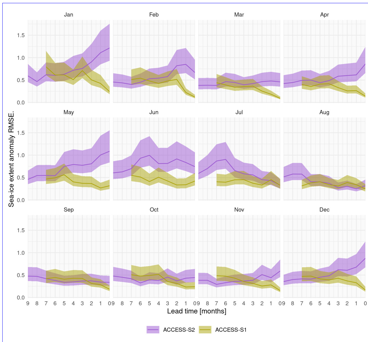
Figure A1. RMSE of monthly mean sea-ice extent anomalies as a function of lead time (months) for ACCESS-S1 (green) and ACCESS-S2 (purple). RMSE is computed over the overlapping period of ACCESS-S1 and ACCESS-S2 hindcasts (1990–2013). Each panel indicates the target month. Note the reverse horizontal axis.
