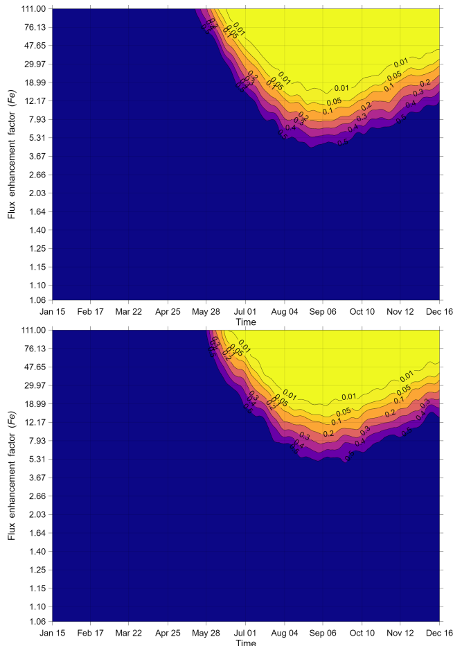
Figure 10. Contour plot of the Yedoma \text{CH}_4 flux detection limit of MERLIN. Shown for the 28 d bin sizes which retain most of the temporal variation. The top panel shows pure detection limits under the union of the Land > 0.5 and Full subsets, the bottom panel the detection limits of Full including high transport modelling errors. Non linear y axis shows flux enhancement (Fe), on the x axis the date (centre of 28 d bins). Colours and isolines indicate the detection limits as statistical significance ( q value) of the differences between the baseline and enhancement scenarios. Note that the peak emissions were during September.
