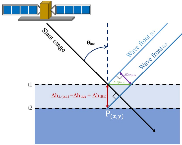
Figure 3. Side-looking spaceborne SAR imaging geometry. A vertical displacement of a Point P_{(x,y)} from t_1 to t_2 is imaged at different slant range positions ( \Delta D_{sr(t_2, t_1)} ) depending on its elevation.
