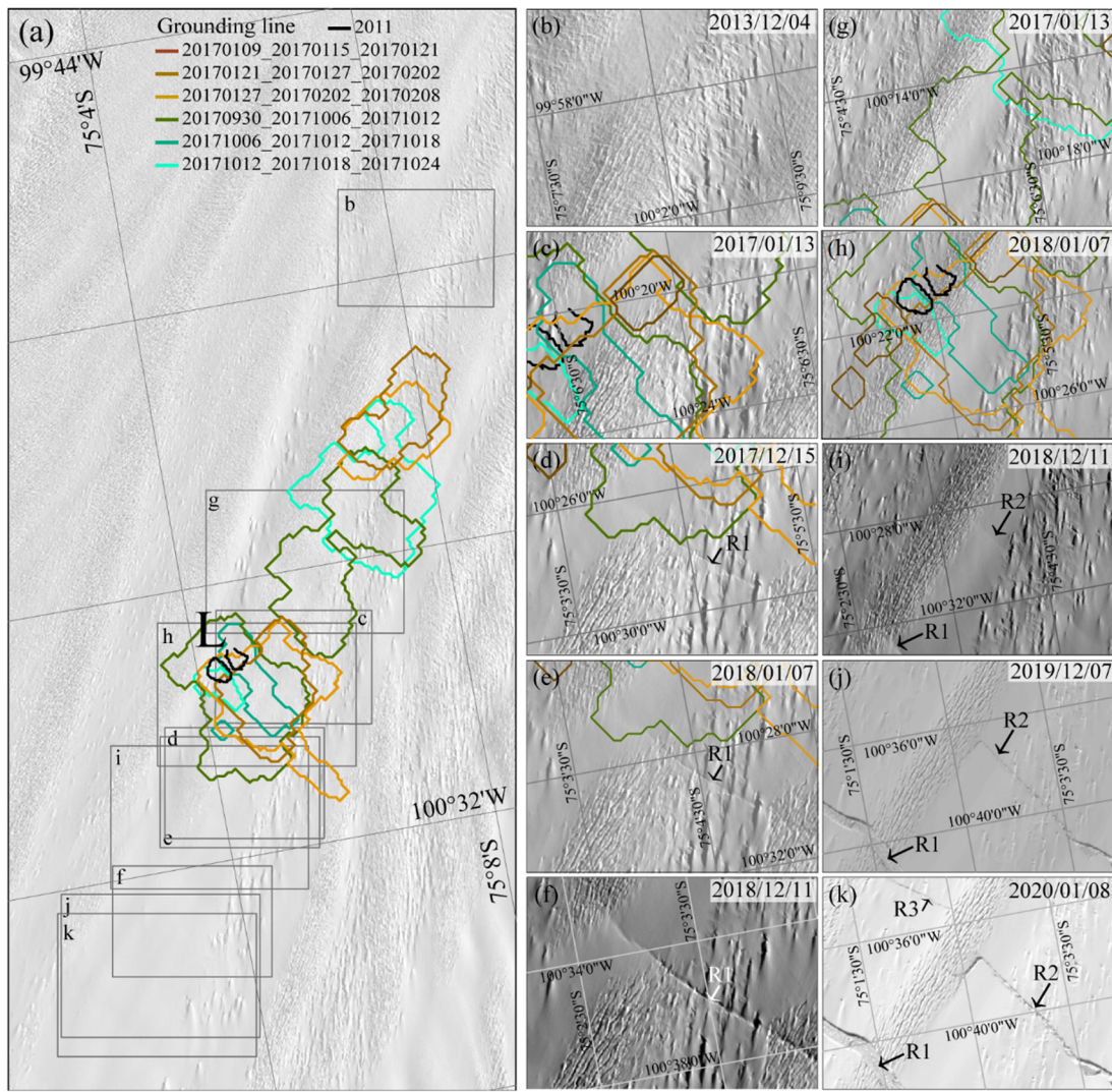
305 Figure 10. Rift propagation history from 2013 to 2019. (a) Overview map showing the positions of panels (b) to (k). The background image is a Landsat-8 panchromatic image from 4 December 2013. (b)-(k) show the propagation history of the rifts R1, R2 and R3 (black or white arrow), which led to the 2020 calving event. The black circles indicate the positions of ice rumple L. Grounding lines are delineated based on the near-zero value of the double-differential vertical displacement.
