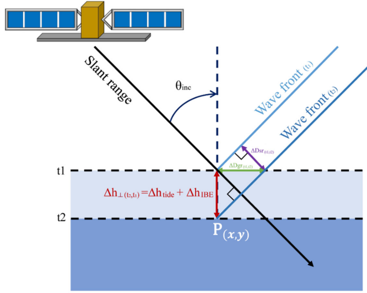
Figure 3. Side-looking spaceborne SAR imaging geometry. A vertical displacement of a Point P_{(x,y)} from t_1 to t_2 is imaged at different slant range positions ( \Delta D_{sr(t_2,t_1)} ) depending on its elevation.
