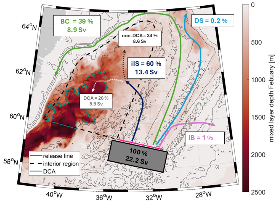
440 Figure 7: Schematic showing the percentages and volume transports of the particle classification in various categories; Denmark Strait (DS) particles leave the Irminger Sea through Denmark Strait, Iceland Basin (IB) particles spend more than 40 days in the Iceland Basin, Boundary Current (BC) particles follow the cyclonic boundary current and never enter the defined interior Irminger Sea region and Interior particles do enter the interior Irminger Sea. A second selection step further subdivides these interior Irminger Sea particles into those entering the Deep Convection Area (DCA) , (compare Figs. 2c, 4) and those staying outside of the defined DCA ( non-DCA ). Note that these volume transports represent the time-mean absolute volume transport released within six months across the OSNAP IC section. In the background, the February mixed layer depth (shading), model bathymetry (grey contours) and the 1500 m-contour line of the mixed layer depth (thick turquoise line). The pink line marks the particle release line along the OSNAP IC mooring array for reference.
