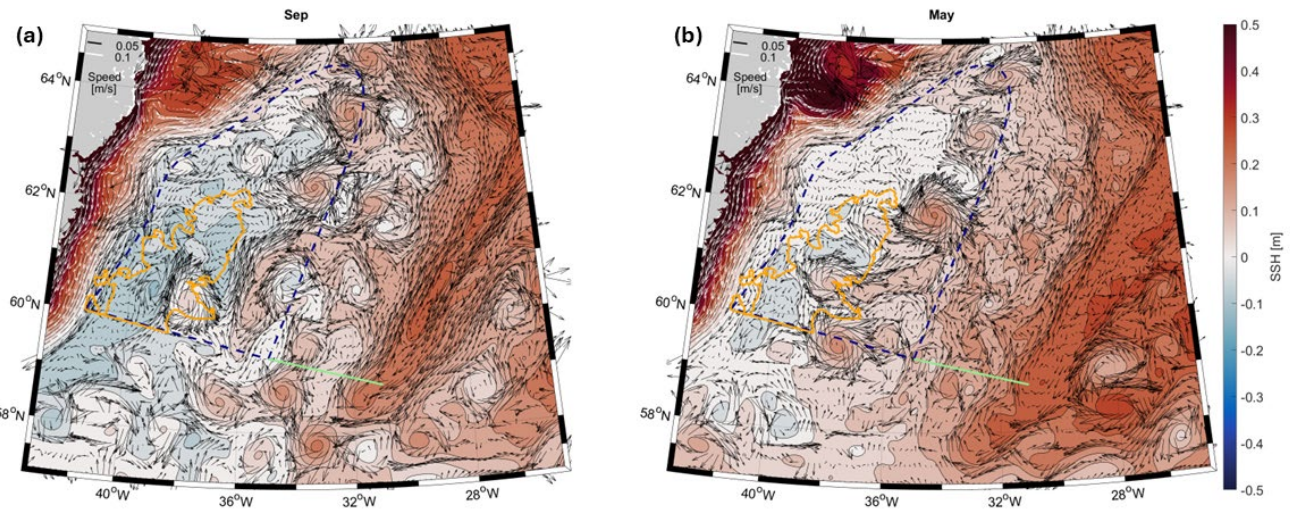
465 Figure 8: Eddy activity in the Irminger Sea from the MITgcm model simulation. Monthly mean sea surface height (SSH, shading) with overlaid one year-averaged circulation over the upper 1500 m (arrows) from the model simulation for (a) September and (b) May. Velocities smaller than 0.1 \text{ m s}^{-1} are indicated by black arrows, larger velocities by white arrows; we only plot every 8 th latitudinal grid point and every 4 th longitudinal grid point for clarity. In all subpanels the green line marks the release line, the dashed line the interior region and the orange line the DCA.
