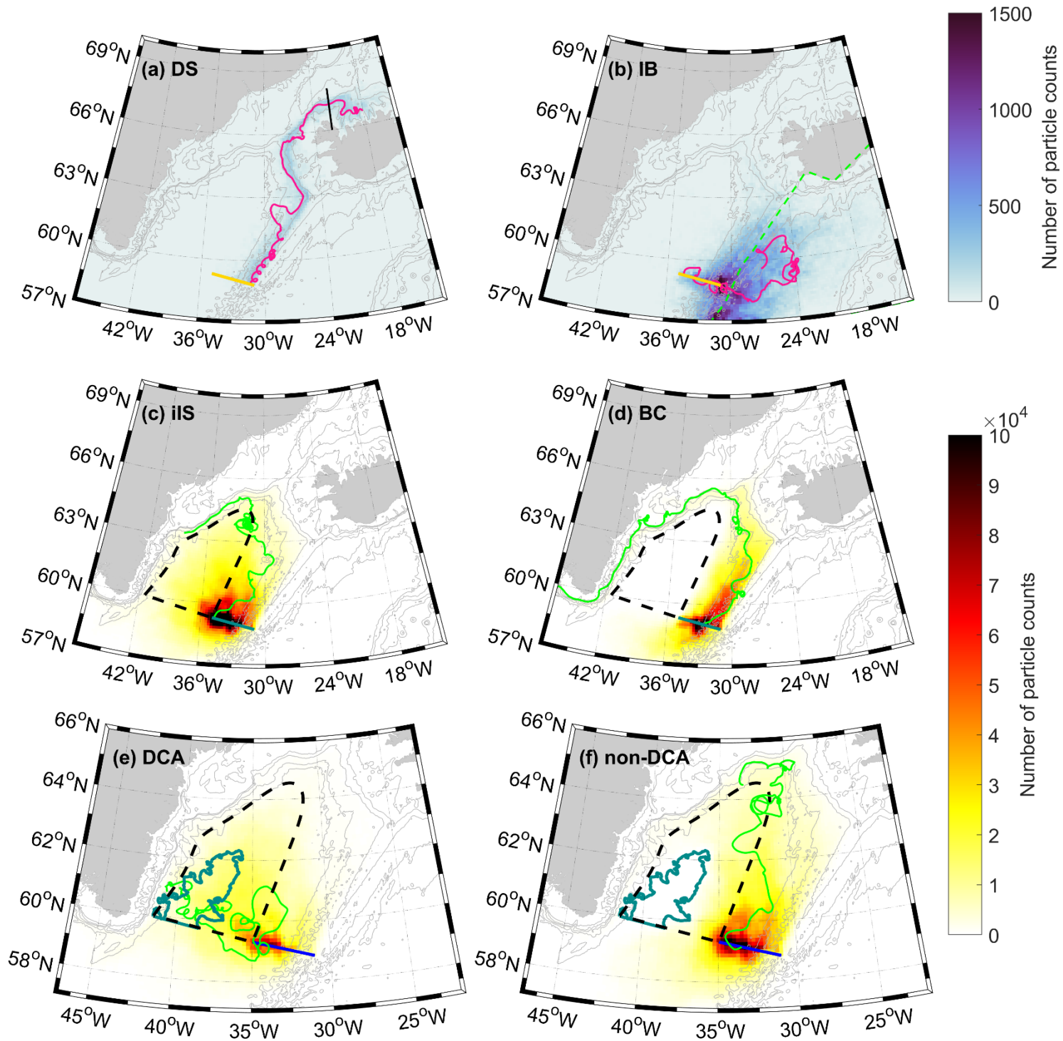
270 Figure 4: Particle density maps of particles released at the OSNAP IC moorings. Particle density distribution for (a) Denmark Strait 275 particles and (b) Iceland Basin particles. The pink line marks an example particle track and the orange line the release line. Dashed black line in (a) and green dashed line in (b) geographically mark the selection criterion for DS and IB respectively. Particle density distribution for (c) interior and (d) boundary current with example particle tracks (green) and interior Irmingier Sea definition (dashed line); release line is marked in greyish blue. (e) DCA particles and (f) non-DCA particles with example particle tracks (green), contours defining the interior Irmingier Sea (dashed line) and the DCA (blue); dark blue line marks the particle release line. Note the different colorbar limits are used for (a-b) compared to (c-f) because of the large difference in particle amount per grid box.
