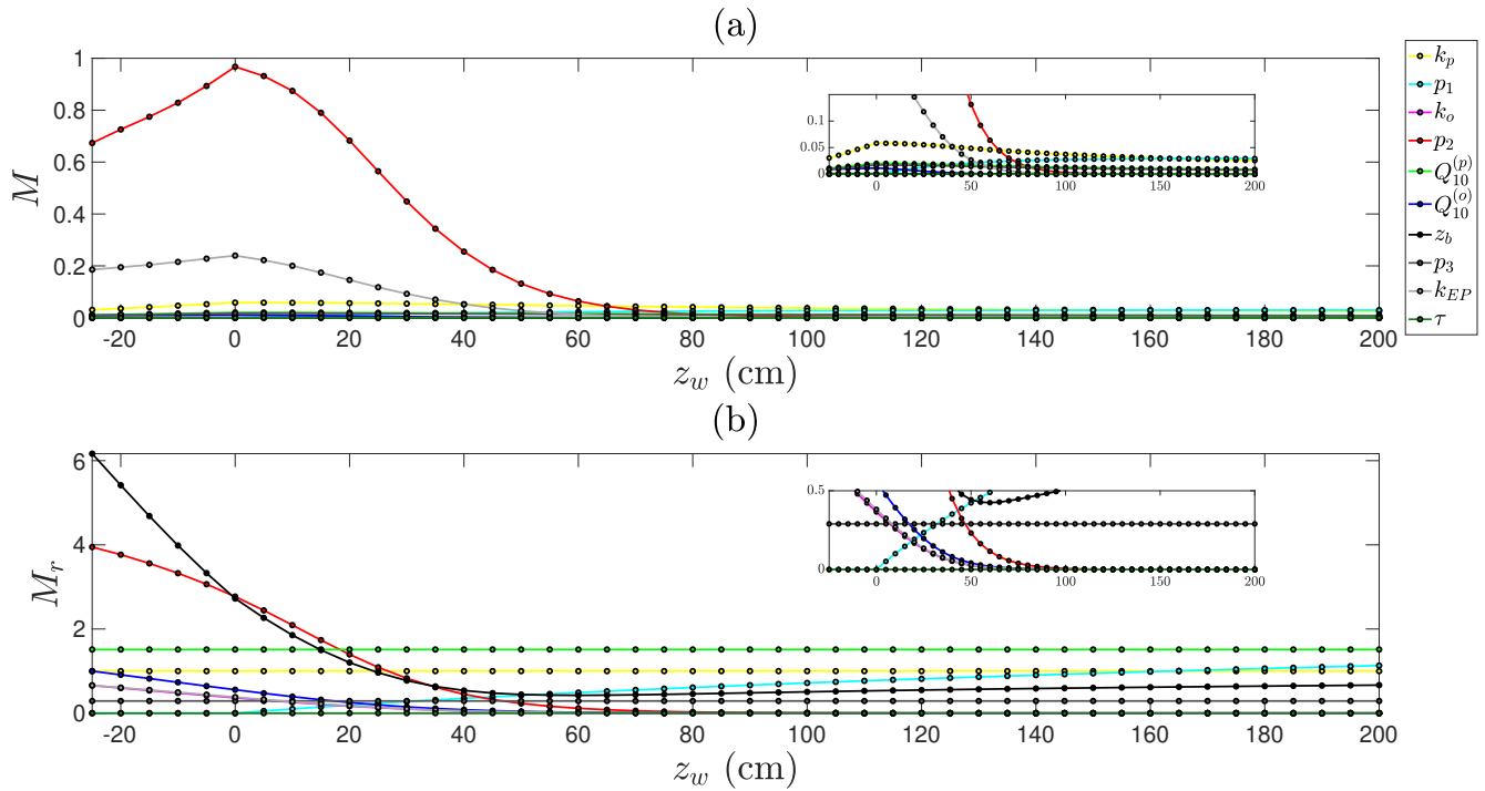
Figure A2. Sensitivity analysis of predicted steady-state \text{CH}_4 emission fluxes across water table depths, with constant NDVI and temperature. (a) Absolute Morris indices and (b) relative (normalised) Morris indices for each parameter as a function of water depth.
