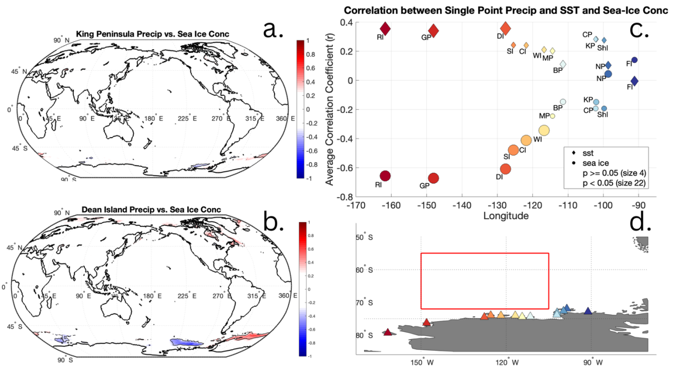
Figure 9: Sea surface temperature and sea ice concentration comparison. Panels a and b: correlation between precipitation at each ice rise and global sea ice concentration at King Peninsula (a) and Dean Island (b). Panel c: correlation between precipitation at each ice rise and sea surface temperature (SST, diamond) as well as sea ice concentration (SIC, circle) averaged over the Amundsen Sea box (panel d).
