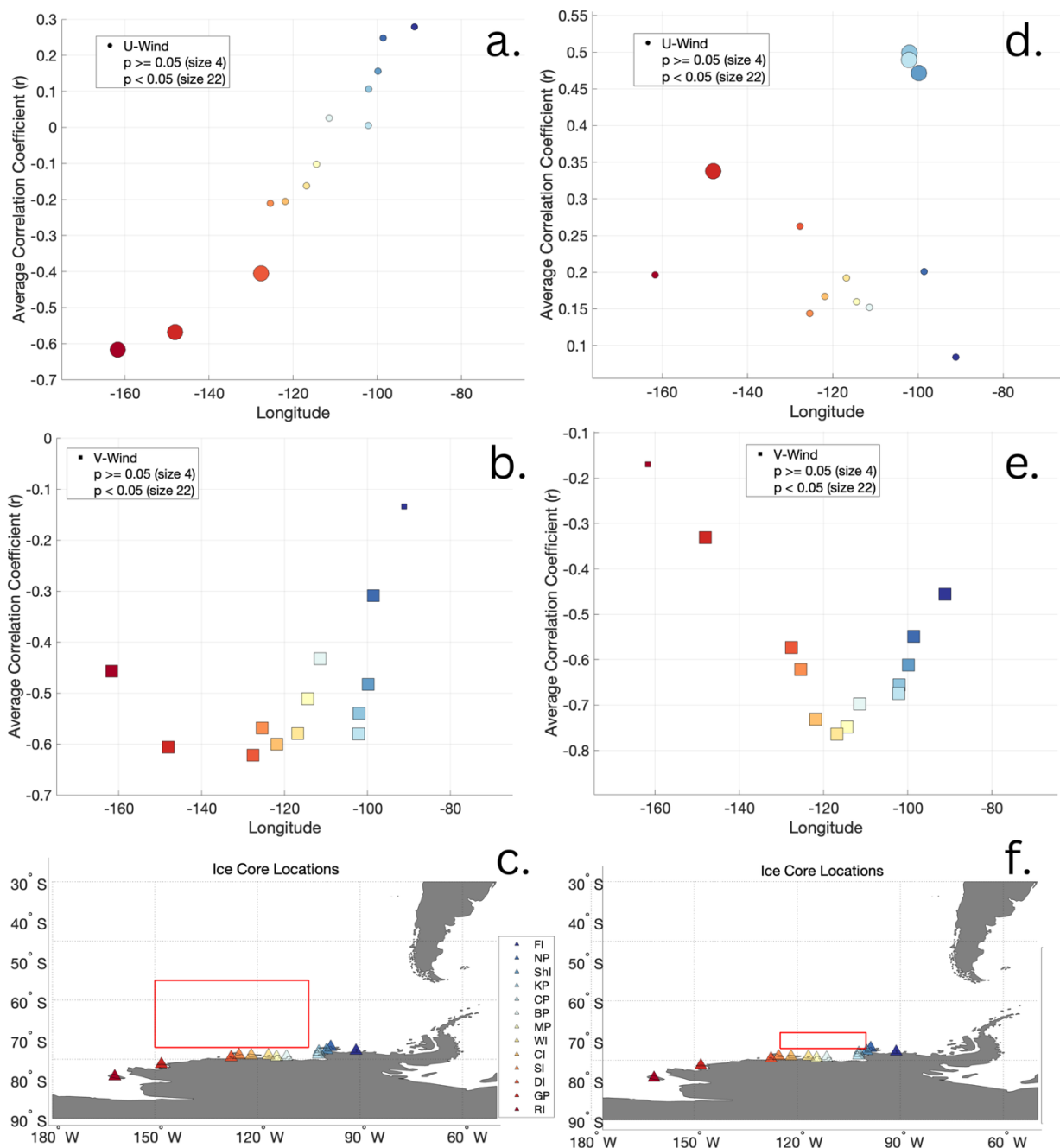
Figure 4: Correlation analysis between snowfall and zonal winds and meridional winds within a broad Amundsen Sea box (a-c) and the Steig et al. (2012) coastal box (d-f).
