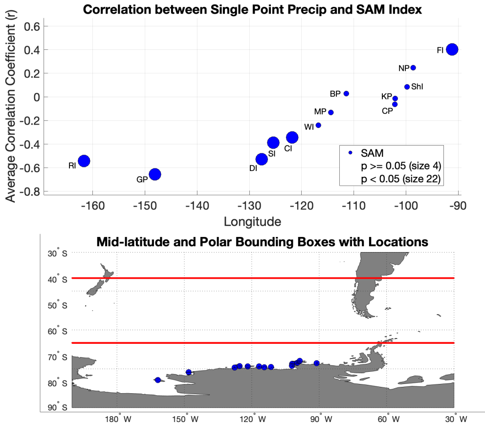
Figure 5: Correlation between precipitation at each ice rise and the Southern Annular Mode Index (Marshall, 2003). The index is defined by averaging MSLP across narrow latitude bands centered on –40° and –65° (red lines) and calculating the difference.
