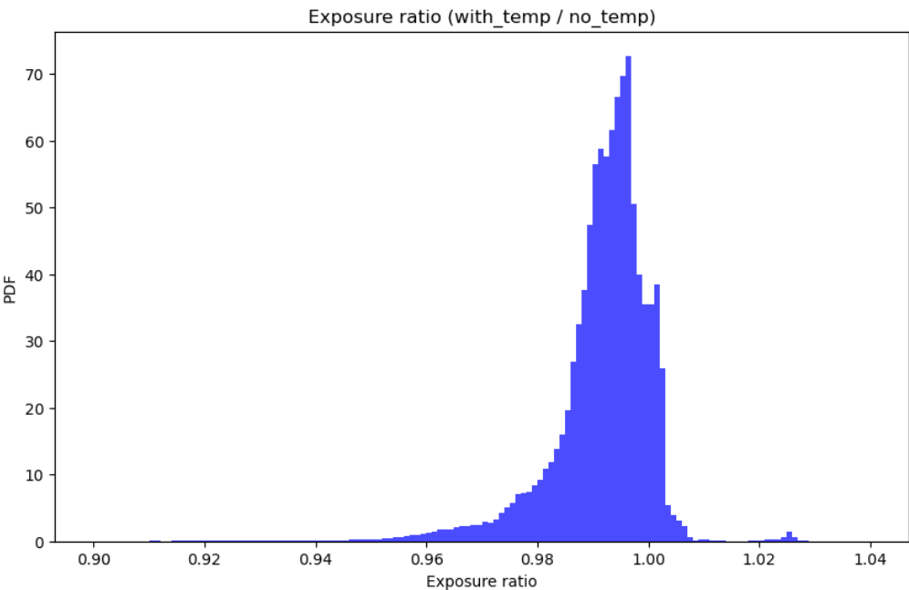
645 Figure A10 Ratio between risk level (Local Personal Risk) computed with temperature effects and without temperature effects. For each building, for each year in the forecast, and for each scenario we obtain a ratio. We show this as a single histogram, combining all the annual data of all scenarios in a single plot. In general, the risk level computed per building with temperature effects is a few percent lower than without temperature effects due to the slightly lower levels of seismicity. However, for some select buildings the ratio is slightly above unity. The main take-away is that the effect of accounting for temperature effects is very minor.
