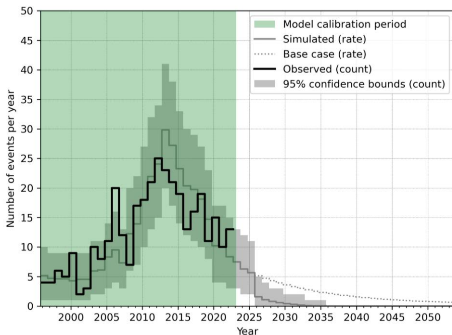
620 | Figure A2 Number of events per year in the Groningen field of magnitude M1.5 and above for the LO-10ZB scenario (without temperature effects included). The solid grey line is the modelled expected number of events, the grey area gives the 95% confidence bounds per year. The solid black line is the historically observed event rate and the green area is the period over which the model is calibrated. The dotted reference line represents the base case for comparison.
