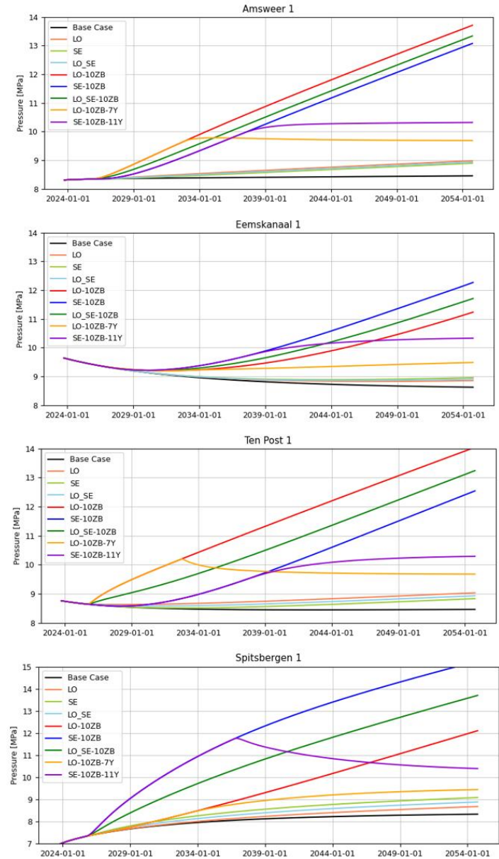
330 Figure 4 Simulated near-well average reservoir pressure [MPa] around 4 wells from 4 different production regions: Amsweer 1, located in the East-Central region, Eemskanaal 1, located in the Eemskanal region, Ten Post 1, located in the Loppersum region, and Spitsbergen 1, located in the South-West region. Results are shown for all scenarios. The wells are not used for injection.
