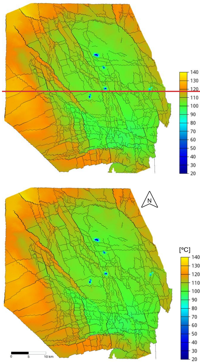
Figure 5 Temperature [°C] at mid-reservoir depth (Upper Slochteren formation) in 2054 for injection scenario LO-10ZB, for an injection temperature of 10 °C.
