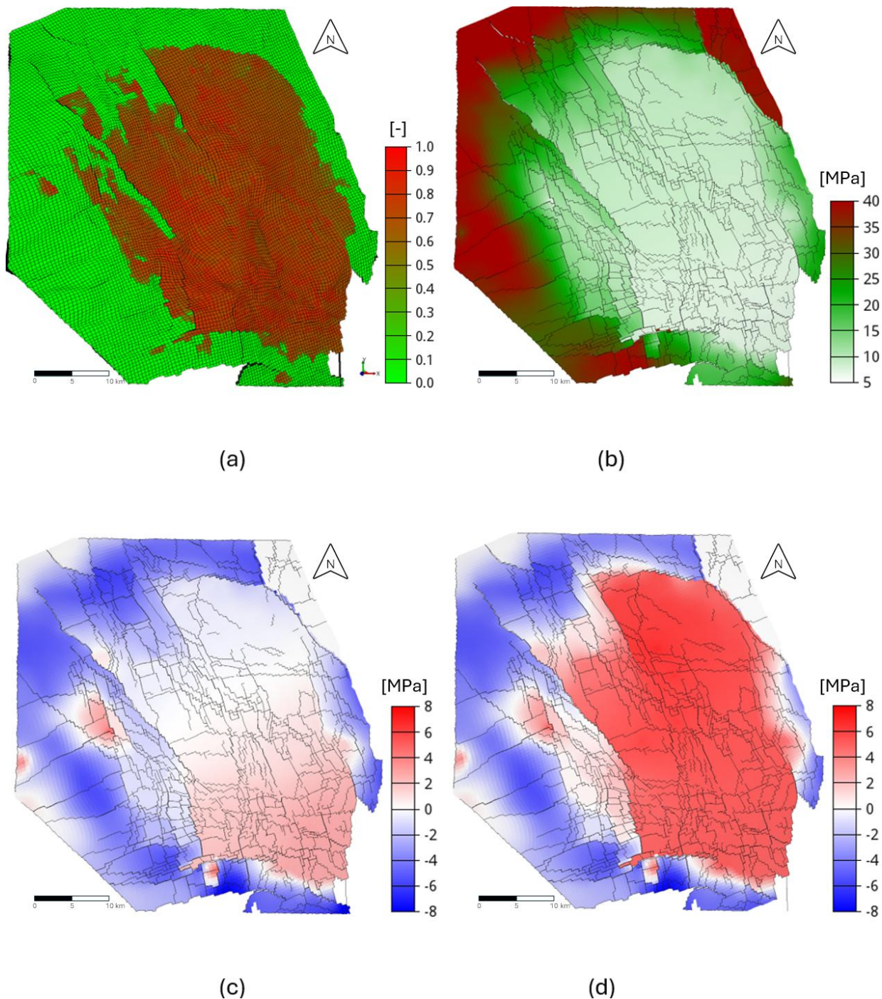
Figure 3 (a) Top view of the initial gas saturation [-] on the simulation grid. (b) Pressure [MPa] at the end of production (October 2023). (c) Change in pressure [MPa] over the injection period for the LO_10ZBSE scenario. (d) Change in pressure [MPa] over the injection period for the LO_SE_1ZB-10ZB scenario.
