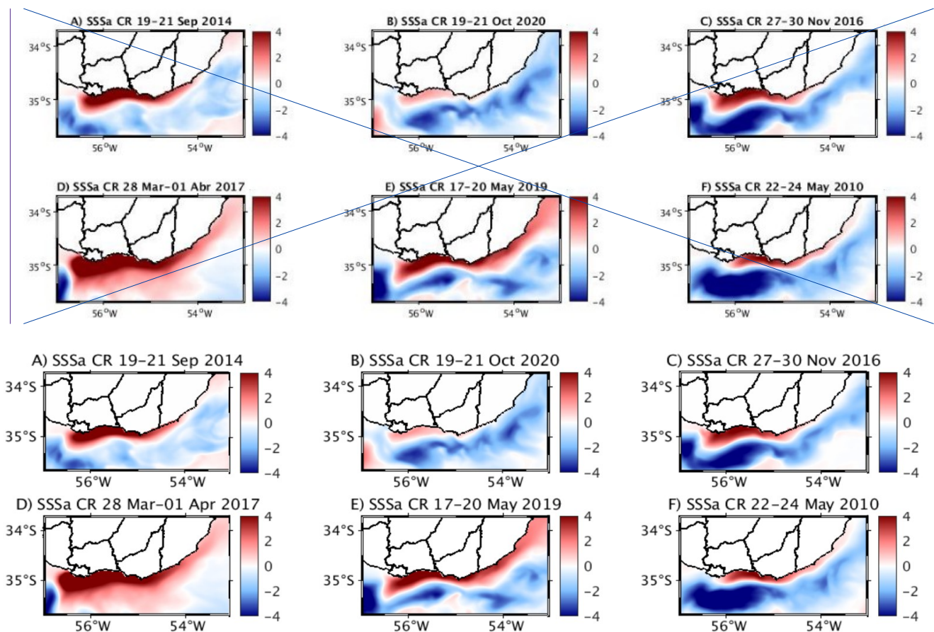
Figure 8: Average simulated Sea Surface Salinity anomalies (SSSa) distribution during selected upwelling events
