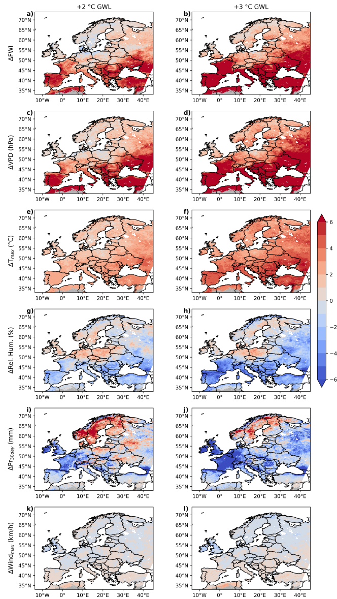
Figure 11. Spatial patterns of the composites based on the ensemble median of 33 bias-adjusted EURO-CORDEX models, shown as changes relative to the reference period (1971-2000) at +2 °C (left panels) and +3 °C GWL (right panels). Composites are created by averaging delta changes of a, b ) FWI, c, d ) VPD (hPa), e, f ) daily maximum temperature (°C), g, h ) daily mean relative humidity (%), i, j ) 30-day antecedent accumulated precipitation (mm), k, l ) daily maximum wind speed (km/h) on days when FWI exceeds its 99 th percentile.
