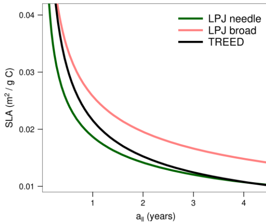
Figure 2: Generalized relationship between leaf longevity ( a_{||} ) and specific leaf area (SLA). For a given size of the leaf carbon pool, short leaf longevities and high SLA result in a high light interception potential (e.g., total leaf area and leaf area index) but are associated with higher annual carbon investments to rebuild the carbon pool due to the short longevity. The generalized relationship employed in the model represents an intermediate form between the leaf longevity to SLA relationships considered for specific plant functional types with fixed a_{||} in the LPJ vegetation model (Schaphoff et al., 2018; Sitch et al., 2003).
