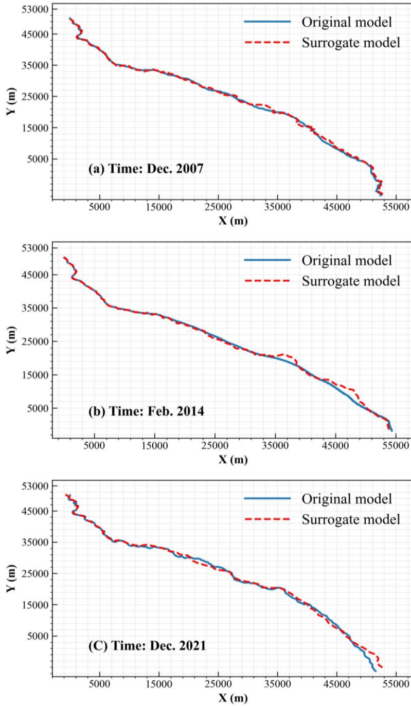
Figure 10. Comparison between the original river channel migration model and the surrogate model at different time points.
