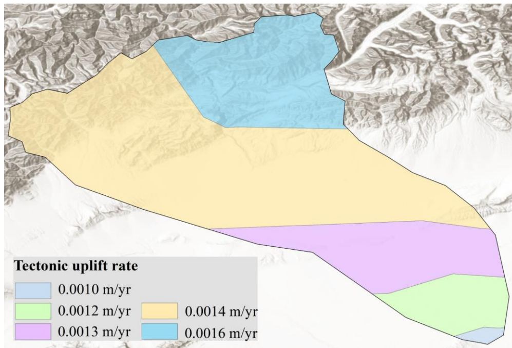
Figure 6. Zonation of average tectonic uplift rates in the study area from 2000 to 2021. Basemap: Esri World Hillshade (Esri).
