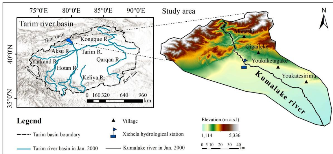
Figure 4. Schematic diagram of the watershed in the study area. Basemap: Esri World Hillshade (Esri).
