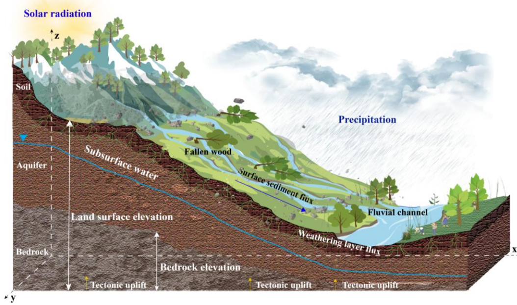
Figure 2. Schematic diagram of the Landscape evolution process.
