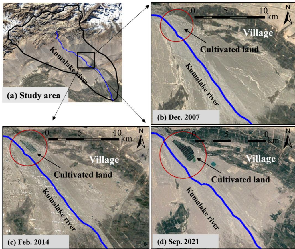
Figure 13. Formation process of cultivated land along the river in the study area. Satellite imagery: © Google Earth 2007, 2014, 2021, modified by the authors.
