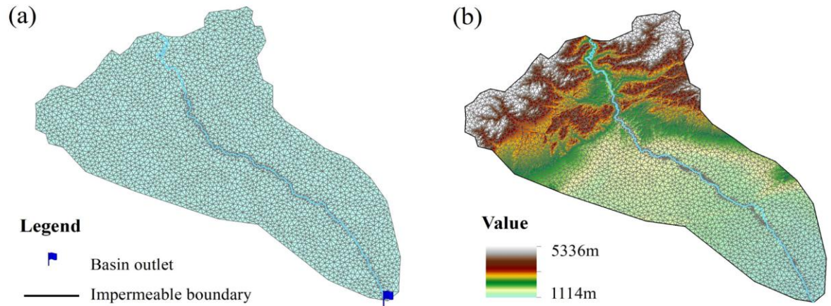
Figure 8. Mesh discretization and initial elevation grid of the research area.
