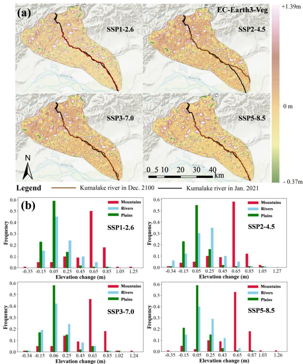
Figure 15. Spatial distribution of river channel (a) and Elevation change (b) under four future climate scenarios based on the EC-Earth3-Veg climate model. Basemap: Esri World Hillshade (Esri).
