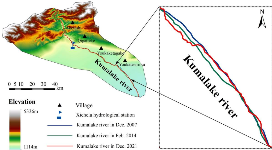
Figure 7. The spatial distribution of the Kumalake River channels in the study area.
