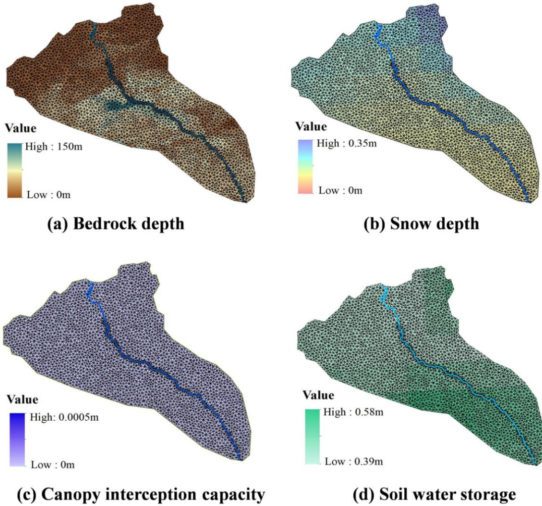
Figure 9. The initial conditions of landscape evolution model.
