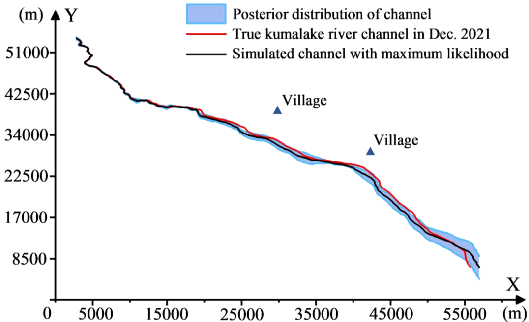
Figure 12. The predicted Kumalake River channel at December 2021.
