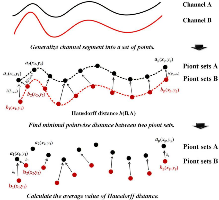
Figure 3. Conceptual schematic diagram of Hausdorff distance.
