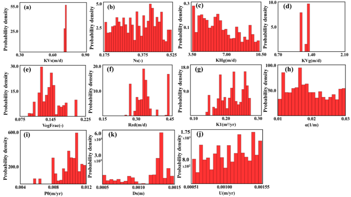
Figure 11. Calibrated posterior distributions of model parameters.
