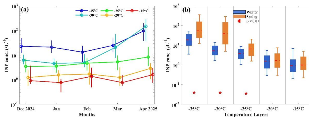
220 Fig. 2. Monthly variations and Seasonal differences in INPs. (a) Monthly median INP concentrations. (b) Seasonal box plots of INP concentrations in winter (December–February) and spring (March–April); boxes indicate the interquartile range, whiskers the 10th–90th percentiles, and red asterisks denote significant differences.
