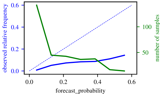
lead = 30-212 days
