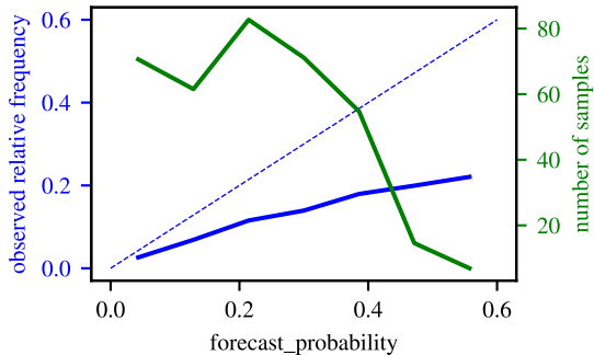
lead = 30-212 days
