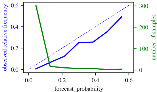
lead = 0-30 days
