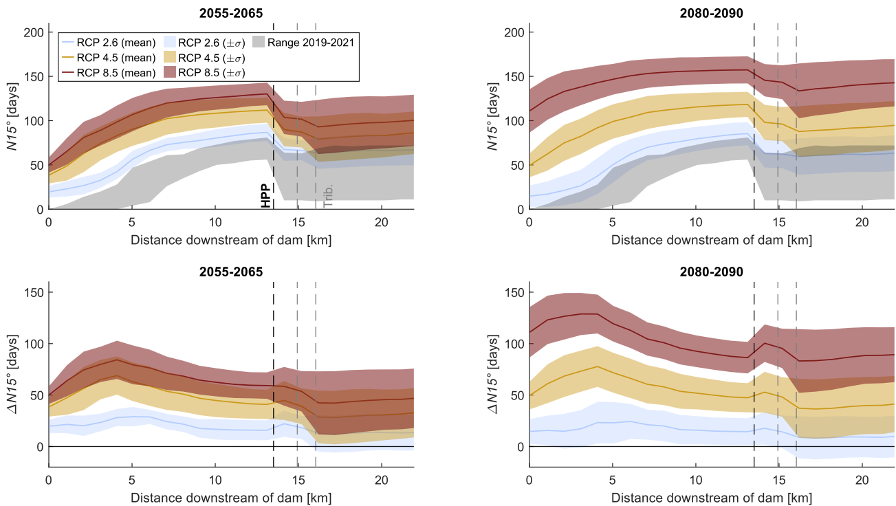
Figure B2 14: Simulated number of days with an average stream temperature above 15°C ( N15^\circ , top) for current and future climate along the reach, and difference between current and future climate ( \Delta N15^\circ , bottom)
