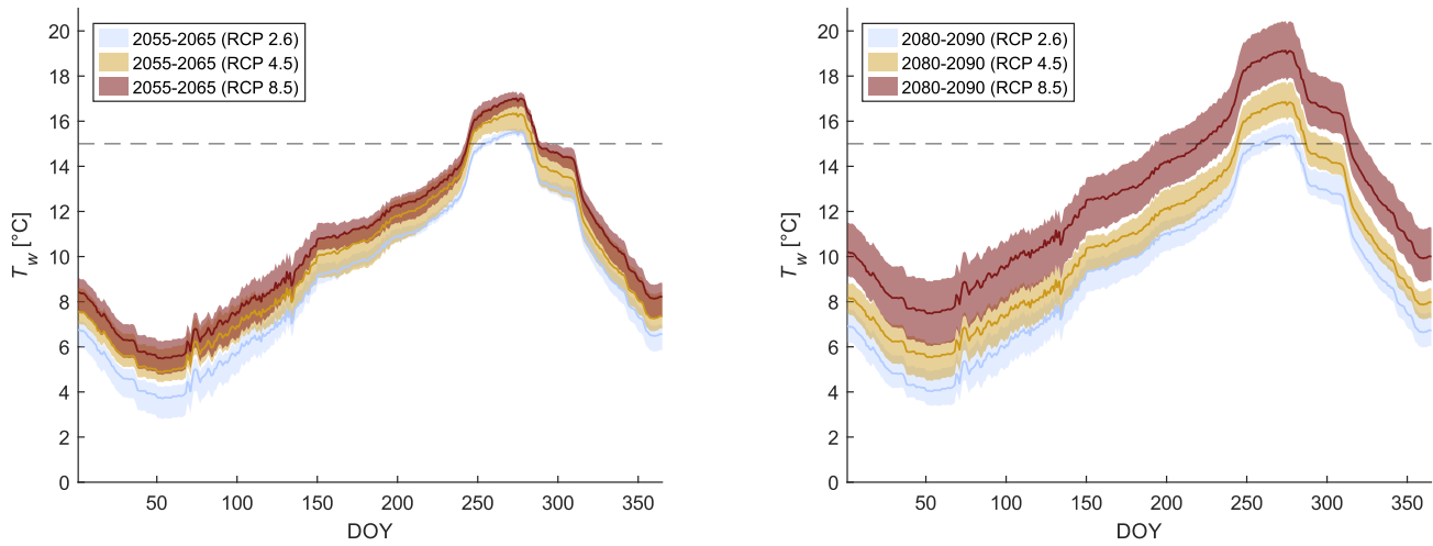
Figure B3 : Simulated lake temperature at residual for intake level (637.5 m asl) under climate change for 2055-2065 (left) and 2080-2090 (right), dotted line indicates 15°C showing that lake temperature will tend to be above this threshold more often in the future
