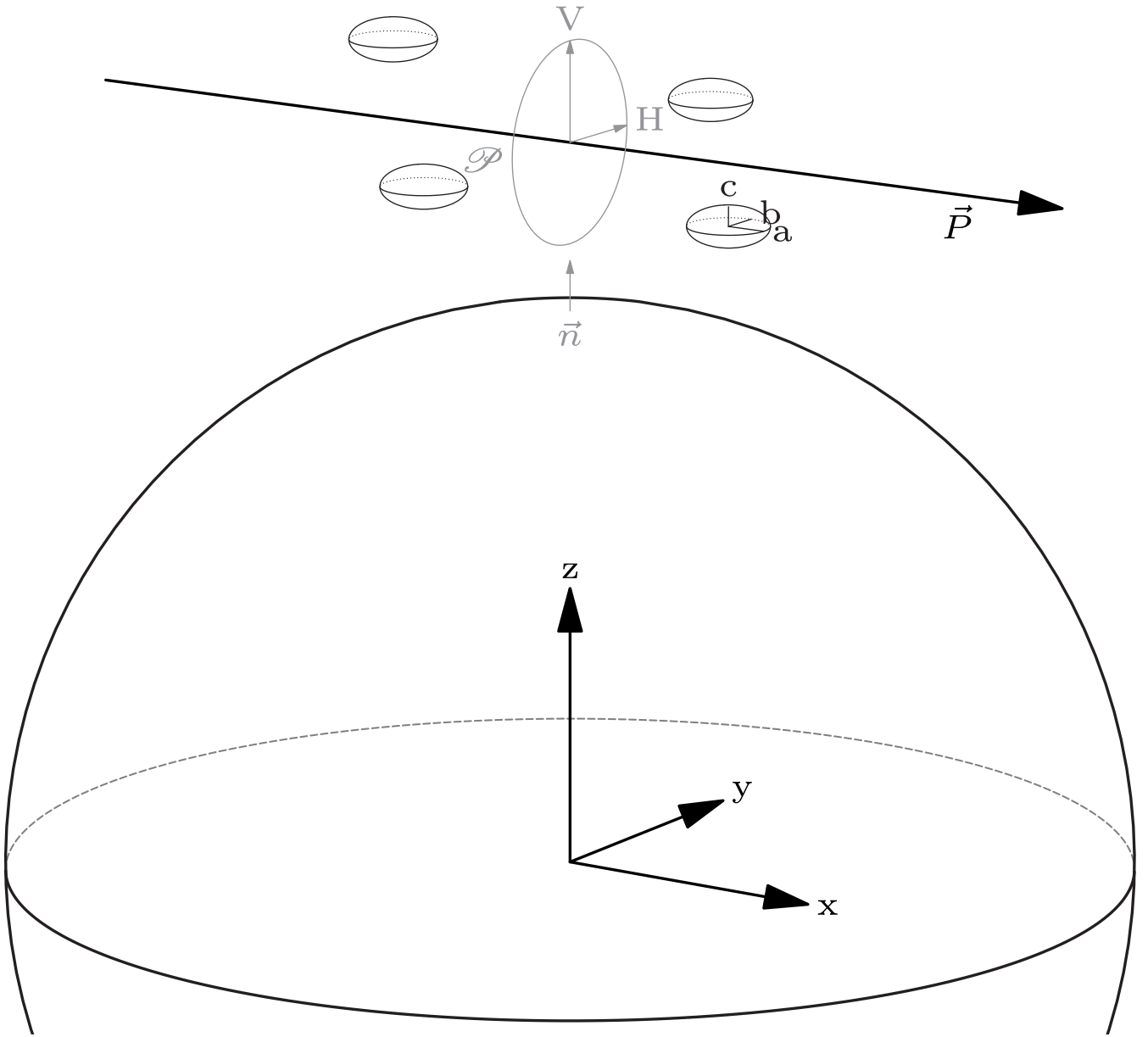
Figure 1. Scheme for a signal propagating along P , through the Earth's atmosphere. The signal finds flattened drops, of axes a = b > c in its path. The electric field oscillates within the polarization plane \mathcal{P} . Due to the symmetry of the drops, there is always in \mathcal{P} a direction H that lies inside the symmetry plane (a,b). Oscillations along this direction H meet the drops along their major axis. Oscillations in the perpendicular direction V meet the drops at some other angle, that depends on the elevation angle of the ray and the canting angle of the drops. In the case depicted, a horizontal ray and zero canting, V is oriented along the minor axis of the drops.
