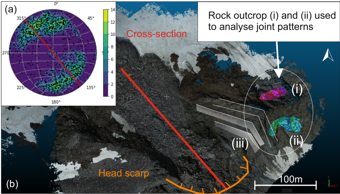
Figure A1. Structural analysis of two rock outcrops in proximity to the rock-slide's detachment area . In total, 11339 planes were reconstructed and analyzed using the FACET plugin in Cloud Compare software (Dewez et al., 2016). Parameters for FACET plugin: Fusion algorithm Kd-tree , max-anlge 20, max relative distance 1.00. (a) Stereographic projection of the geological planes using CLAR-method for illustration and 'Kamb exponential smoothing': Units are in numbers of standard deviations by which the density estimate differs from uniform (produced with mplstereonet Kington, 2024)). The two identified clusters are joint planes. (b) Orthophotographic view of the ridge exhibiting the detachment area of the rock slideslope failure , including the location of the two rock outcrops and the whitish highlighted structural features of morphology (iii) that intersect the ridge: Steep dipping, perpendicular oriented foliation planes. The UAV point cloud model recorded in August 2024 was used as the basis for analysis in Cloud Compare (2 cm model resolution).
