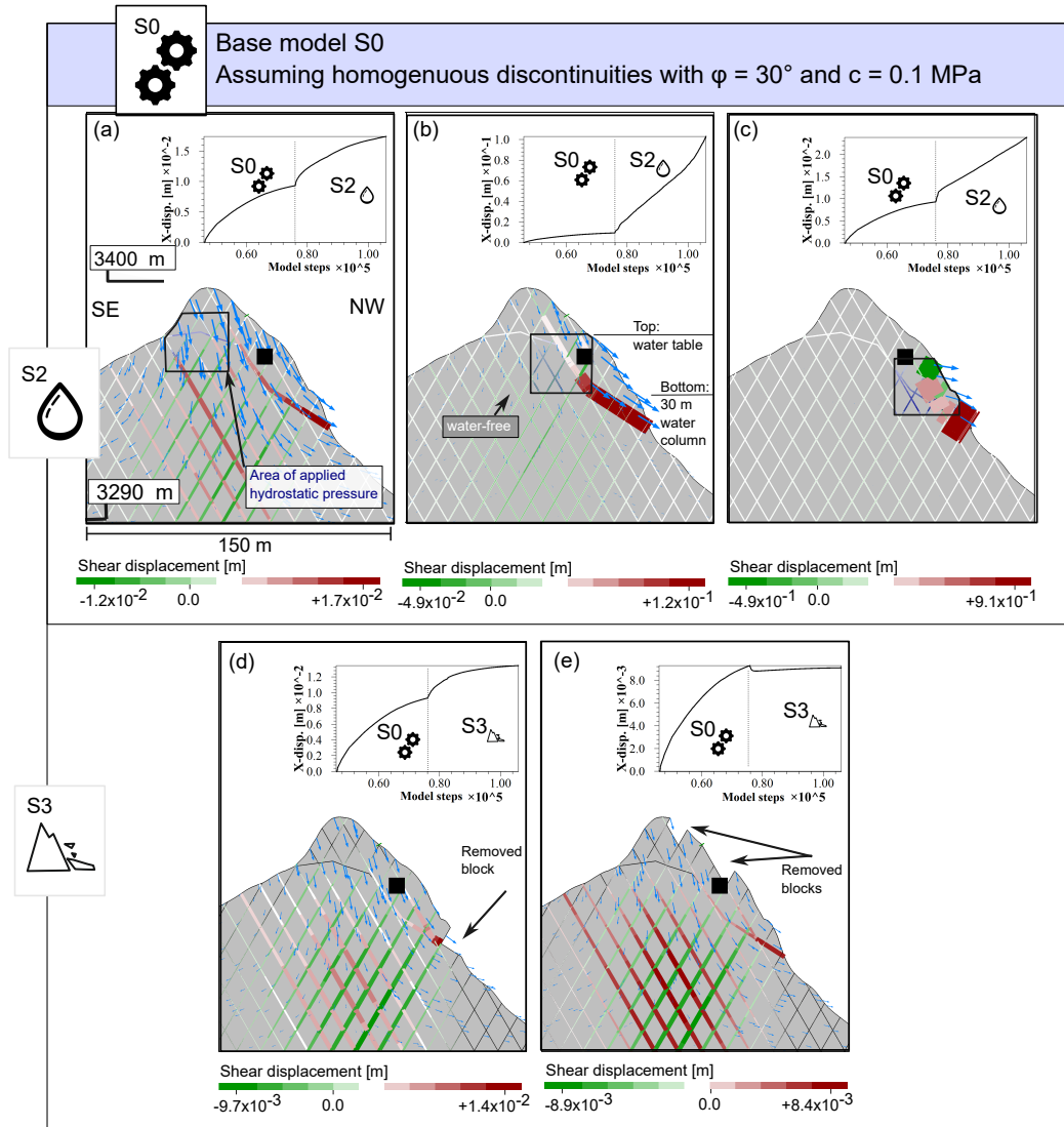
Figure 11. The impact of hydrostatic pressure and rockfalls on rock slope stability calculated with UDEC for model setup A -(a-e) using the model of back-calculated pre-failure state from scenario S0 ( \phi = 30^\circ and c = 0.1 MPa; see Fig. 10c) or (f-j) the temperature-dependent shear criterion S1 (Fig. 10b) as base a basis. (a-c/f-h) Impact of hydrostatic water pressure on slope mechanics, illustrated for three different locations of assumed water pressure. (d,e/f-j) Impact of rockfalls (removal of individual blocks) on slope mechanics. Explanation of charts as shown in Figure 9. Note that the state of the model is displayed for the end of the simulation, and the illustrated shear displacement shows the cumulative displacement of S0 /S1 and S2 or S3, respectively.
