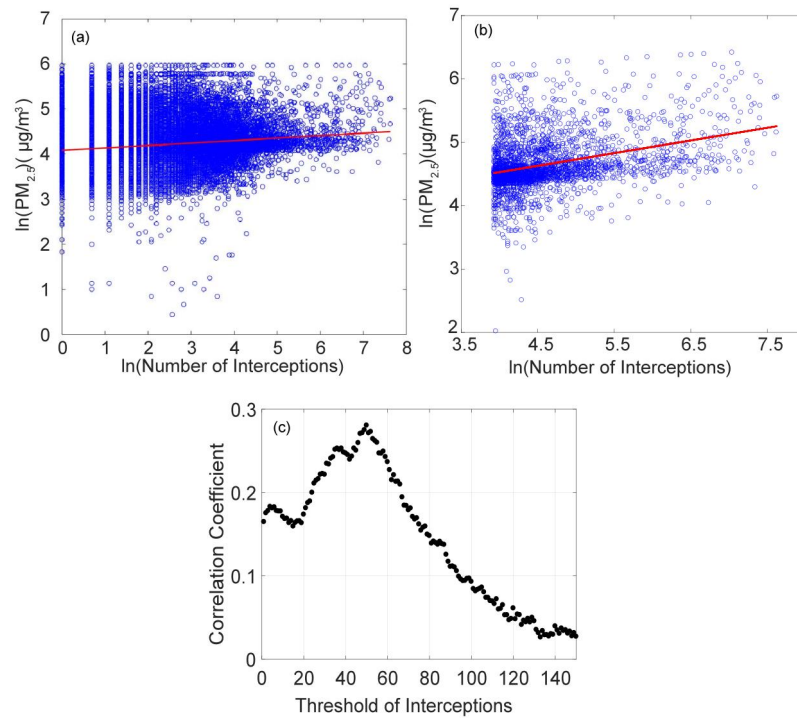
Figure 5. (a) and (b) scatter distributions of \text{PM}_{2.5} concentrations against the number of fire hotspots when interception threshold is set to be 1 and 50, respectively. (c) correlation coefficient between \text{PM}_{2.5} and the number of fire hotspots as a function of the interception threshold.
