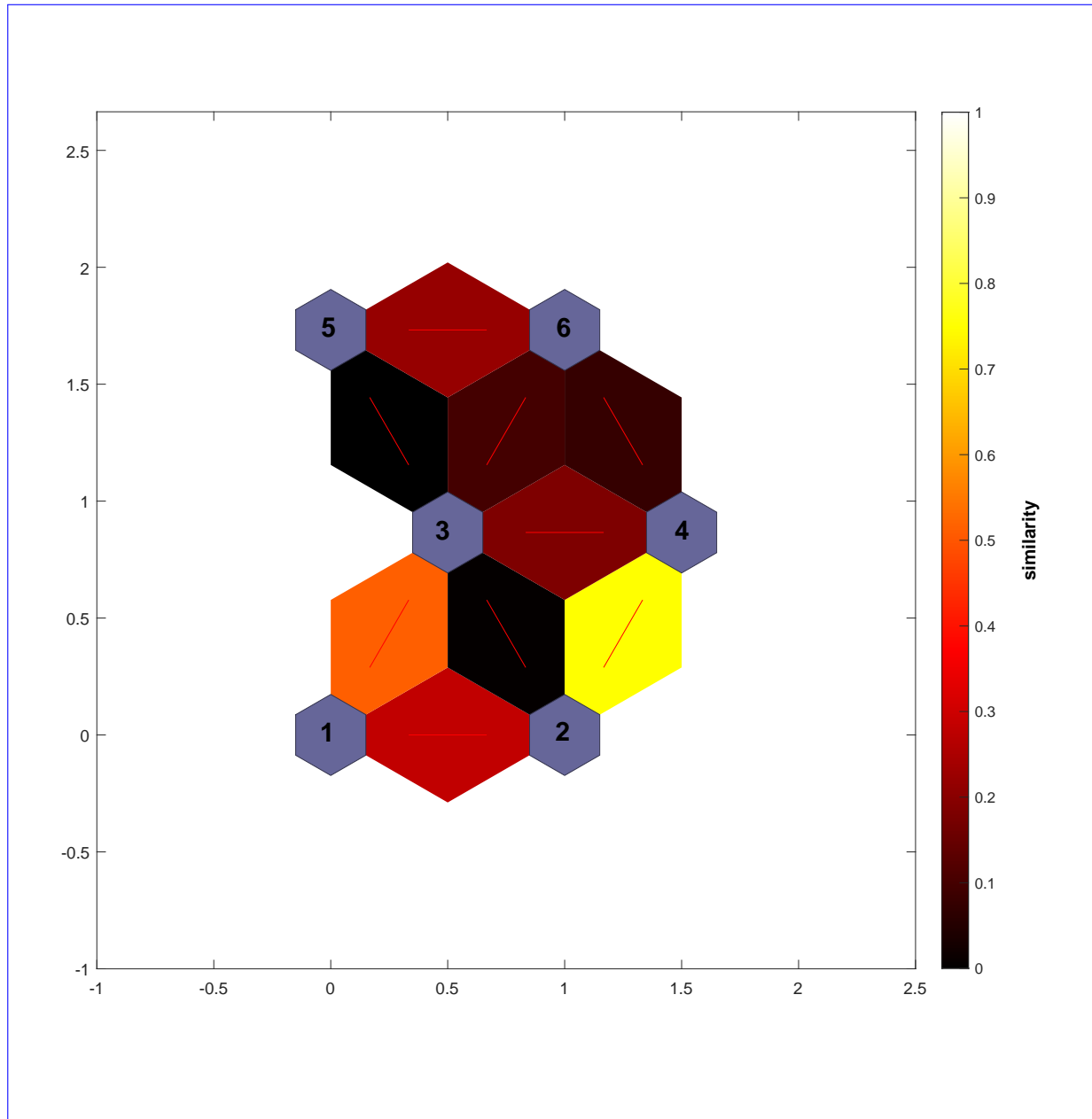
Figure A1. SOM configuration with neighbour similarity, illustrating the differences between neighbouring clusters. Cluster numbers are noted in the purple nodes; note their different order compared to other figures in the paper.
