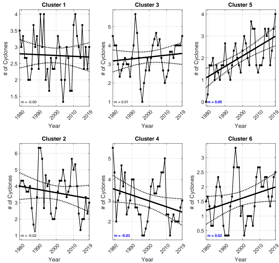
Figure 9. As in fig. 1a, but shown separately for each cluster. The slope of each linear trend is annotated as m (cyclones-EMCs per year). Trends significant at the 90% confidence level (Mann-Kendall test, \alpha = 0.1 ) are indicated by blue coloured m .
