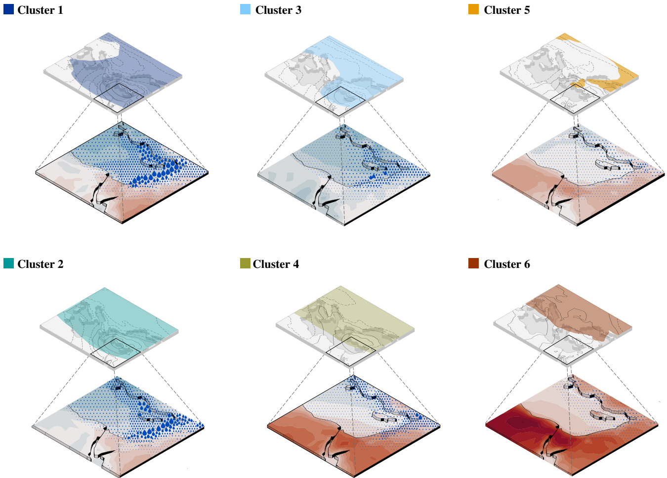
Figure 10. Schematic summary of the EMC clusters. For each cluster, the upper panels show the large classification domain with the 3-PVU surface ( shading ) and SLP ( black contours at 2-hPa intervals, dashed over 1015 hPa ). The lower panels present a zoomed view over the Eastern Mediterranean, displaying temperature anomalies and accumulated precipitation.
