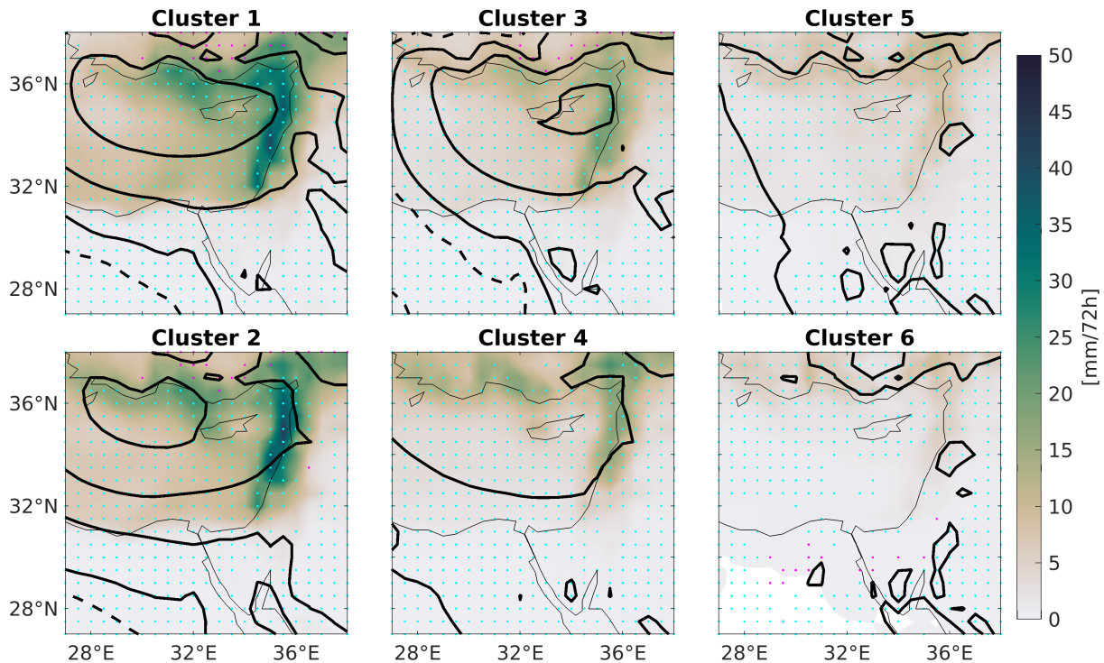
Figure 5. Composite mean 3-day ERA5 accumulated precipitation (shaded (white is 0) , mm/72h), beginning at 6 am of the day of minimum cyclone SLP, by cluster. Cyan-dotted areas indicate regions where ERA5 convective-scale precipitation exceeds 60% and magenta-dotted areas where ERA5 large-scale precipitation exceeds 60%. SLP is shown with black contours at 2-hPa intervals, with dashed contours for values above 1015 hPa. Note the smaller domain compared to Figure 2, covering only the cyclone-detection region.
