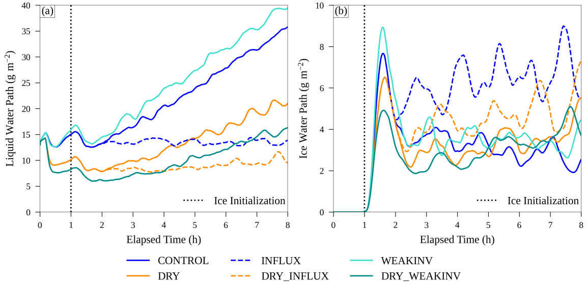
Figure 2. Time series of LWP (a) and IWP (b) in six simulations. The initiation of ice formation at t = 1 hour is indicated by the vertical dotted line.
