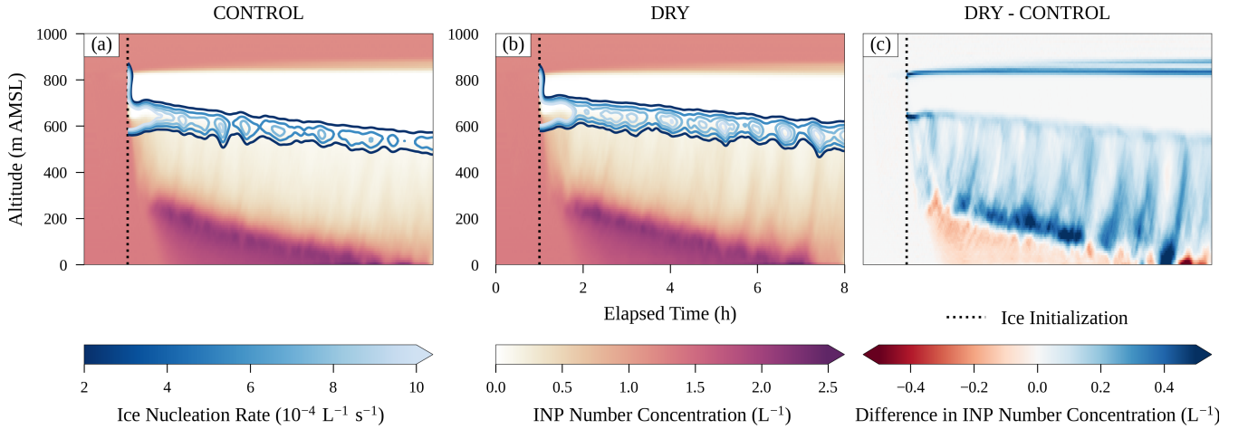
Figure 14. A time-height comparison of INP number concentration and nucleation rate. (a,b) show INP number concentration in pink-purple shading and ice nucleation rate in blue contours. The contour range is from 2 \times 10^{-4} \text{ particle L}^{-1} to 1 \times 10^{-3} \text{ particle L}^{-1} with a contour interval of 2 \times 10^{-4} \text{ particle L}^{-1} . Contours are smoothed in time with a gaussian kernel with a 2.5 minute standard deviation for clarity. (c) shows the difference in INP number concentration between DRY and CONTROL in red and blue shading.
