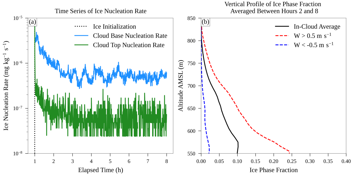
Figure 8. (a) A time series of heterogeneous ice nucleation rate at cloud base (blue) and cloud top (dark-bluegreen) in the CONTROL simulation. Ice initiation at t = 1 hour is denoted by the black vertical dotted line. (b) A time-average vertical profile of ice phase fraction in updrafts (red, dashed), downdrafts (blue, dashed), and over the entire cloud (black, solid) between hours 2 and 8 in CONTROL.
