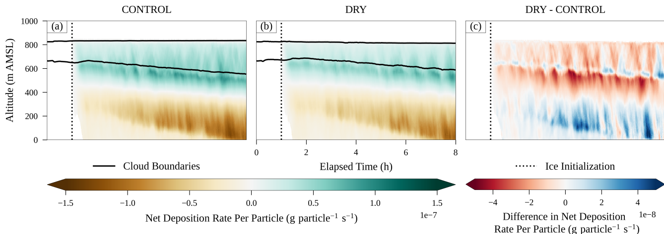
Figure 11. A time-height comparison of net deposition rate per particle. Deposition rates per particle are shown in green and brown shading in (a,b), while differences between CONTROL and DRY and CONTROL are shown in blue and red shading in (c). Cloud contours for respective simulations are indicated by solid black lines in (a,b), while the initiation of ice processes at t = 1 hour is shown by the vertical dotted black lines.
