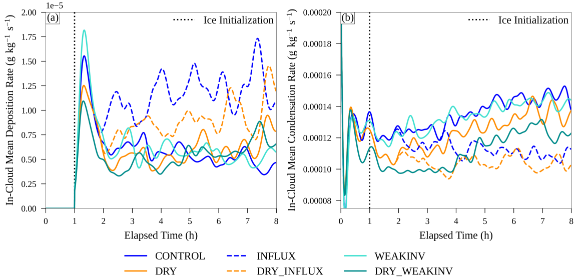
Figure 13. Time series of average in-cloud deposition rate (a) and condensation rate (b). Note that this is not the deposition rate per particle, but rather per mass of air. Ice initiation at t = 1 hour is indicated by the vertical dotted black lines. Quantities are smoothed with a Gaussian time filter with a standard deviation of 5 minutes for clarity.
