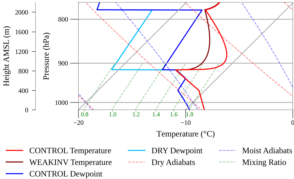
Figure 1. Initial thermodynamic conditions of the CONTROL simulation. Temperature Initial temperatures of the CONTROL and dewpoint WEAKINV simulations are indicated by the red and blue-maroon solid lines, respectively. Initial dewpoints of CONTROL and DRY are indicated in blue and light blue solid lines, while dry respectively. Dry and moist adiabats are indicated by the red and blue dashed lines, respectively. Isopleths Isolines of constant water vapor mixing ratio are depicted from 0.8 to 1.6 g kg -1 , at intervals of 0.2 g kg -1 , in the green dashed lines.
