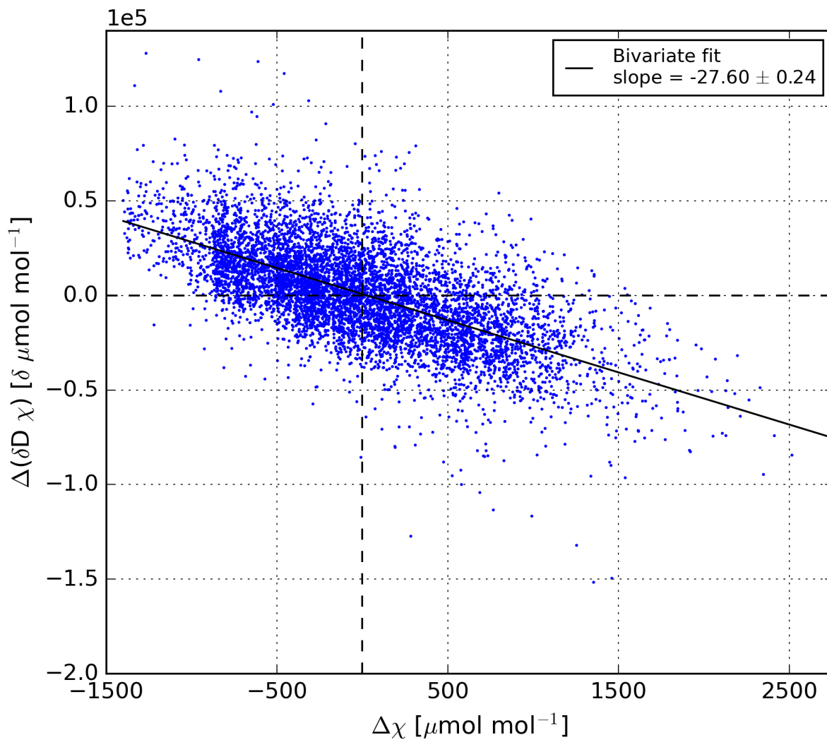
Figure A1. Example Miller-Tans analysis of the 30 min interval starting at 15:00 on 15-08-2022. The variations in \delta values and H 2 O mole fractions ( \chi ) were measured using the H 2 O isotope analyser measuring from the inlet at 57 m. The \Delta refers to the difference between the measured value and the atmospheric background (Miller and Tans, 2003).
