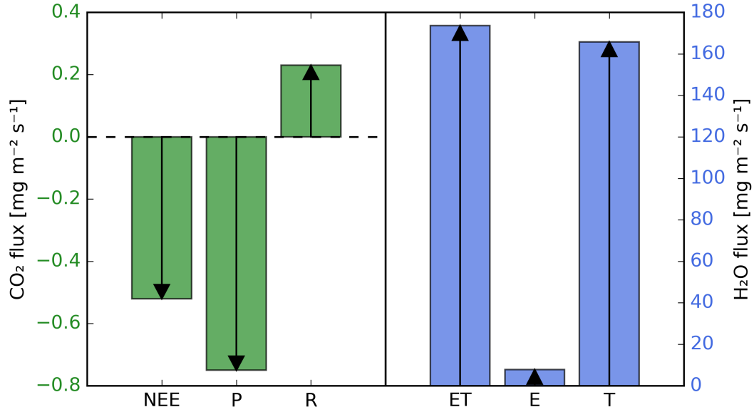
Figure 7. Results of the partitioning of the net ecosystem exchange fluxes NEE and ET based on the 13 day composite 14:00 isotopic state, following Eq 2. For NEE , the ^{18}O -CO 2 isotope was used following the approach described in Sec. 2.2. For ET , the average of the partitioning results derived from \delta D and \delta^{18}O is shown (see Sec. 2.1).
