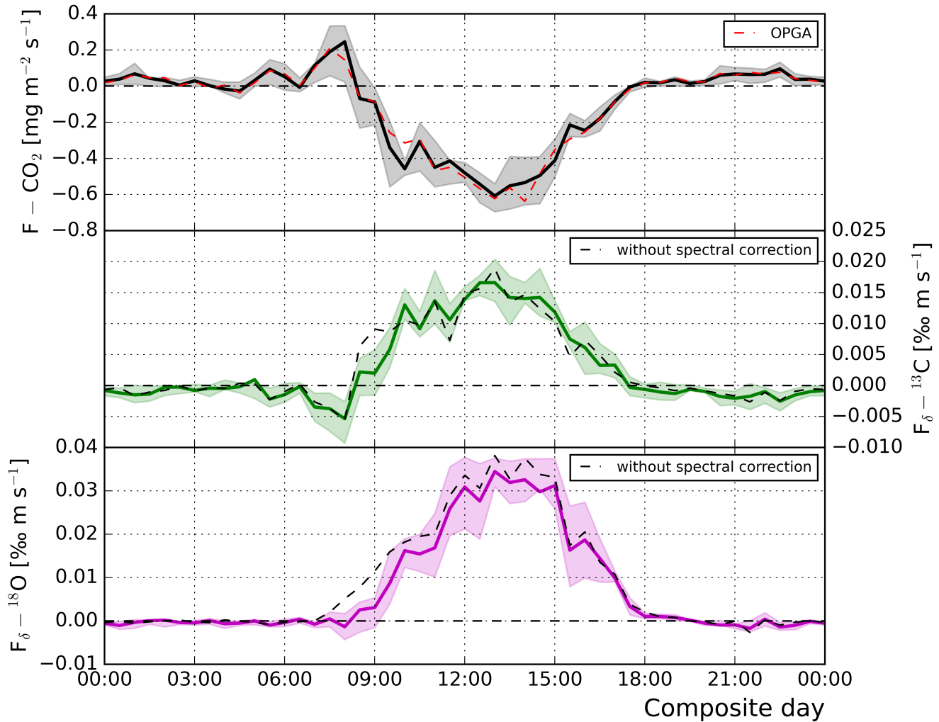
Figure 4. top) Composite day 30 min average \text{CO}_2 fluxes derived using the closed path isotope analyser and an Open Path Gas Analyser (OPGA, shown in red). middle) and bottom) Composite day 30 min average {}^{13}\text{C} and {}^{18}\text{O} \delta fluxes derived using the \text{CO}_2 isotope analyser combined with the EC method. The dashed black lines show the data before correction of signal loss at high frequencies. The shaded areas indicate the 25 to 75 % quantiles of the 13 days contributing to the composite day.
