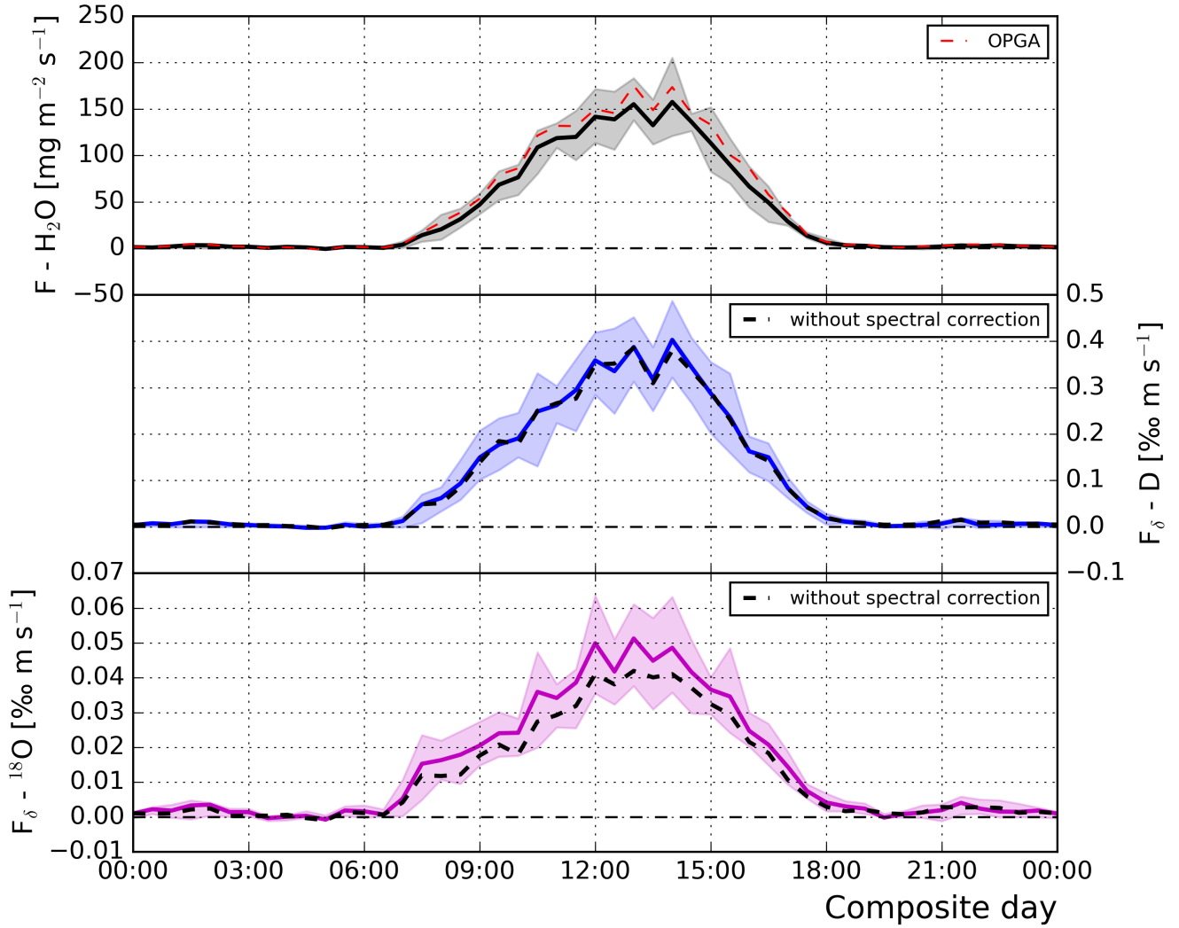
Figure 2. top) Composite day 30 min average water flux derived using the closed path isotope analyser and an Open Path Gas Analyser (OPGA, shown in red). middle) and bottom) Composite day 30 min average D and ^{18}\text{O} \delta fluxes derived using the water isotope analyser combined with the EC method. The dashed black lines show the data before correction of signal loss at high frequencies. The shaded areas indicate the 25 to 75 % quantiles of the 13 days contributing to the composite day.
