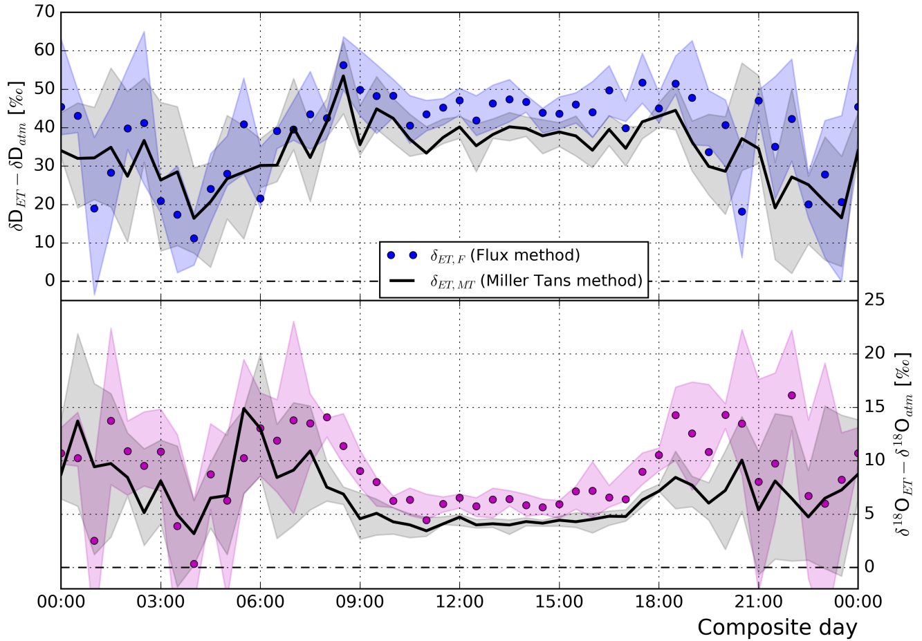
Figure 3. Composite day representation of 30 min average isotopic compositions of the net flux ( \delta_{ET} ) derived using measurements performed with the water isotope analyser. The flux method composition ( \delta_{ET,F} ) was derived using Eq. 4. Both the Miller-Tans and flux methods are described in Sec. 2. The shaded areas indicate the 25 to 75 % quantiles of the 13 days contributing to the composite day.
