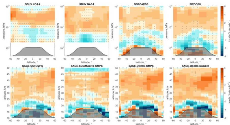
Figure 1. Ozone trends ( \% \text{ decade}^{-1} ) for the period 2000–2024 estimated from eight merged satellite data records using an independent linear trend model. Trends are shown for the SBUV COH (NOAA), SBUV MOD (NASA), SWOOSH, GOZCARDS, SAGE-CCI-OMPS, SAGE-SCIAMACHY-OMPS, SAGE-OSIRIS-OMPS, and SAGEII-OSIRIS-SAGEIII datasets. Gray stippling denotes results that are not significant at the 2\sigma level. Data are presented on the vertical coordinates (left-hand axis) and latitudinal grid associated with each dataset. The black lines show the mean climatological thermal tropopause height (or pressure) from the ERA-5 reanalysis. The trends in the upper troposphere are shaded and not assessed in this study.
