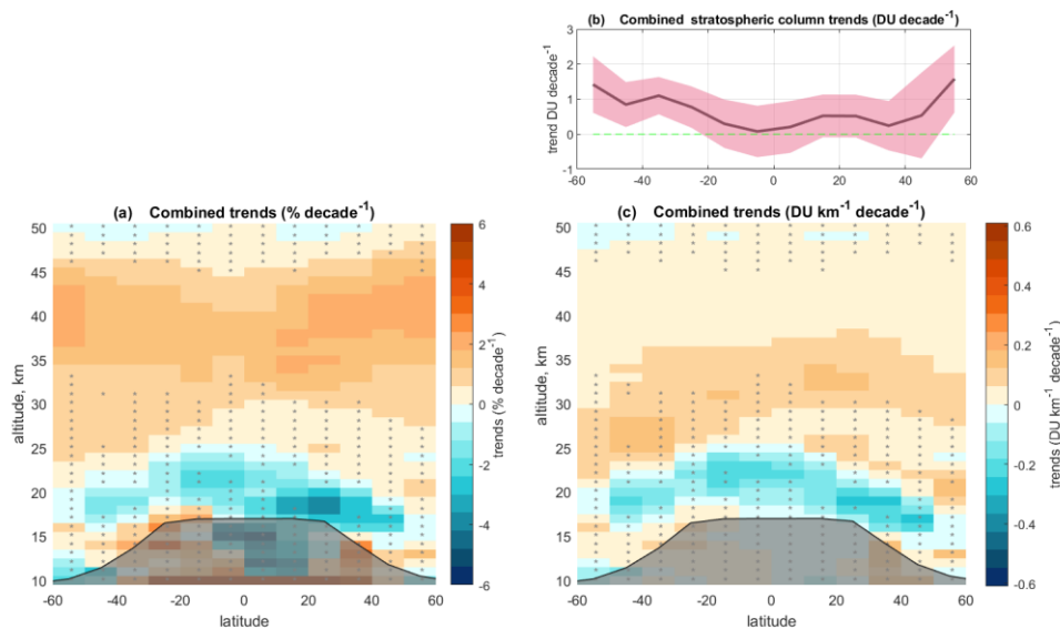
380 Figure 3. The combined (mean) ozone trends from eight merged satellite datasets as a function of latitude and altitude, expressed in % decade -1 (panel (a)) and DU km -1 decade -1 (panel(c)). The black lines show the climatological mean tropopause height. Gray stippling denotes results that are not significant at the 2 \sigma level. Panel (b): stratospheric column averaged trend (DU decade -1 ), red line, with 2 \sigma uncertainty (pink shading). The green dashed line in panel (b) highlights zero level.
