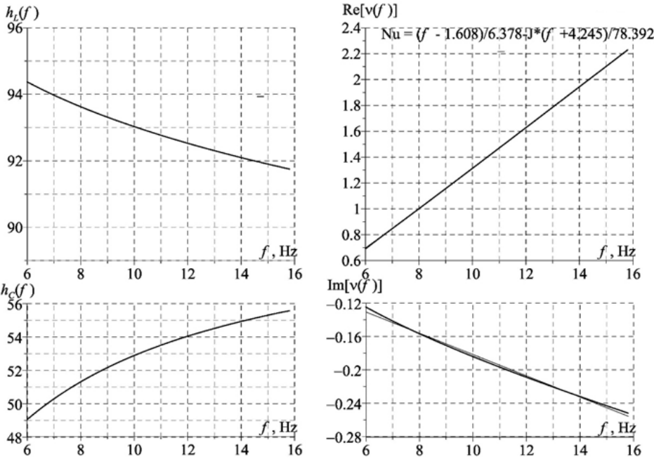
Figure A2: Real parts of the complex characteristic ionosphere heights (the graphs in the left column) and the 225 complex propagation constant of ELF radio waves as a function of frequency (graphs in the right column).
