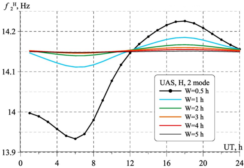
Figure A3: Impact of the source width on the range of diurnal variations in the second mode frequency in the horizontal magnetic field while measured at the Vernadsky station.
