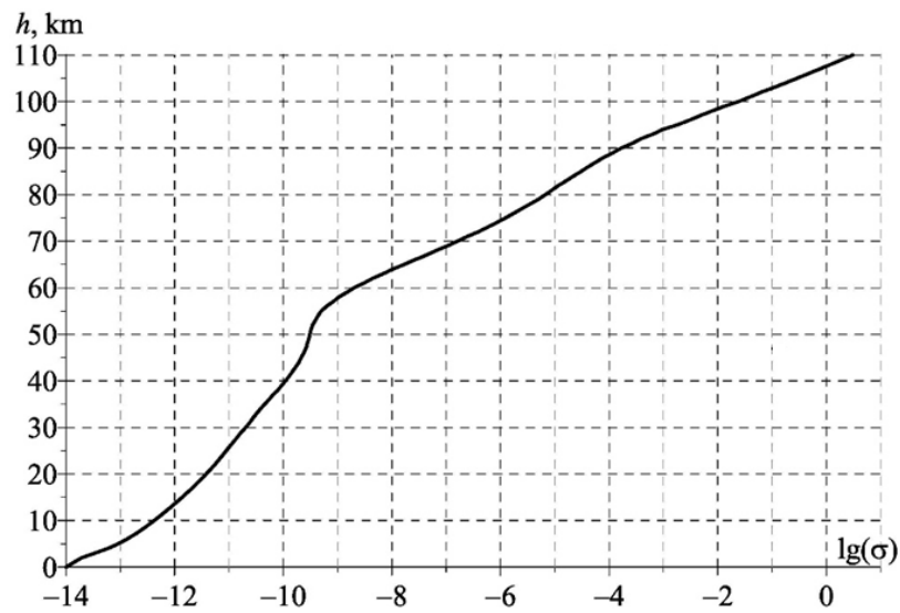
Figure A1: Vertical profile of the middle atmosphere conductivity.
