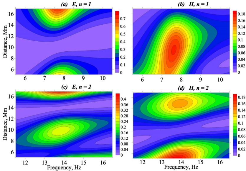
70 Figure 1: Distribution of the field intensities |E_r|^2 and |H_\phi|^2 of the first and the second SR modes over the frequency-distance plane.
