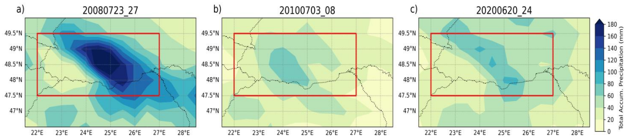
Figure S1. Accumulated precipitation from ERA5 for the three flood events in western Ukraine, from ERA5 (a) 23-27 July 2008, (b) 3-8 July 2010 and (c) 20-24 June 2020.
