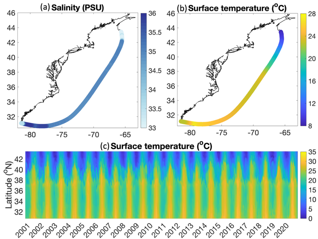
185 Figure 4: Ocean boundary forcing in the model. (a, b) Mean salinity and surface temperature along the ocean boundary over the 20-year simulation period. (c) Time series of surface temperature along the ocean boundary excluding the near near-shoal part on the southeastern side, from lower to higher latitudes.
