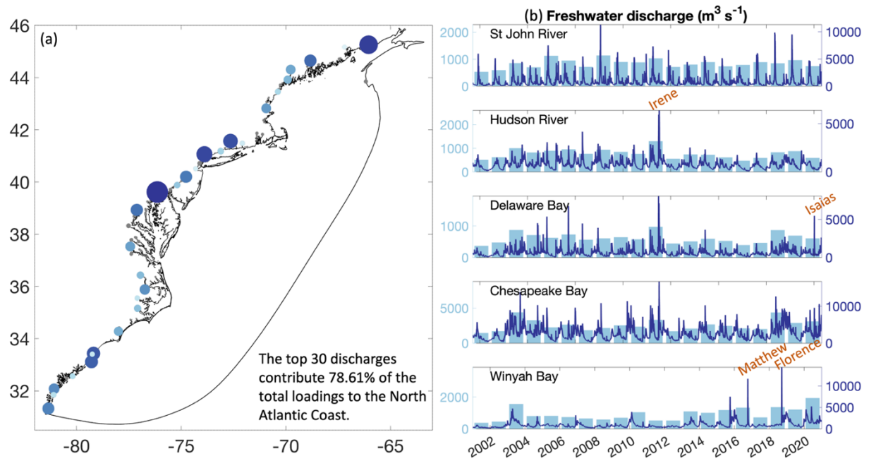
180 Figure 3: (a) Spatial distribution and (b) time series of freshwater discharge across the major water bodies of the North American Atlantic Coast. Darker colors, correlated to larger circle size, in panel (a) represent higher freshwater discharge amounts for the period from 2001 to 2020. Light blue bars in panel (b) represent the annual mean discharge for each of these estuaries.
